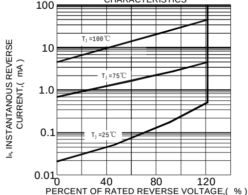
FIG.5-TYPICAL REVERSE CHARACTERISTICS
