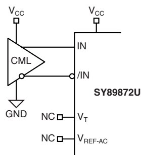
Figure 3a. DC-Coupled CML Input Interface
