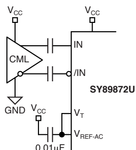
Figure 3b. AC-Coupled CML Input Interface
