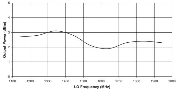
Figure 8: Typical Local Oscillator Output Power vs. Frequency ( T_A = +25\text{ }^{\circ}\text{C} , V_{DD} = +5\text{ V} )
