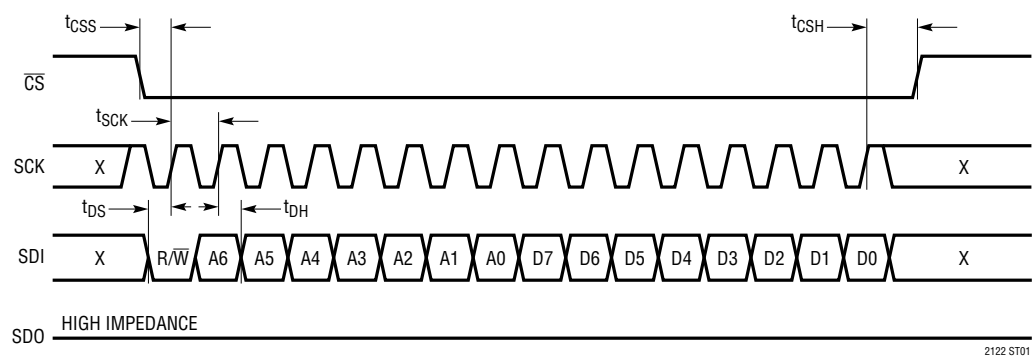
SPI Timing, Write Mode
