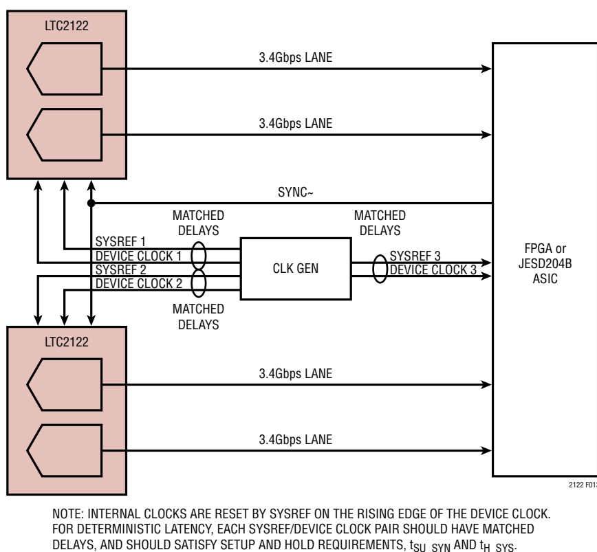
Figure 13. JESD204B Subclass 1 Configuration
