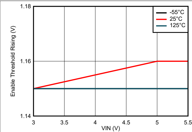
Figure 6-7. Enable Threshold Rising Variation
