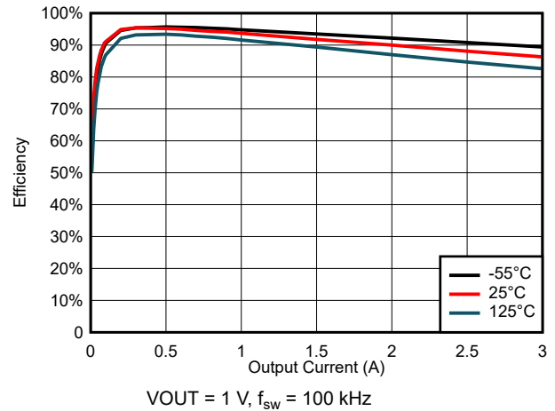
Figure 6-16. Efficiency for V_{\text{IN}} = 3 \text{ V}
