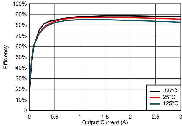
Figure 6-43. Efficiency for V_{\text{IN}} = 5 \text{ V}
