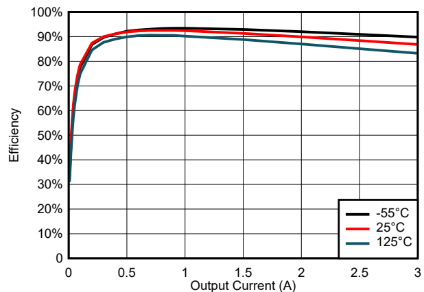
Figure 6-44. Efficiency for V_{\text{IN}} = 5 \text{ V}
