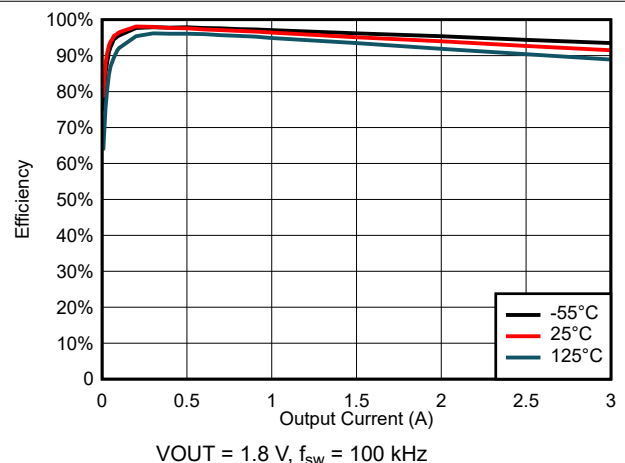
Figure 6-18. Efficiency for V_{\text{IN}} = 3 \text{ V}
