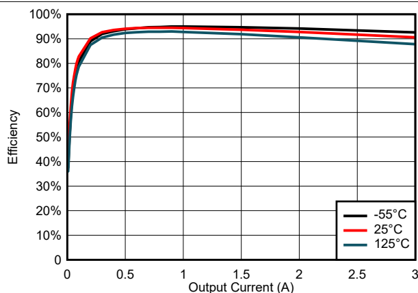
Figure 6-45. Efficiency for V_{\text{IN}} = 5 \text{ V}
