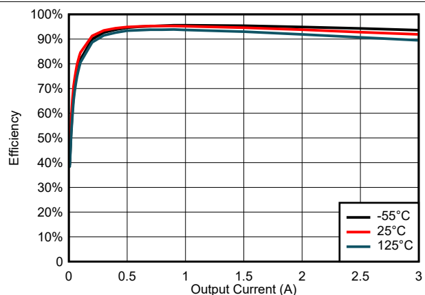
Figure 6-46. Efficiency for V_{\text{IN}} = 5.5 \text{ V}
