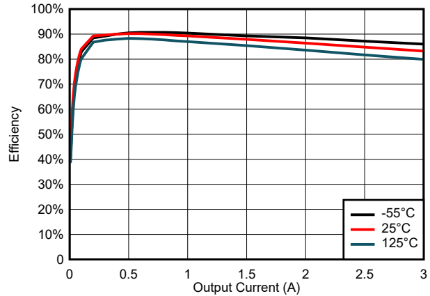
Figure 6-20. Efficiency for V_{IN} = 3 \text{ V}
