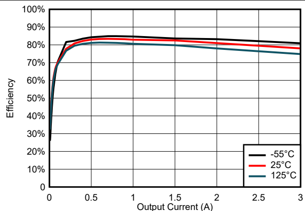
Figure 6-22. Efficiency for V_{IN} = 3 \text{ V}
