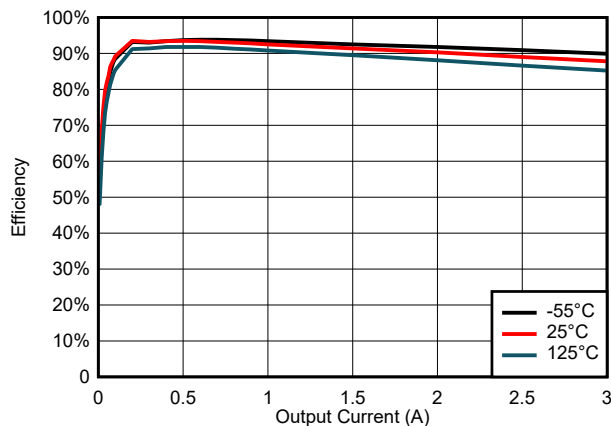
Figure 6-19. Efficiency for V_{IN} = 3 \text{ V}
