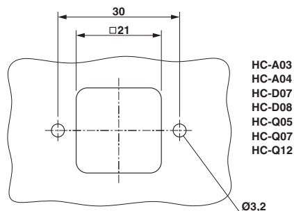
Dimensional drawing
