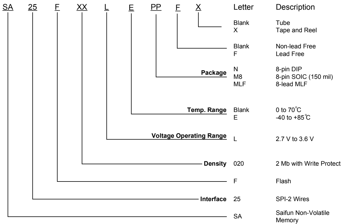
Figure 3. SA25F020 Ordering Information
