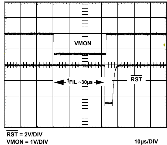
FIGURE 5. VMON LOW TO RST LOW
