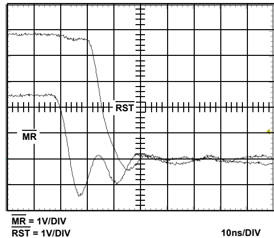
FIGURE 7. MR LOW TO RST LOW
