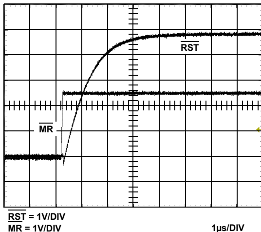
FIGURE 6. MR HIGH TO RST HIGH
