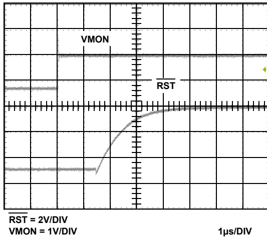
FIGURE 4. VMON HIGH TO RST HIGH
