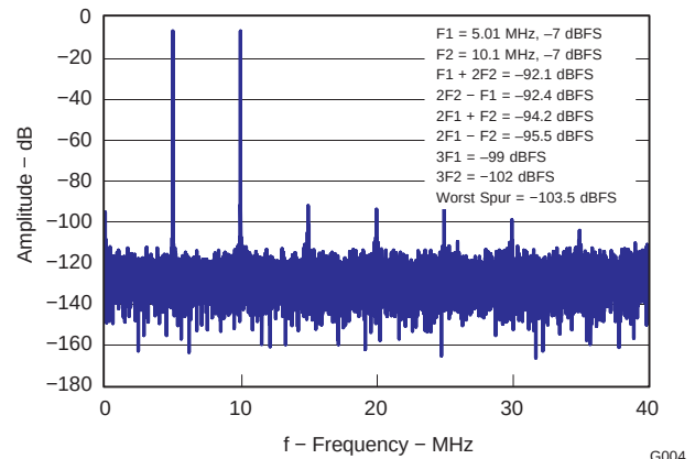
Figure 9. Intermodulation Distortion
