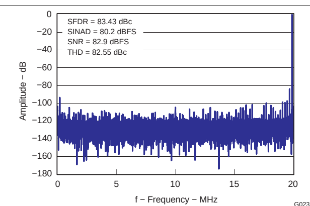
Figure 23. FFT for 20 MHz, –1-dBFS Input Signal
