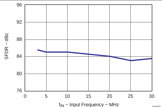
Figure 11. SFDR vs f_{IN}
