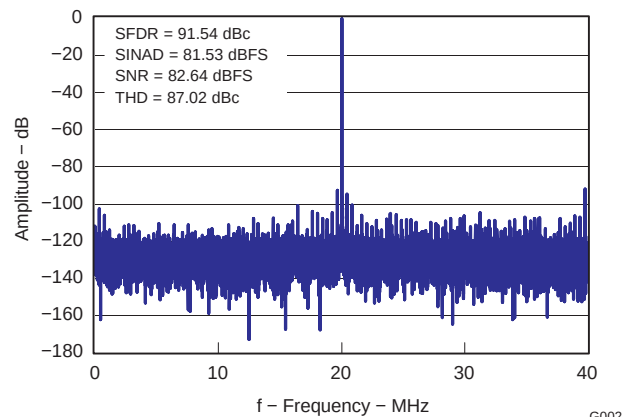
Figure 7. FFT for 20 MHz, –1-dBFS Input Signal
