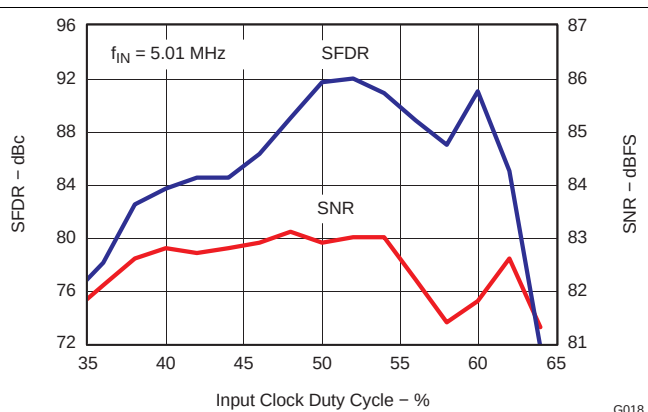
Figure 19. Performance vs Clock Duty Cycle
