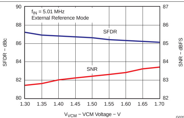
Figure 21. Performance in External Reference Mode
