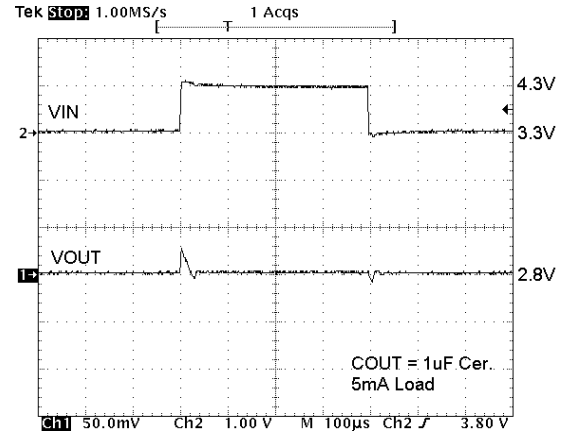
Line Transient (1Vpp) Step Response
