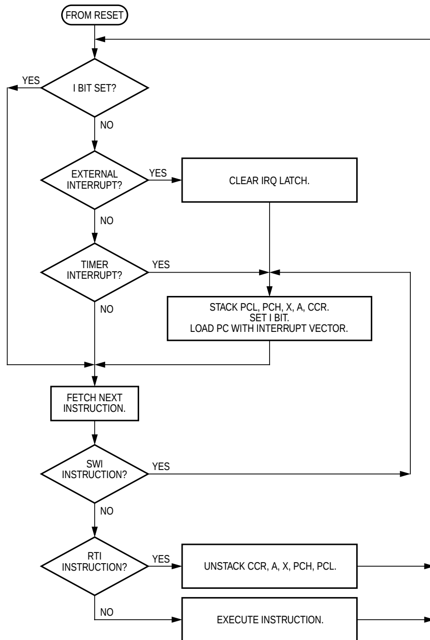
Figure 9-3. Interrupt Flowchart
