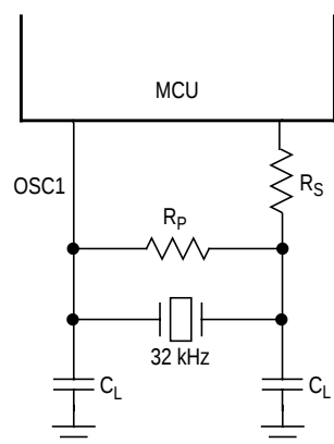
Figure B-1. Crystal Connections
