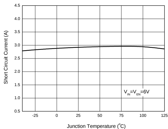
Figure 12. Short Circuit Current vs. Junction Temperature
