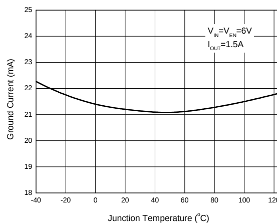
Figure 11. Ground Current vs. Junction Temperature
