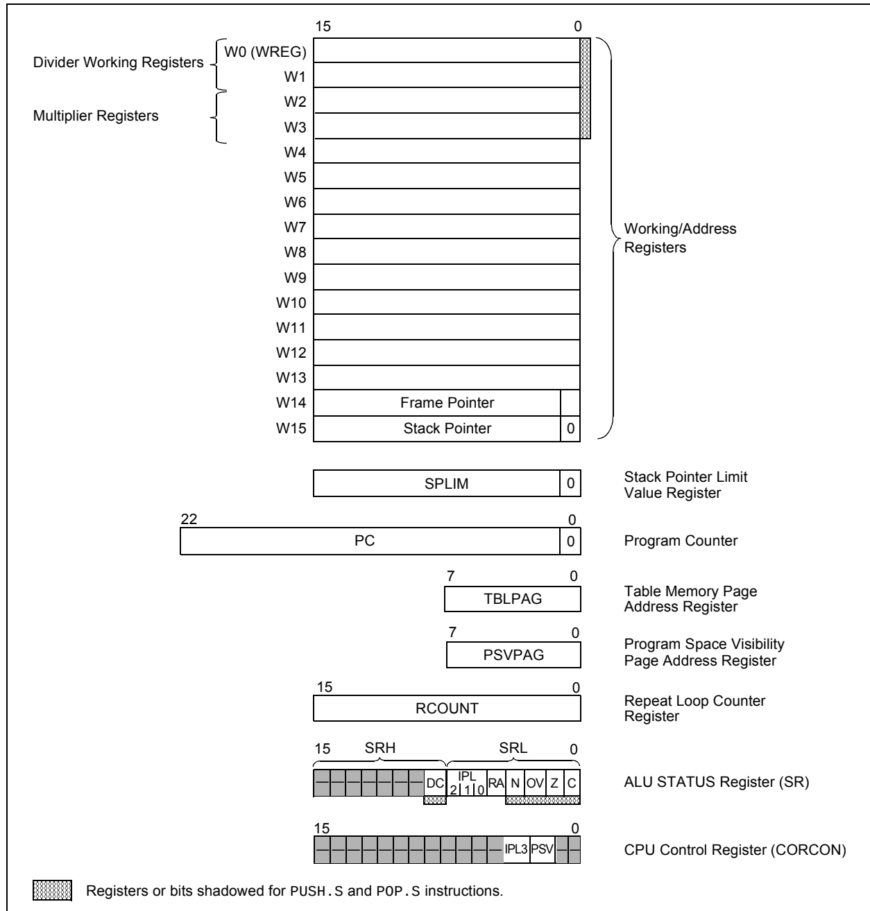
FIGURE 3-2: PROGRAMMER'S MODEL
