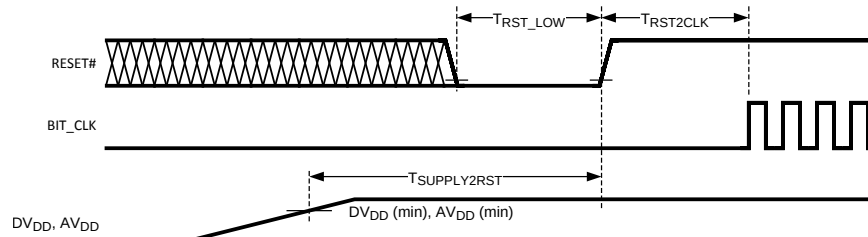
Figure 1. Power On Reset
