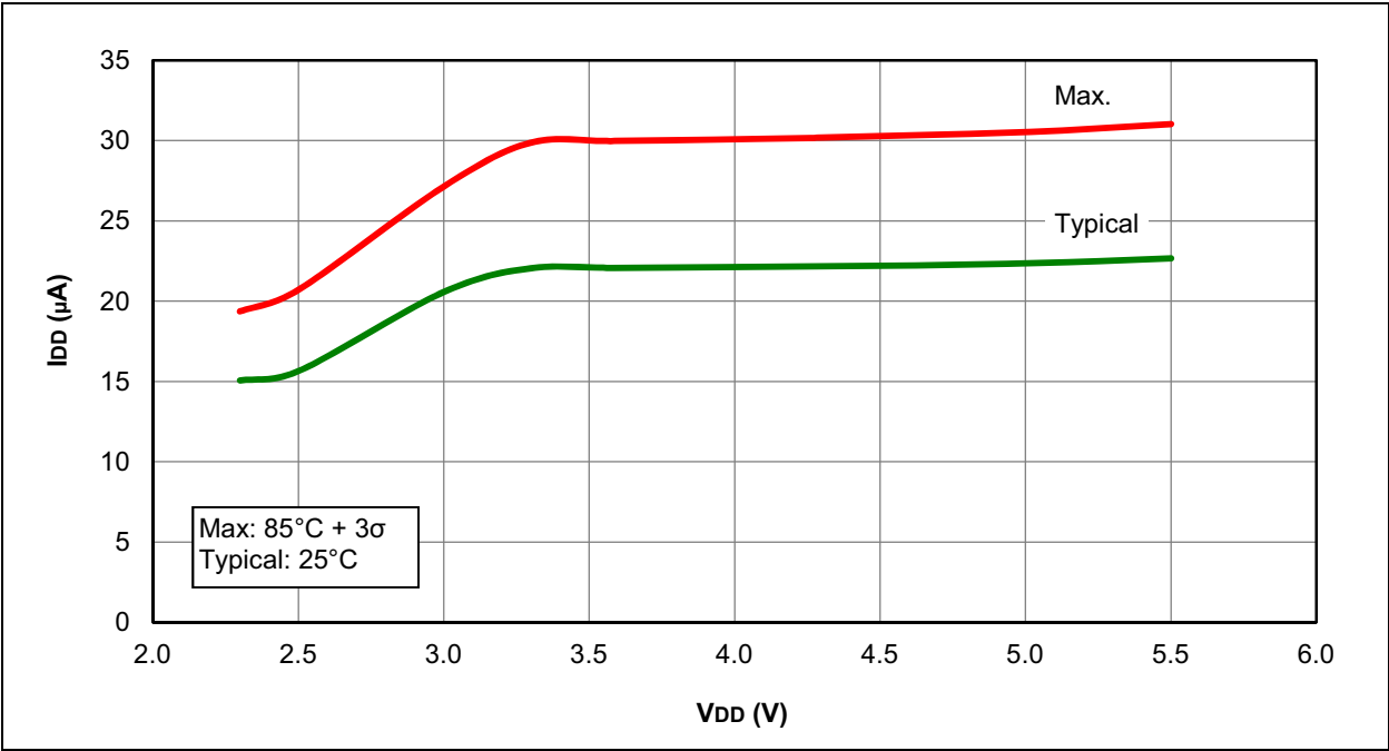
FIGURE 26-20: I DD , LFINTOSC MODE, F osc = 31 kHz, PIC16F1512/3 ONLY
