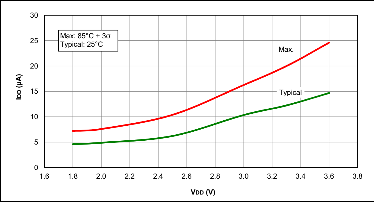
FIGURE 26-19: I DD , LFINTOSC MODE, F osc = 31 kHz, PIC16LF1512/3 ONLY
