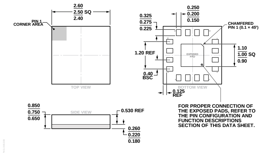
Figure 27. 16-Terminal Land Grid Array [LGA] 2.5 mm × 2.5 mm Body and 0.75 mm Package Height (CC-16-6)
