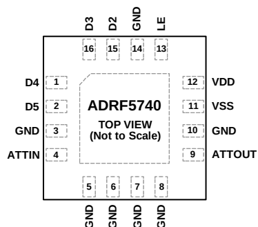
Figure 4. Pin Configuration
