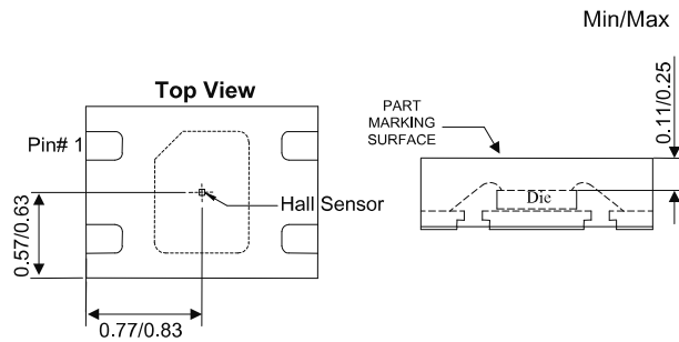
Sensor Location
