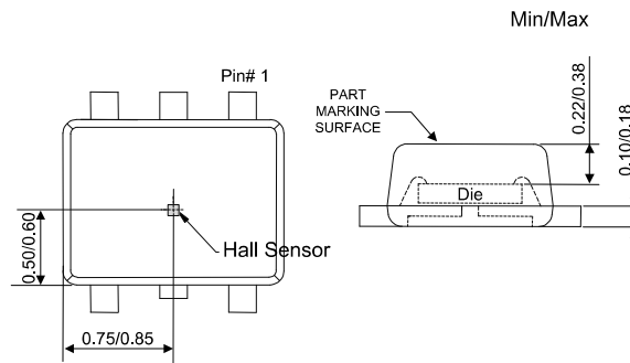
Sensor Location
