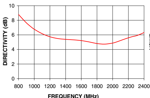
ZX60-2411BM+ DIRECTIVITY
