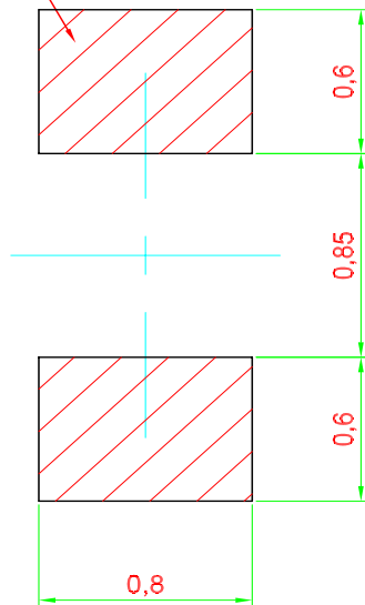
Recommended Solder-pad
