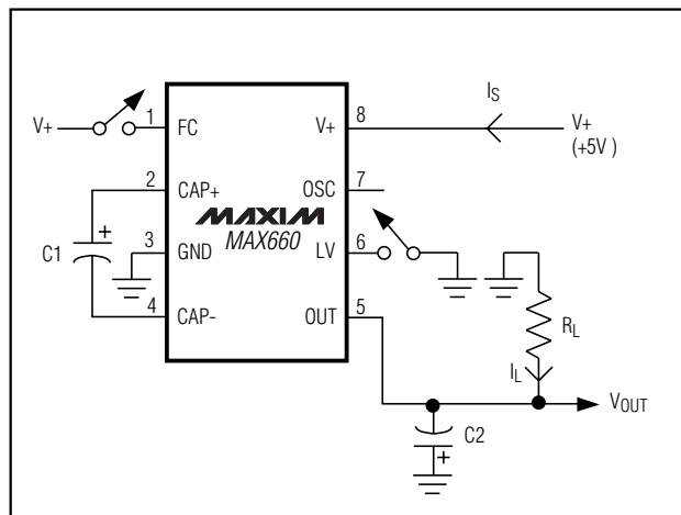
Figure 1. MAX660 Test Circuit
