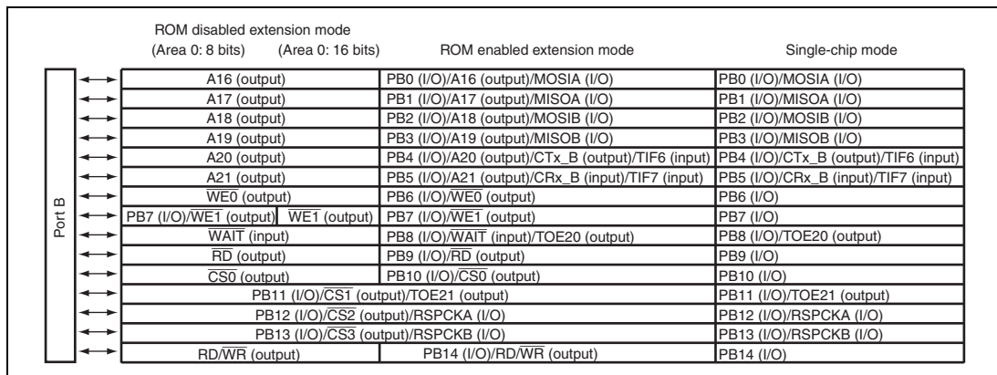
Figure 23.2 Port B
