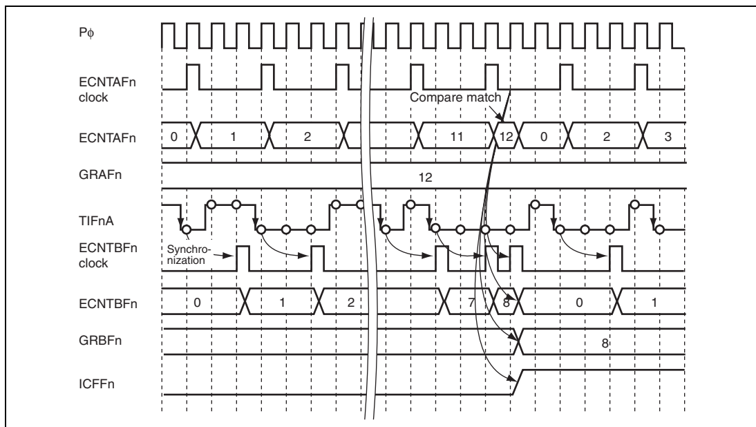
Figure 13.36 Operation Example of Edge Count in a Given Time
