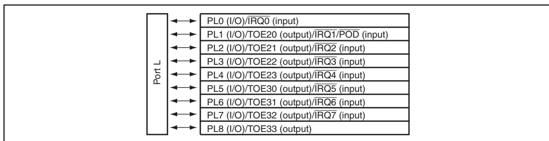
Figure 23.11 Port L
