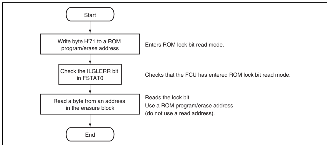
Figure 25.24 Procedure for Reading Lock Bit in Memory Area Read Mode
