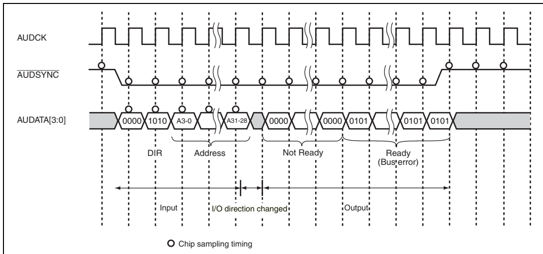
Figure 21.14 Example Operation of Error (Longword Read)
