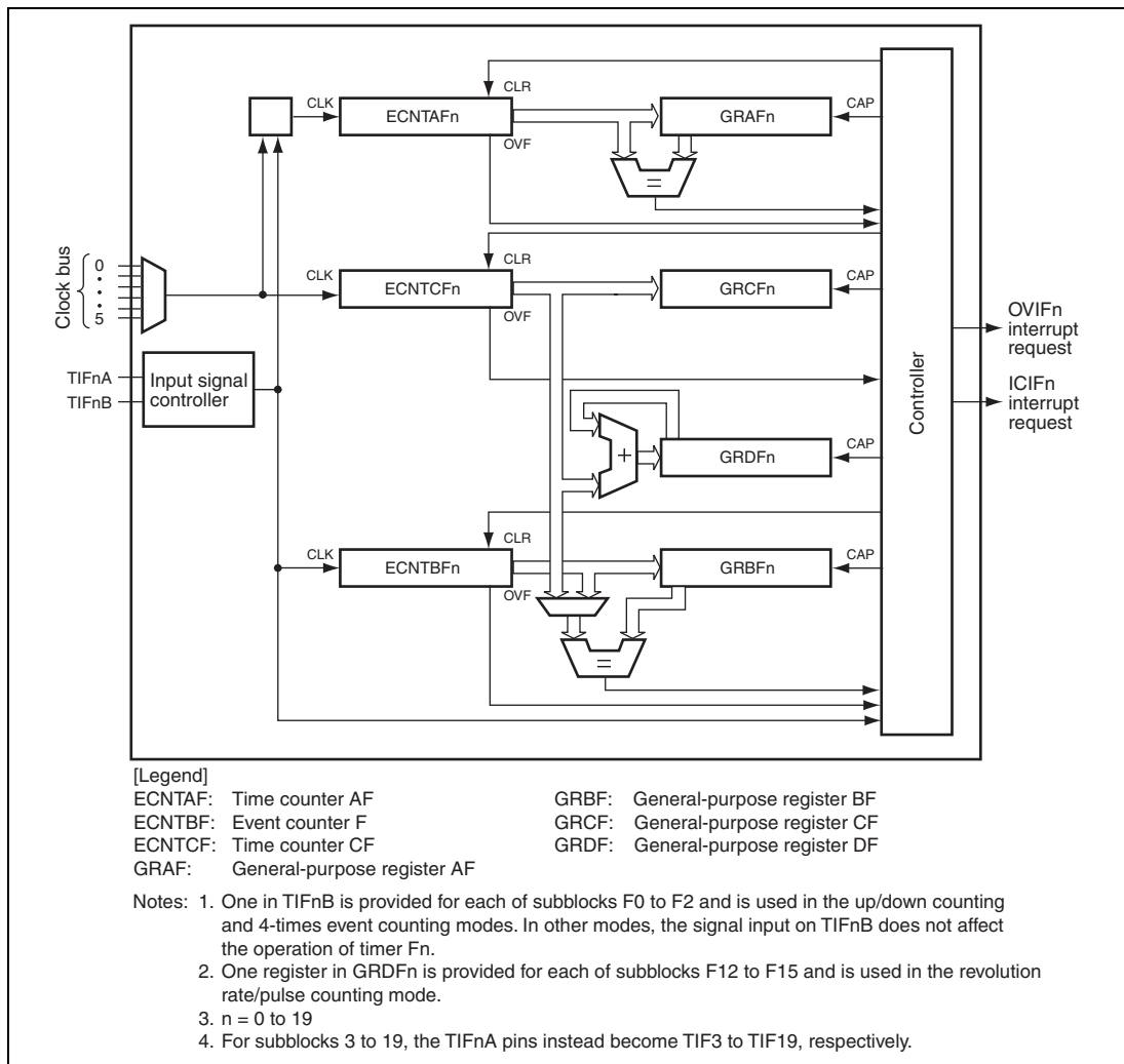
Figure 13.35 Block Diagram of Subblocks of Timer F
