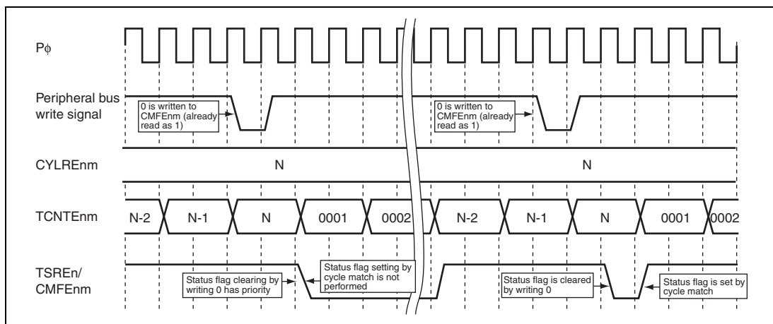
Figure 13.62 Conflict between Clearing of Cycle Match Status Flag by Writing 0 and Cycle Match
