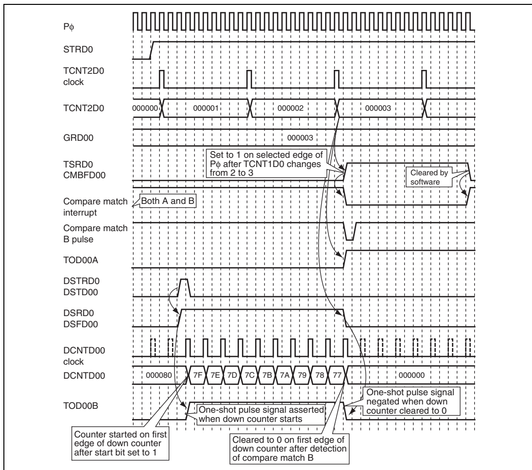
Figure 13.29 Operation Example of One-Shot Pulse Output (2) (Counting Started by Writing 1 to Counter Starting Bit and Stopped on Compare Match B)
