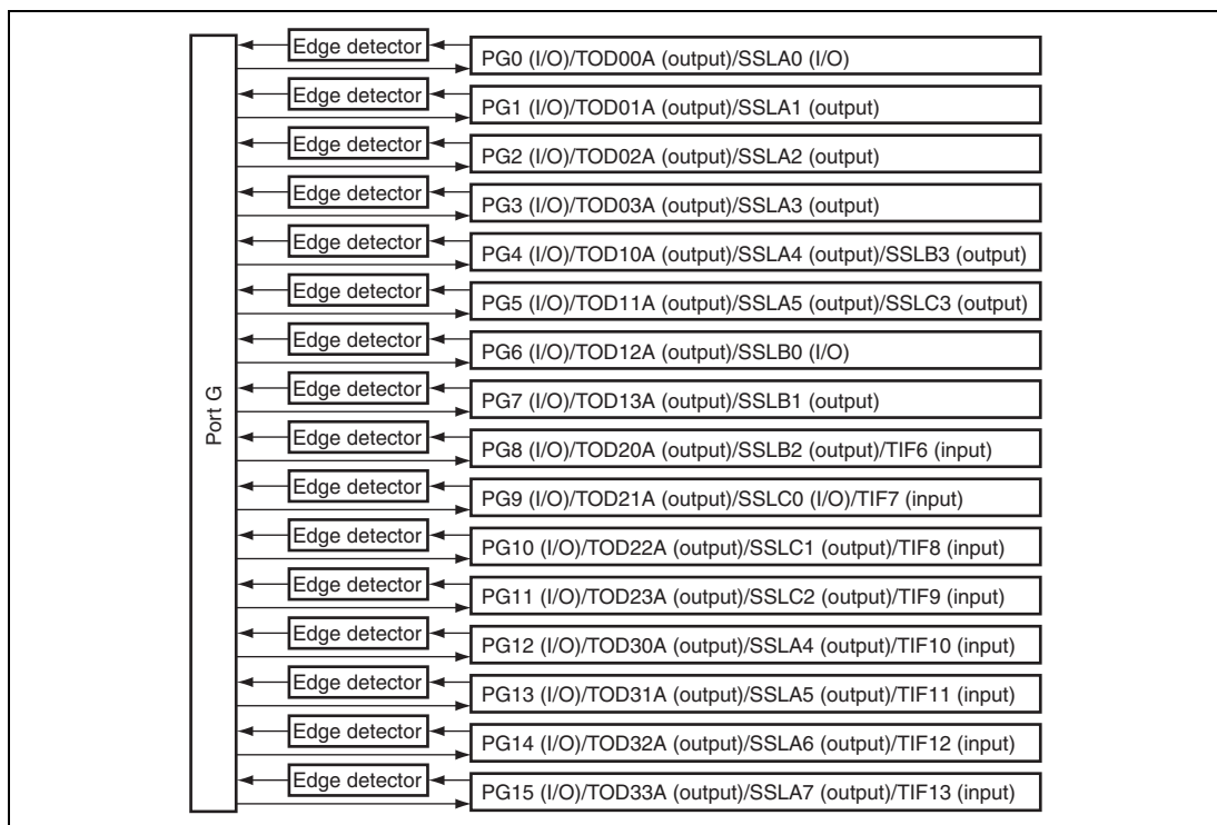
Figure 23.7 Port G
