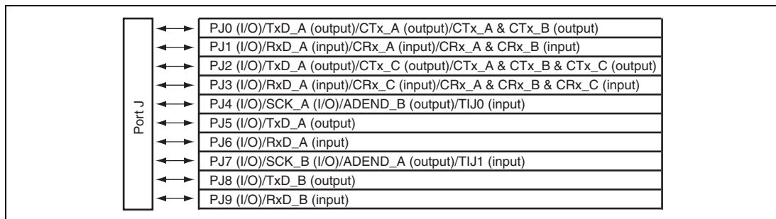
Figure 23.9 Port J
