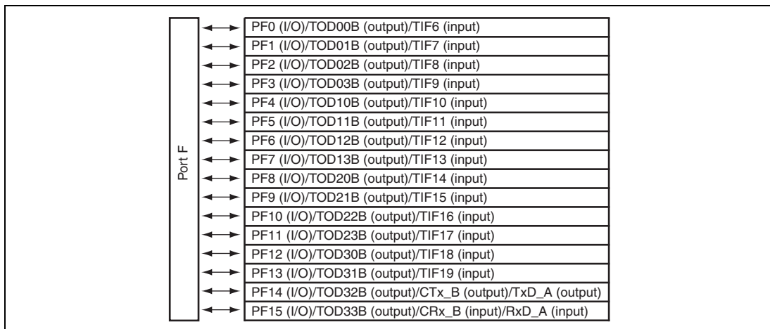
Figure 23.6 Port F
