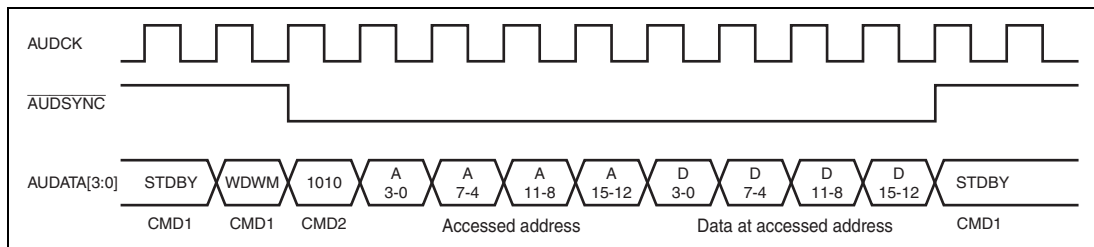
Figure 21.6 Window Data Tracing using WDW Command (M Bus, Lower 16 Bits of Address, Word-Size Data)
