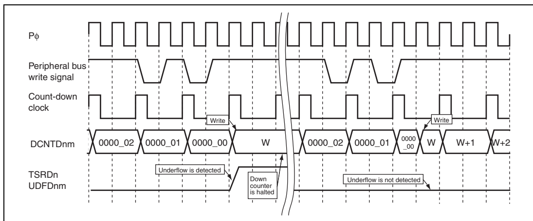
Figure 13.75 Conflict between Writing to DCNTDnm and Underflow
