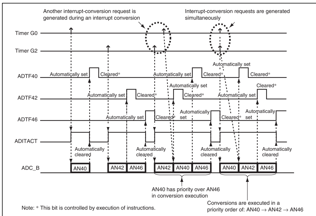
Figure 19.6 Example Operation of Interrupt Conversion
