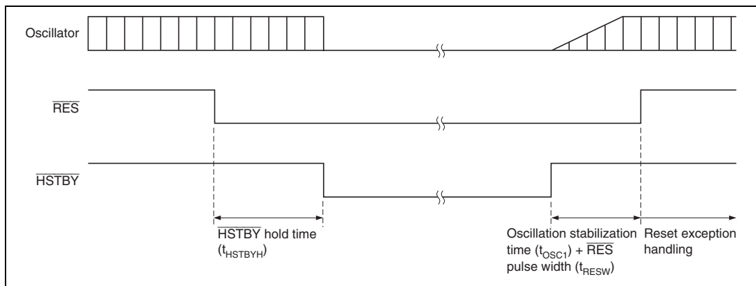
Figure 29.2 Timing in Hardware Standby Mode
