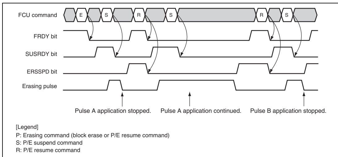
Figure 25.28 Suspending Erasure Processing (Suspension-Priority Mode)
