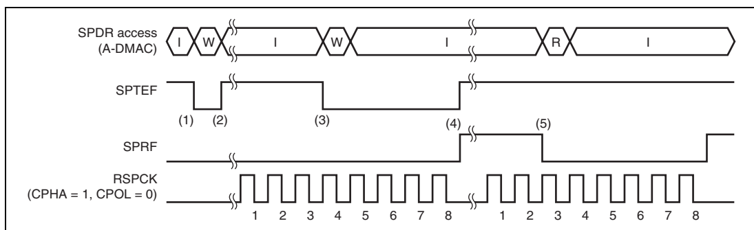
Figure 17.14 SPTEF and SPRF Bit Operation Example
