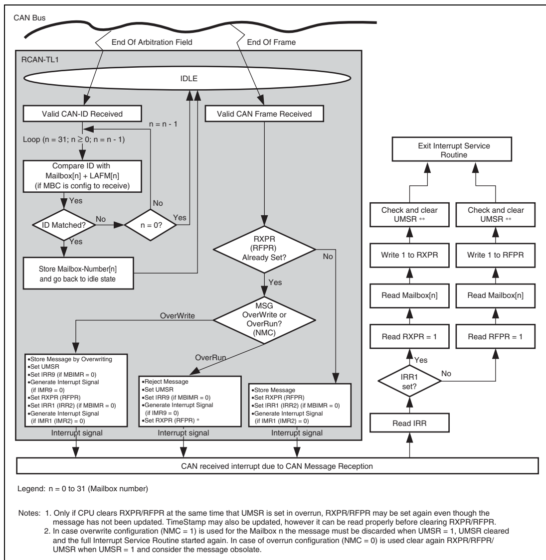
Figure 18.24 Message receive sequence
