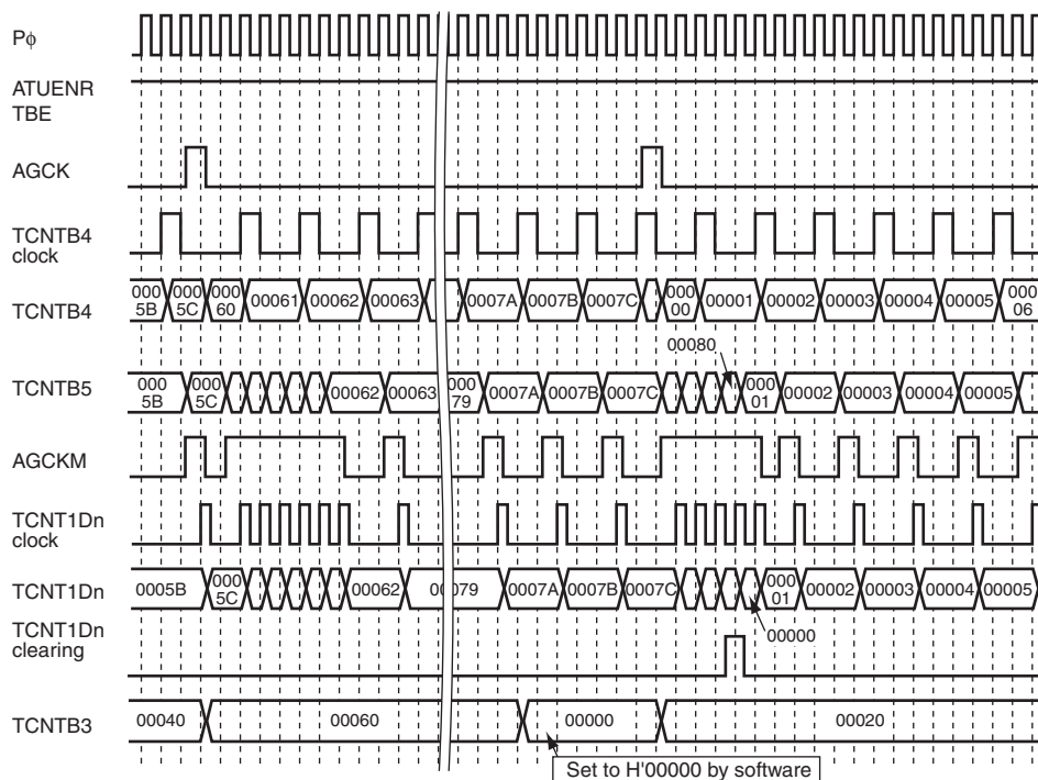
Figure 13.21 Operation of TCNTB5 (with Correction at End of Cycle)
