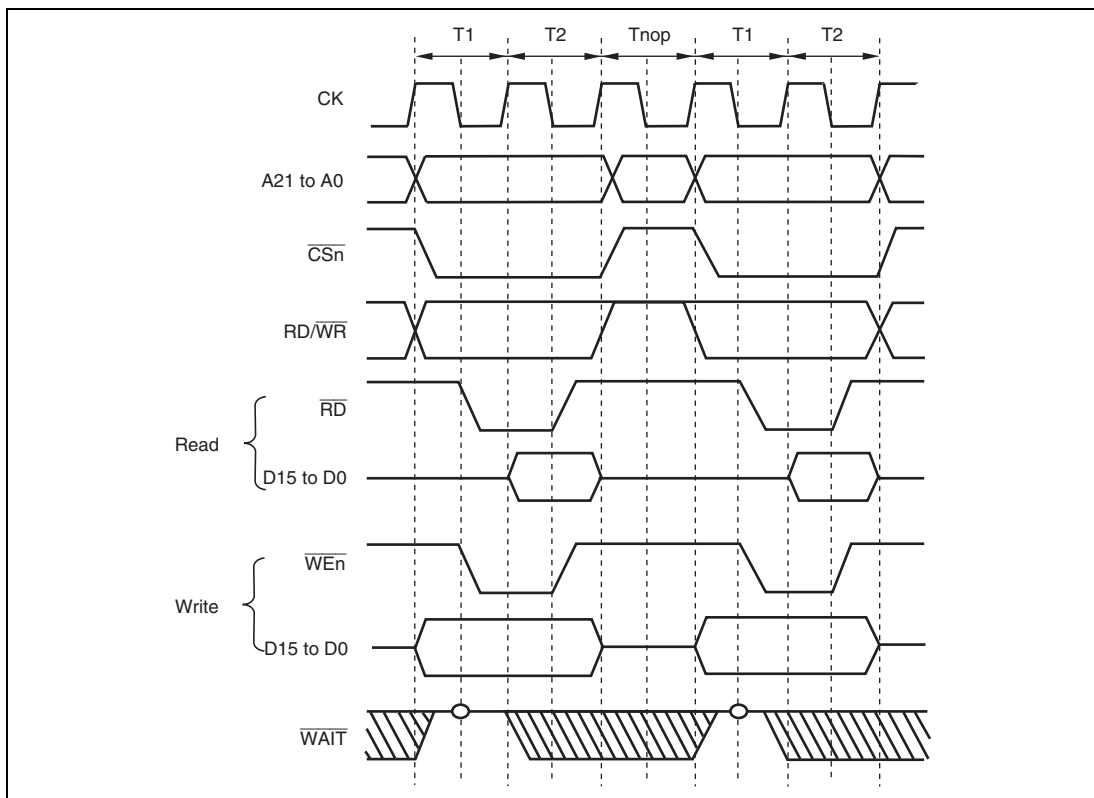
Figure 10.3 Continuous Access 1
