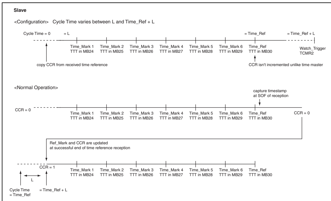
Figure 18.20 Time Slave
