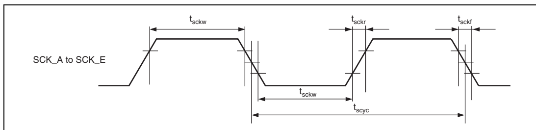
Figure 32.18 SCK Input Timing
