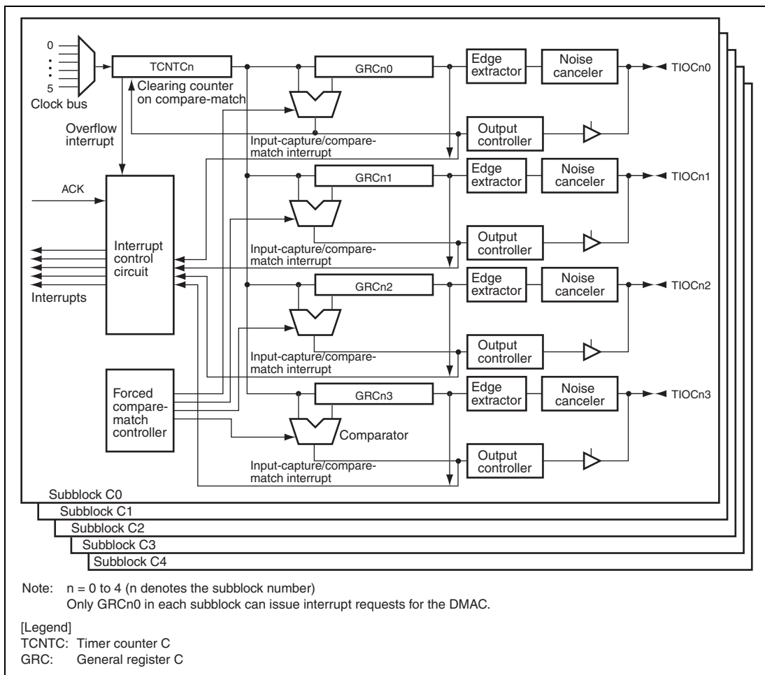
Figure 13.23 Block Diagram of Timer C
