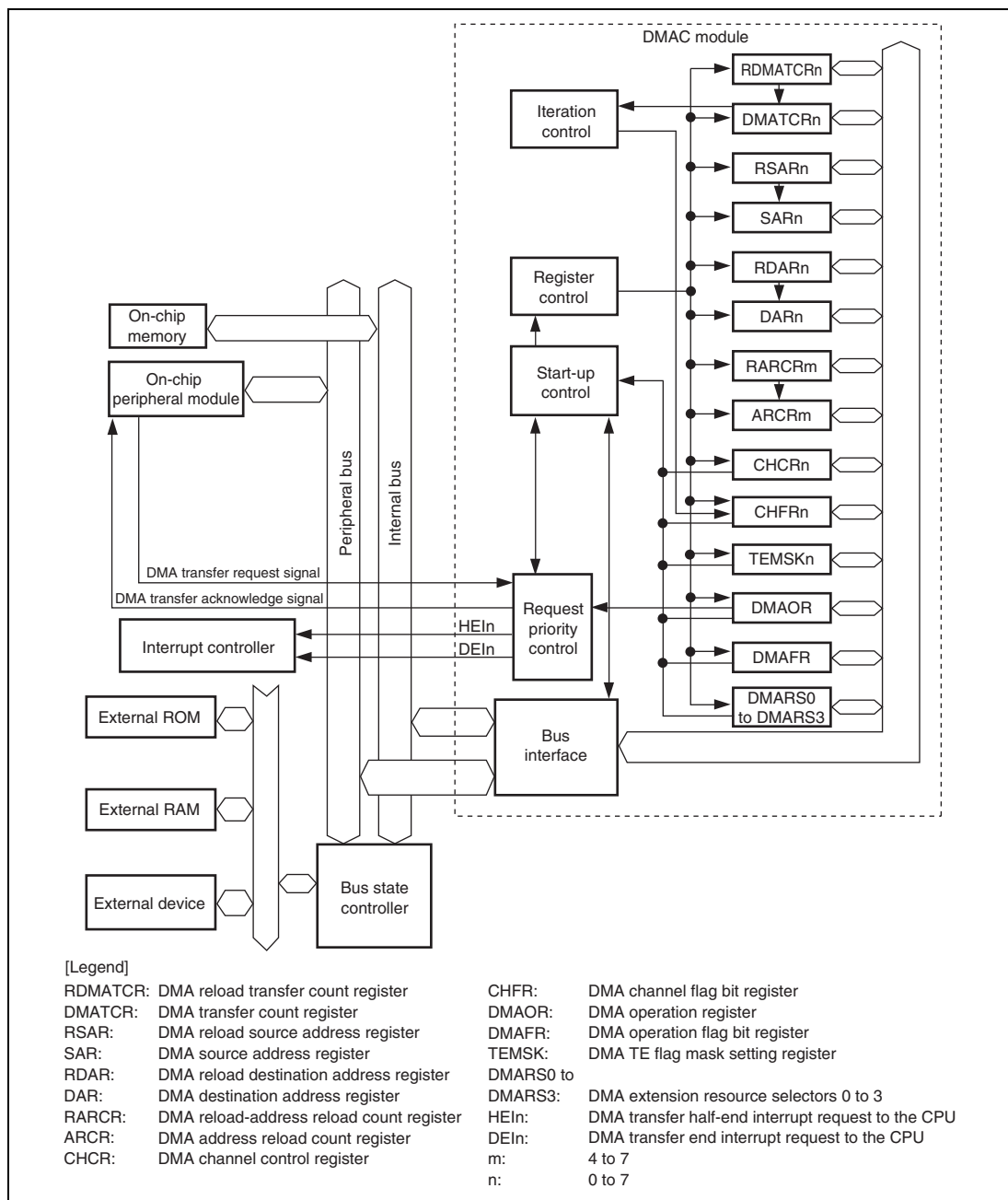
Figure 11.1 Block Diagram of DMAC
