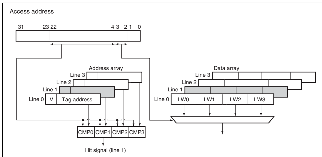
Figure 27.2 Concept of Looking up the Data Cache (with Line 1 being Hit)
