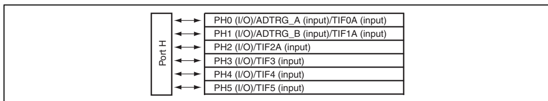
Figure 23.8 Port H
