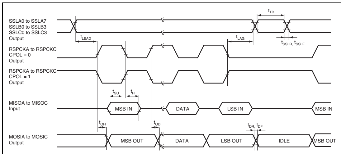
Figure 32.23 SPI Timing (Master, CPHA = 1)
