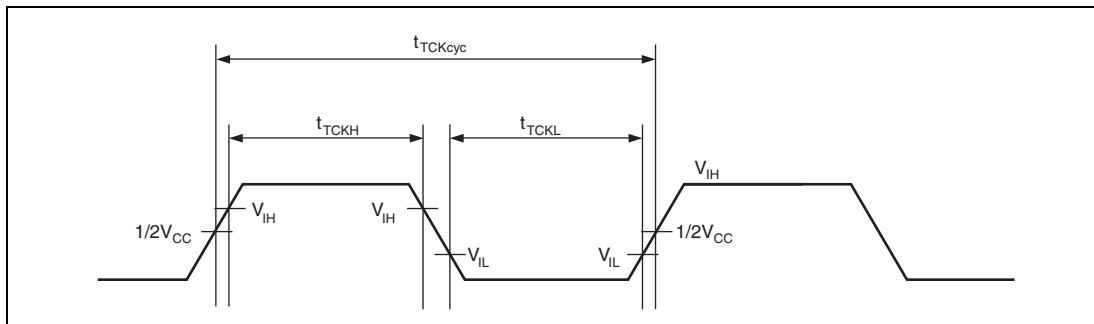
Figure 32.30 JTAG Interface Clock Timing
