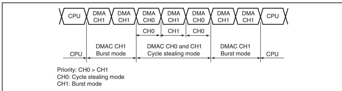
Figure 11.10 Bus State when Multiple Channels are Operating
