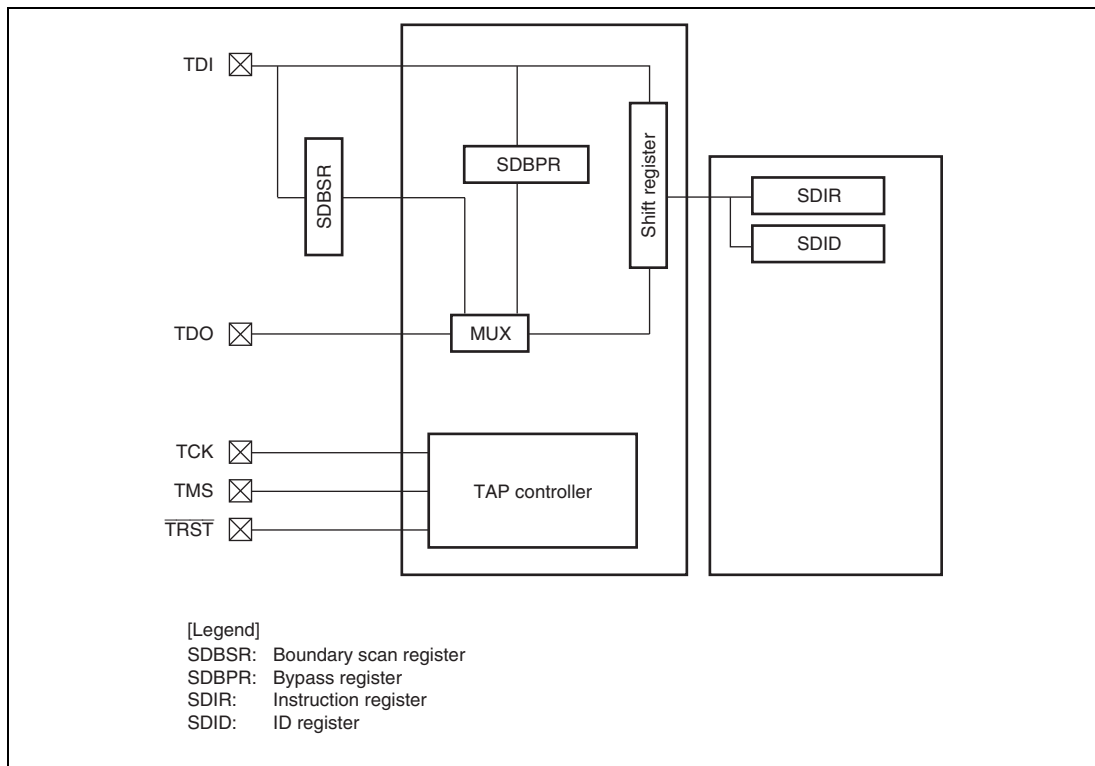
Figure 20.1 Block Diagram of JTAG Interface
