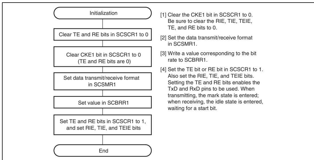
Figure 16.3 Sample Flowchart for SCI Initialization
