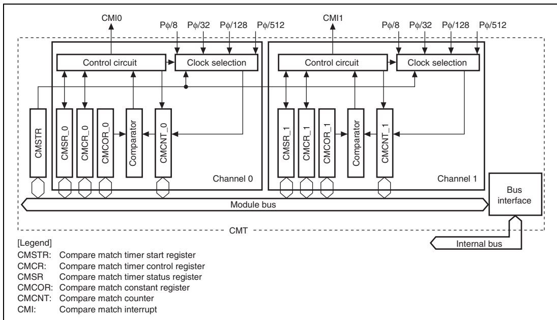
Figure 15.1 Block Diagram of CMT
