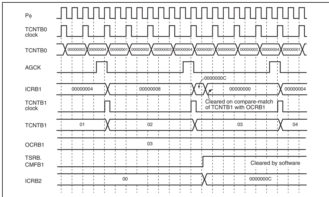
Figure 13.14 Compare-Match Operation of TCNTB1 and Capture Operation of ICRB1 and ICRB2
