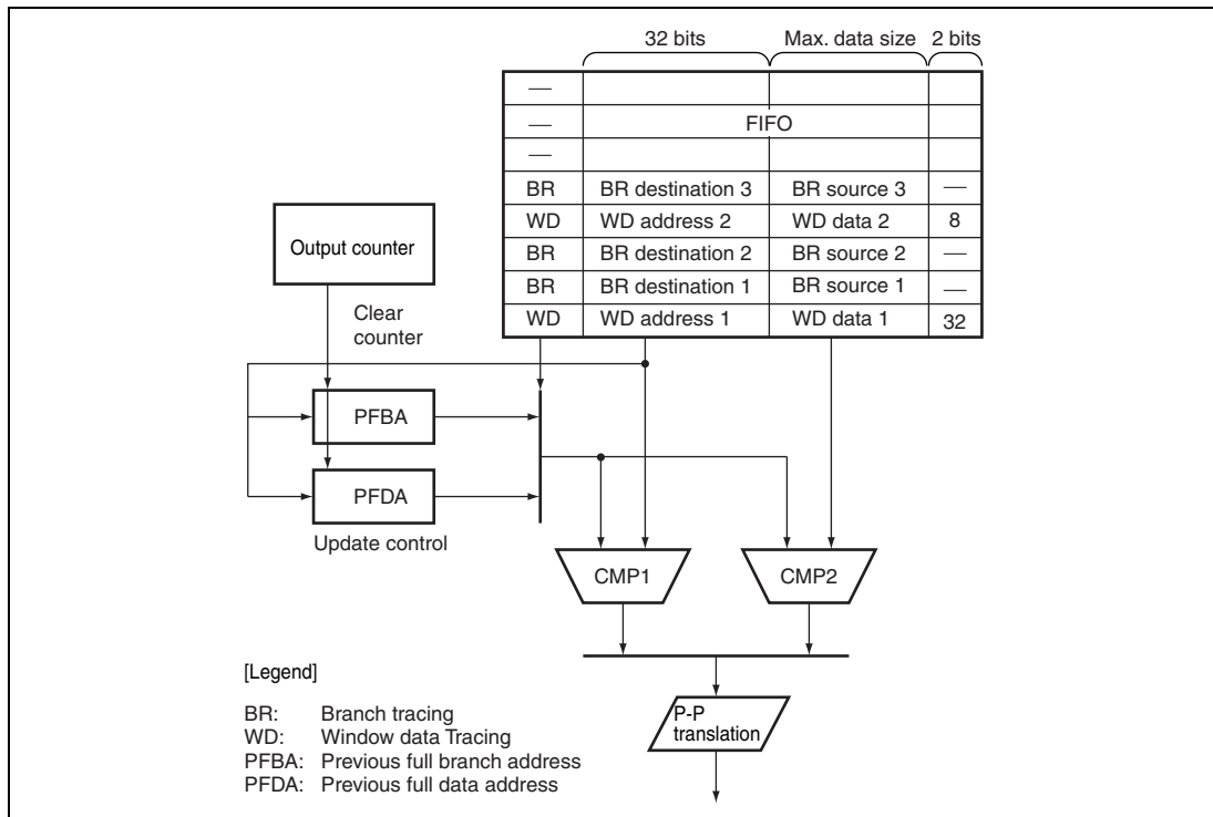
Figure 21.10 Example of Address Comparison
