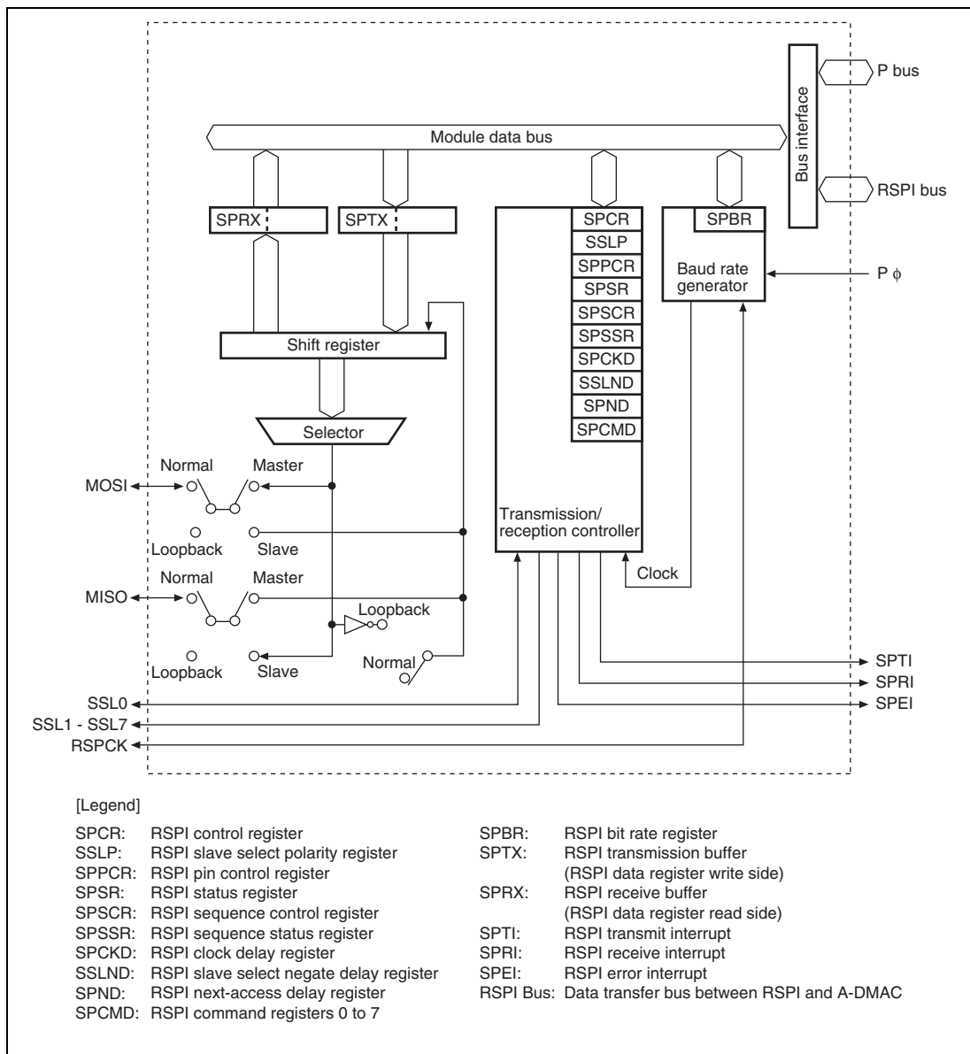
Figure 17.1 Block Diagram of RSPI (for One Channel)
