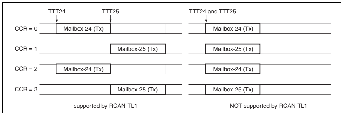
Figure 18.18 Limitation on Tx-Trigger Time
