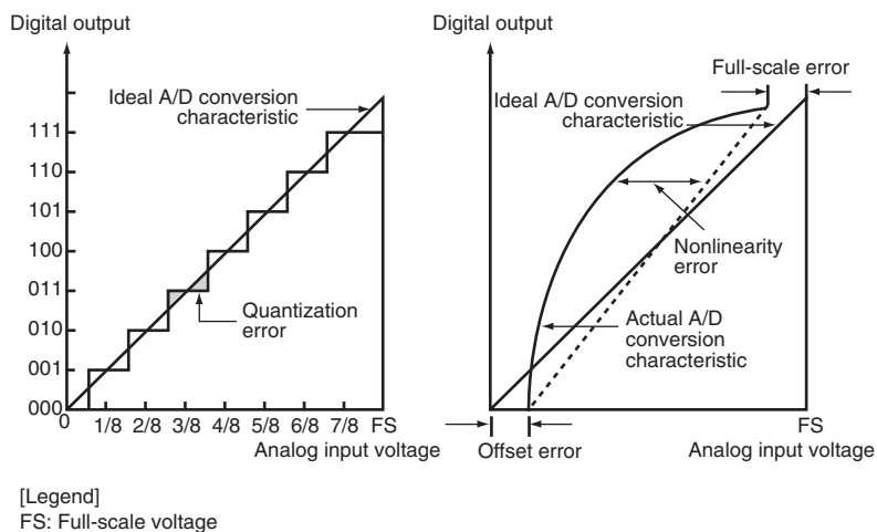
Figure 19.11 Definition of A/D Conversion Accuracy
