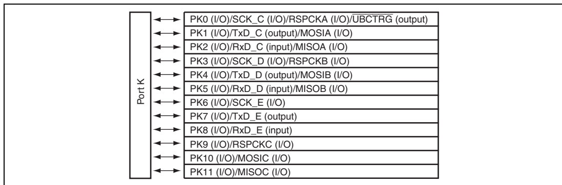
Figure 23.10 Port K
