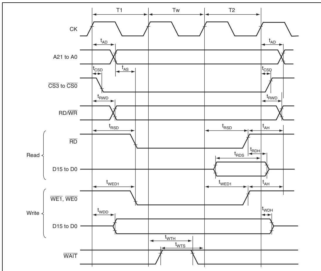
Figure 32.9 Bus Timing (One Software Wait Cycle)
