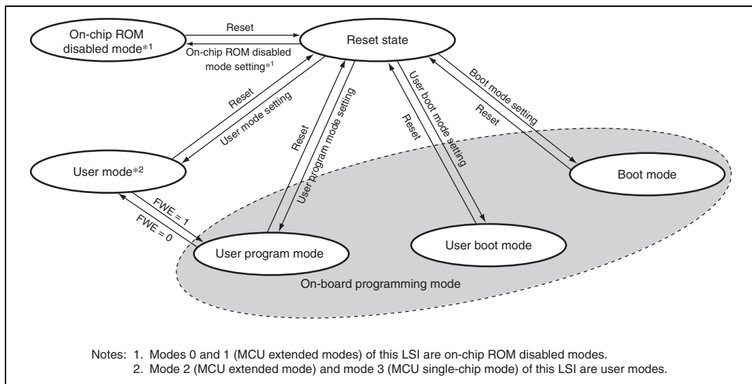
Figure 25.4 ROM-Related Mode Transition
