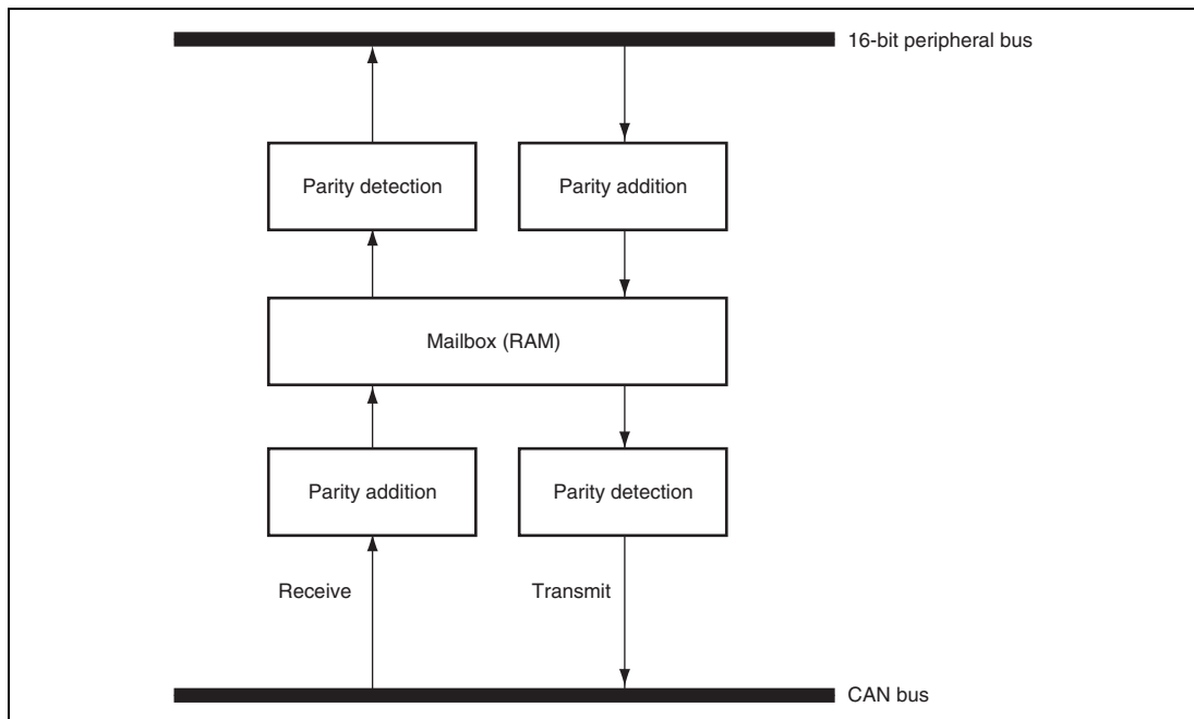
Figure 18.26 Parity Addition and Detection
