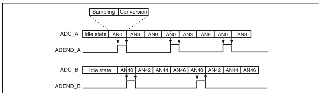
Figure 19.10 Example of ADEND_A and ADEND_B Outputs
