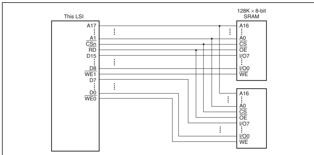
Figure 10.7 Example of 16-Bit Data-Width SRAM Connection
