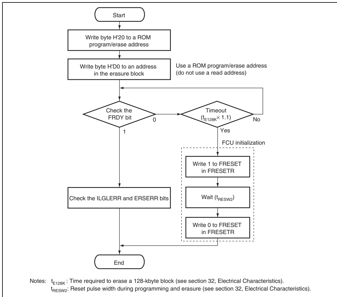
Figure 25.19 Procedure for ROM Erasure
