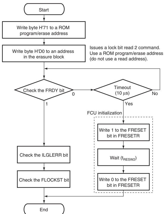
Figure 25.25 Procedure for Reading Lock Bit in Register Read Mode
