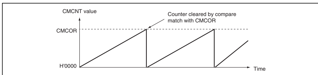
Figure 15.2 Counter Operation
