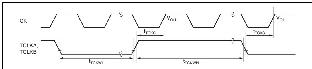
Figure 32.15 ATU Clock Input Timing
