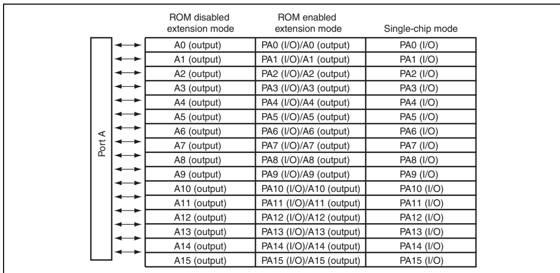
Figure 23.1 Port A
