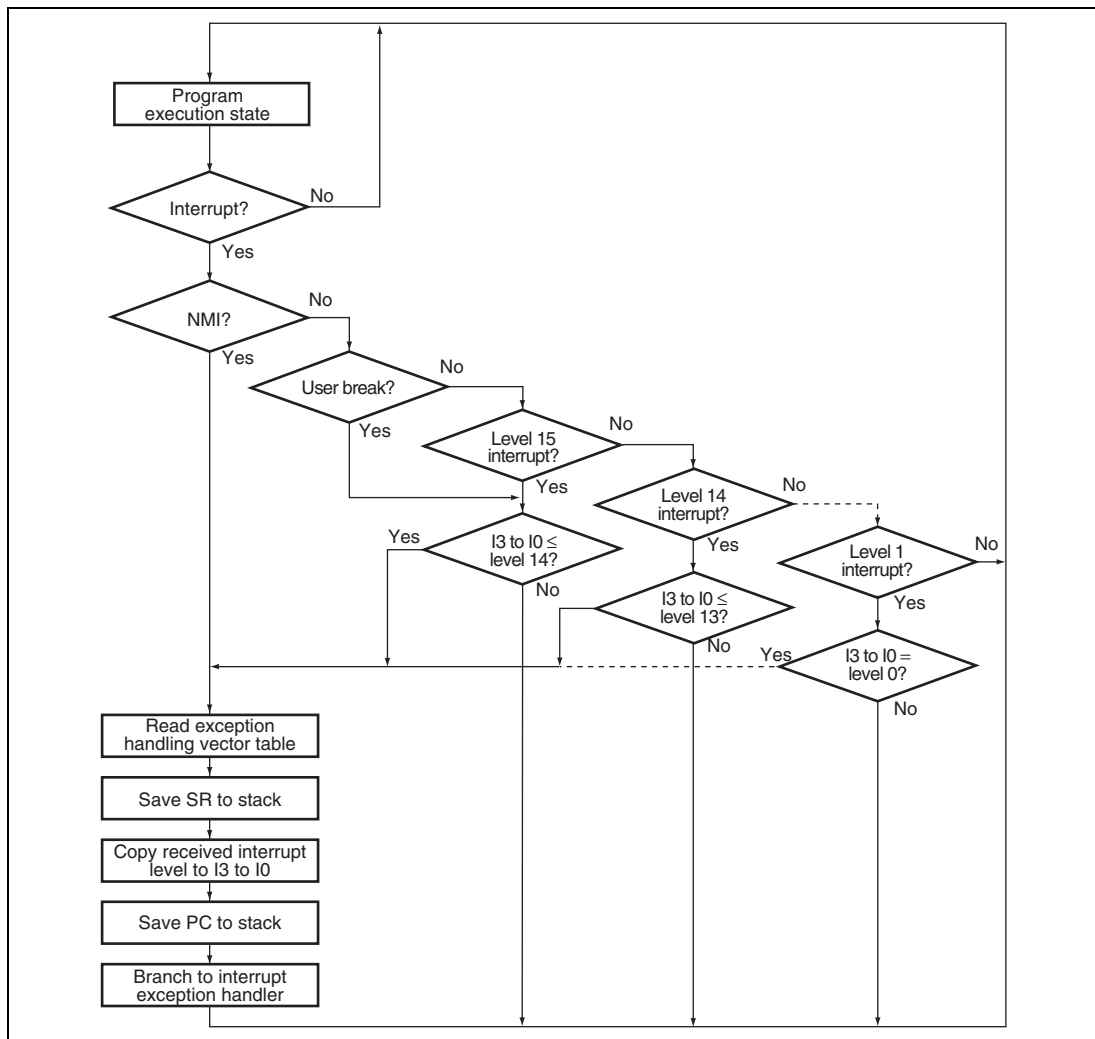
Figure 8.2 Interrupt Operation Flow
