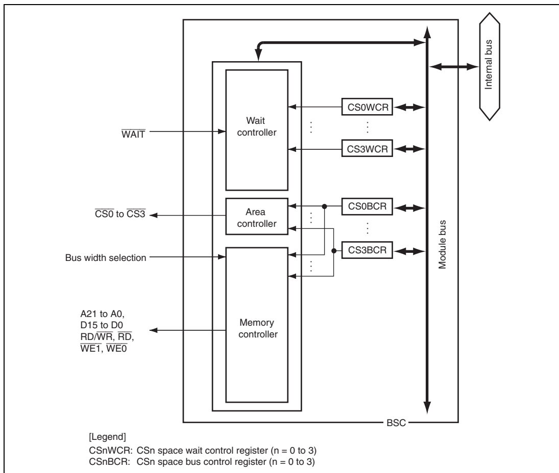
Figure 10.1 Block Diagram of BSC
