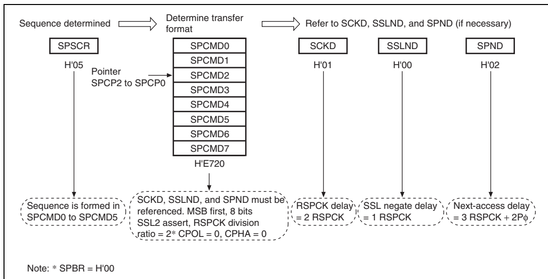
Figure 17.16 Determination Procedure of Serial Transfer Mode in Master Mode
