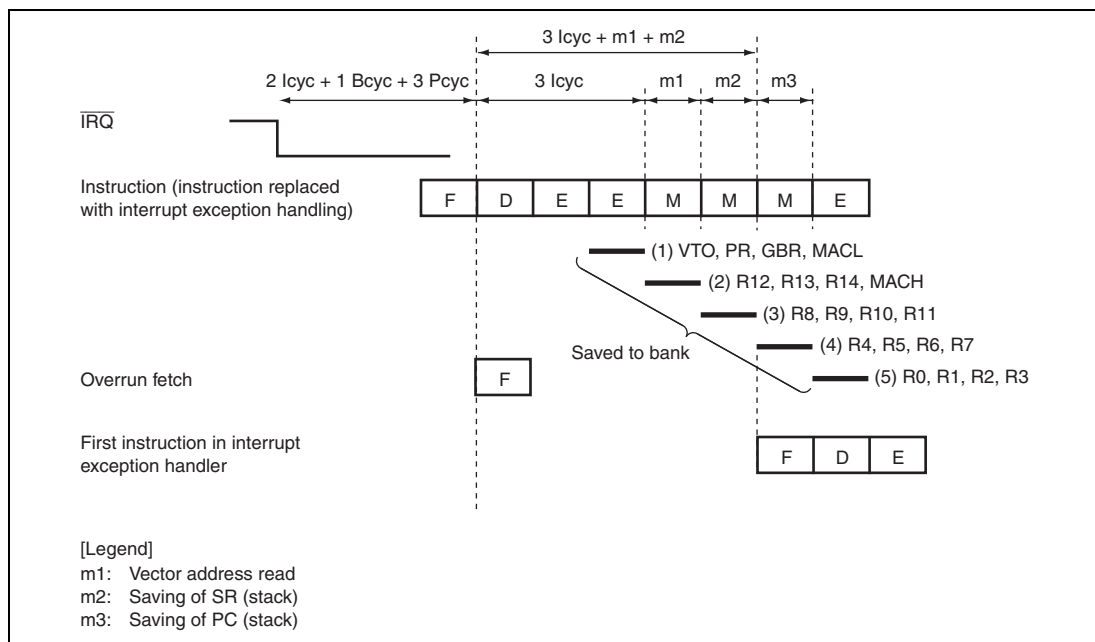
Figure 8.12 Bank Save Timing
