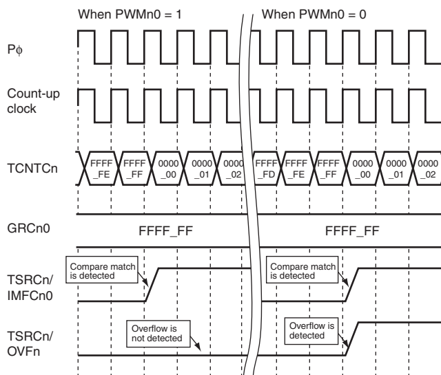
Figure 13.72 Conflict between Counter Clearing by Compare Match of Timer C and Overflow (PWMn0 = 1/0)
