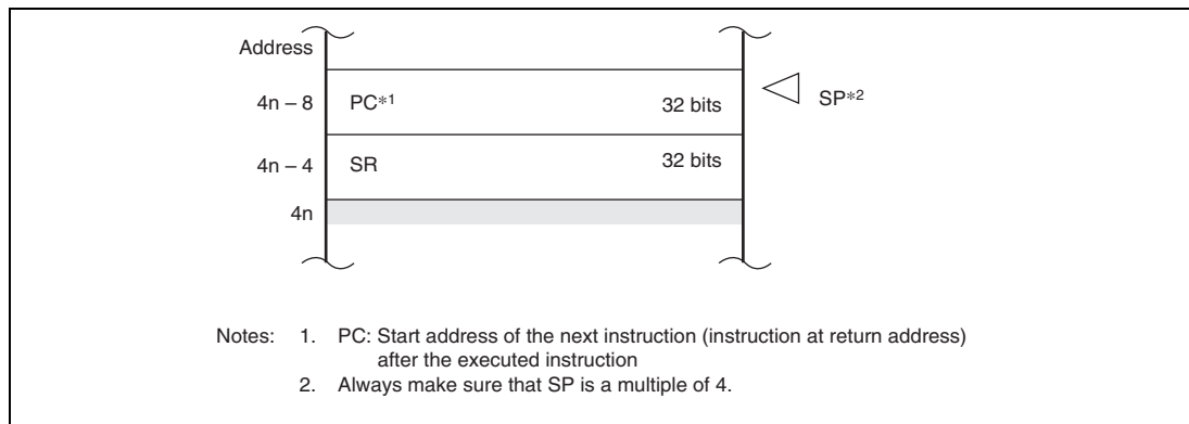
Figure 8.3 Stack after Interrupt Exception Handling
