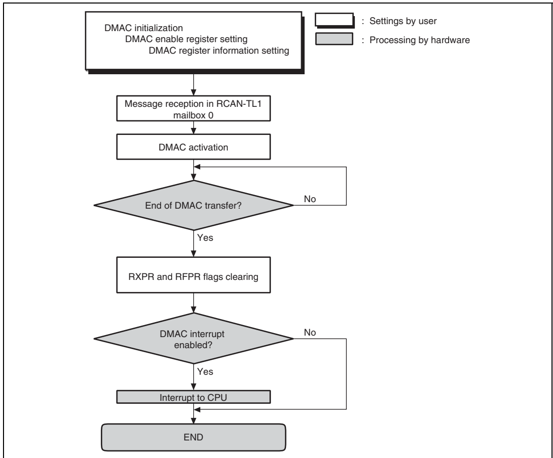
Figure 18.27 DMAC Transfer Flowchart
