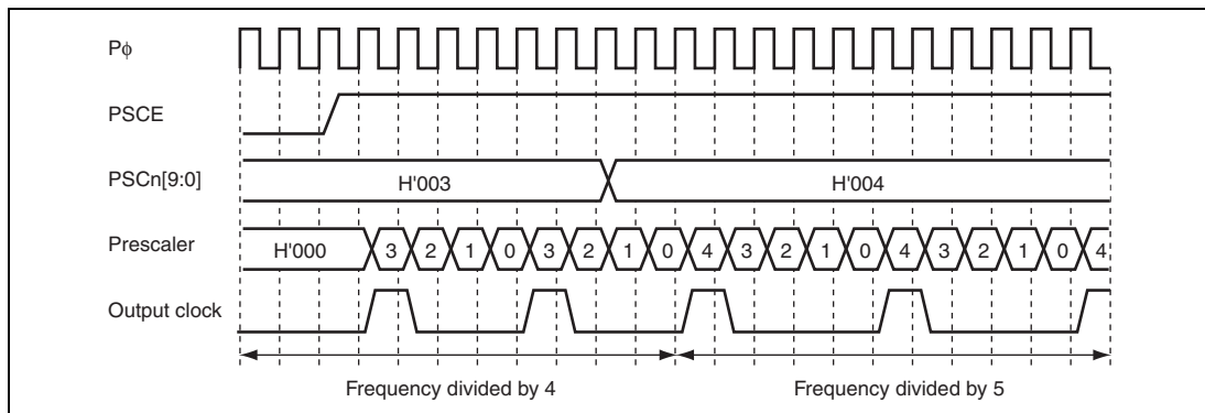
Figure 13.3 Starting Prescaler
