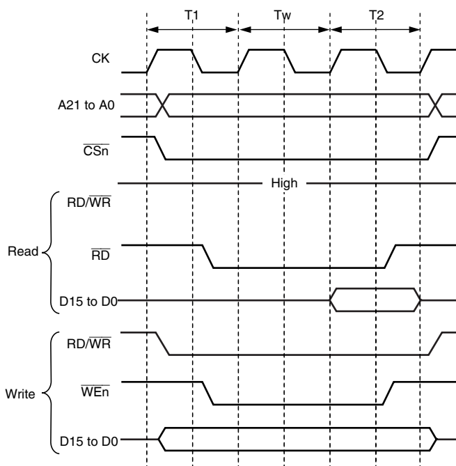
Figure 10.5 Basic Access for Two-Times Multiplied Peripheral Clock (Access Wait 1)
