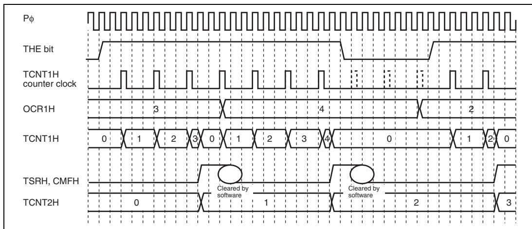
Figure 13.48 Operations of Timer H
