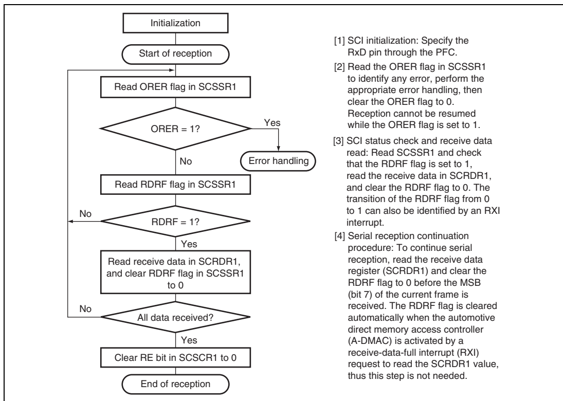
Figure 16.12 Sample Flowchart for Receiving Serial Data (1)
