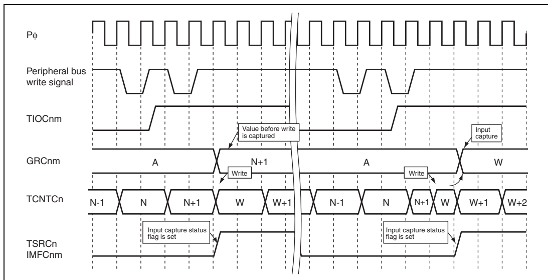
Figure 13.53 Conflict between Writing to TCNTCn and Input Capture
