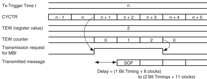
Figure 18.23 Timing Diagram of Timer
