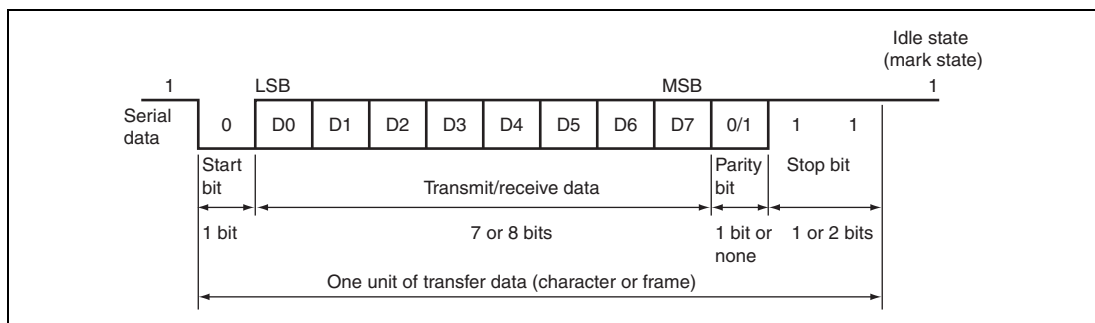
Figure 16.2 Example of Data Format in Asynchronous Communications (8-Bit Data with Parity and Two Stop Bits)
