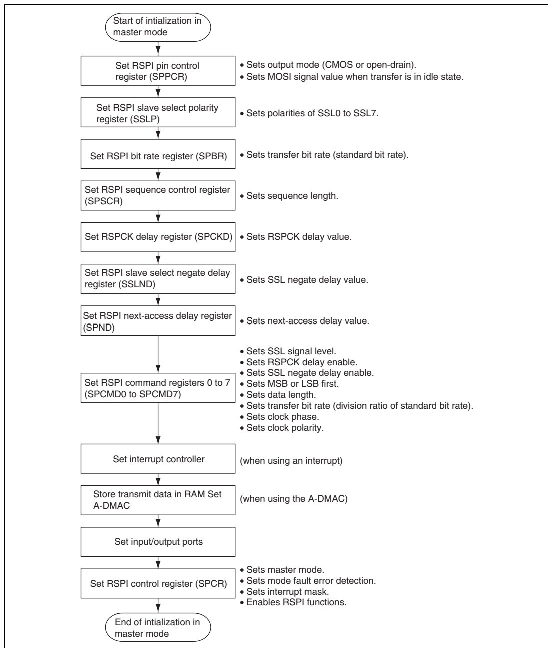
Figure 17.18 Example of Initialization Flowchart in Master Mode
