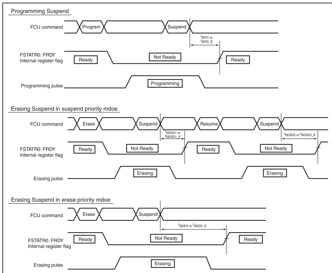
Figure 32.38 Flash Programming/Erasing Suspend Timing
