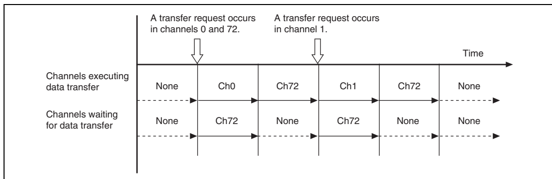
Figure 12.13 Channel Priorities
