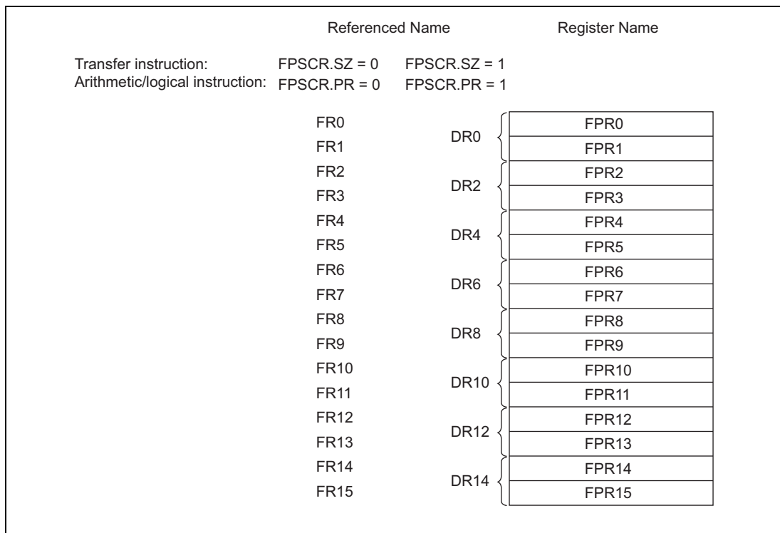
Figure 2.5 Floating-Point Registers
