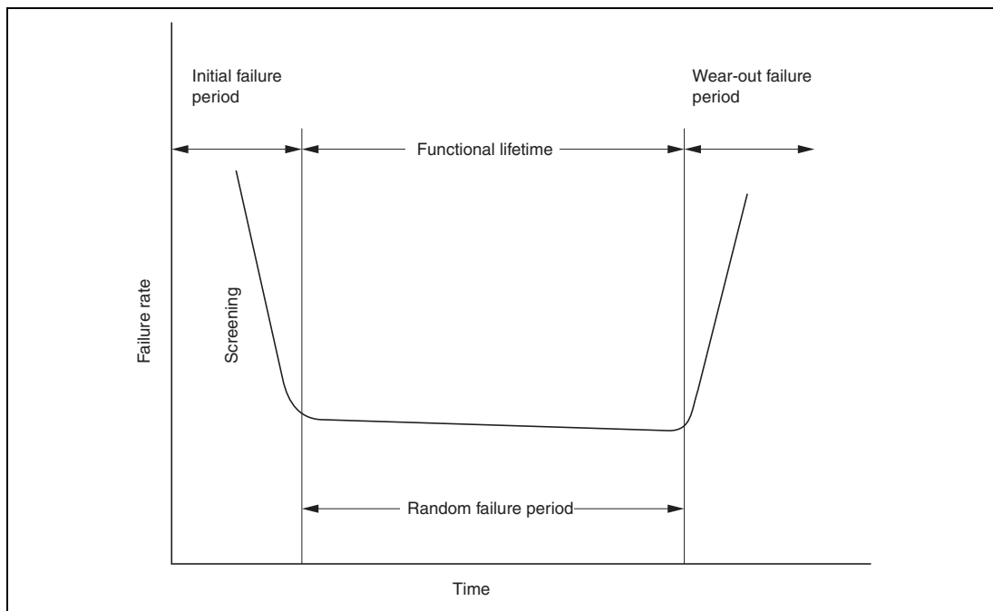
Figure 30.1 Failure Rate Curve (Bathtub Curve)
