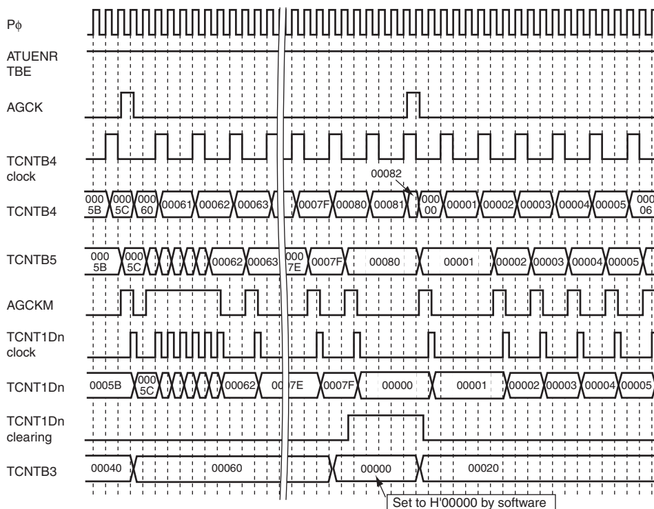
Figure 13.22 Operation of TCNTB5 (without Correction at End of Cycle)
