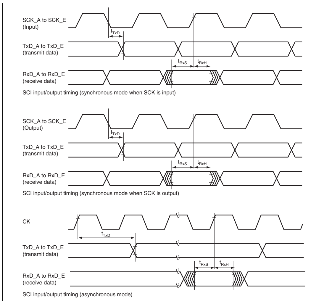
Figure 32.19 SCI Input/Output Timing
