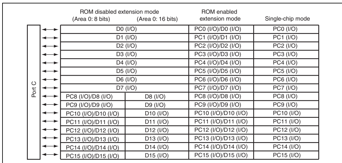
Figure 23.3 Port C
