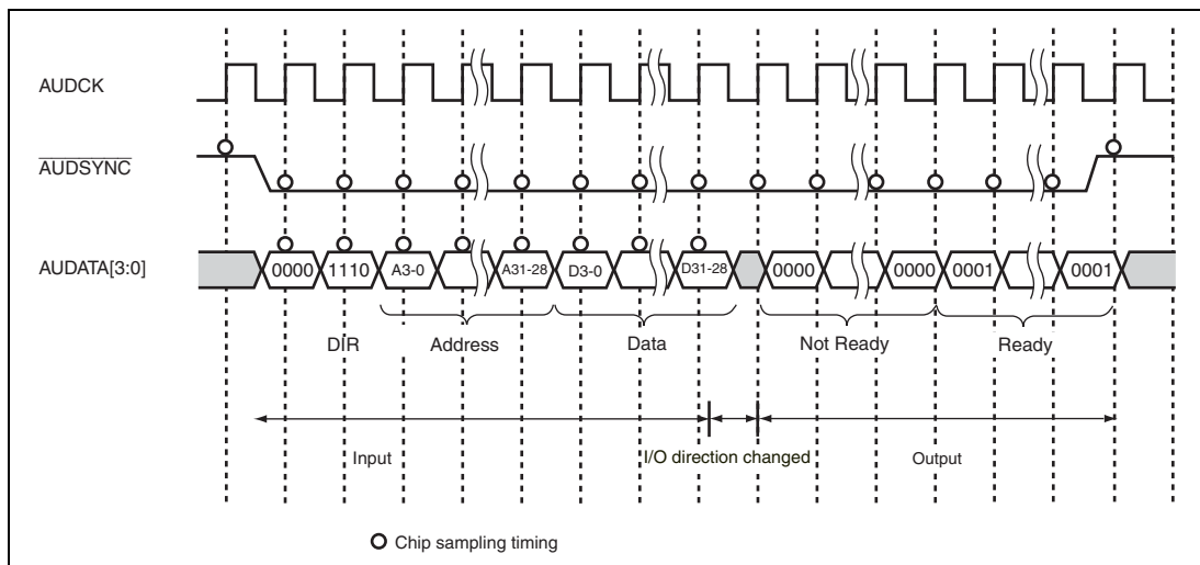
Figure 21.12 Example Operation of Byte Read
