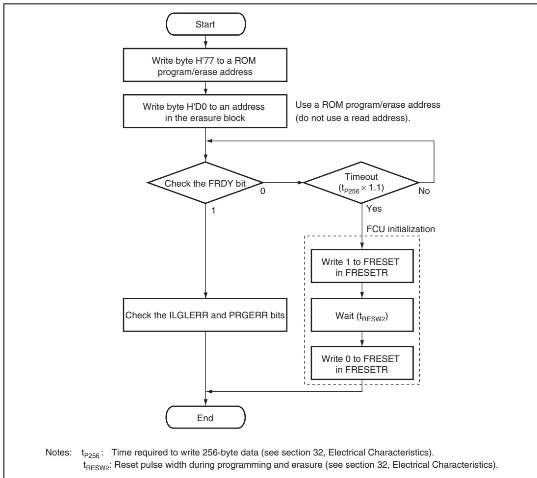
Figure 25.26 Procedure for Writing to the Lock Bit
