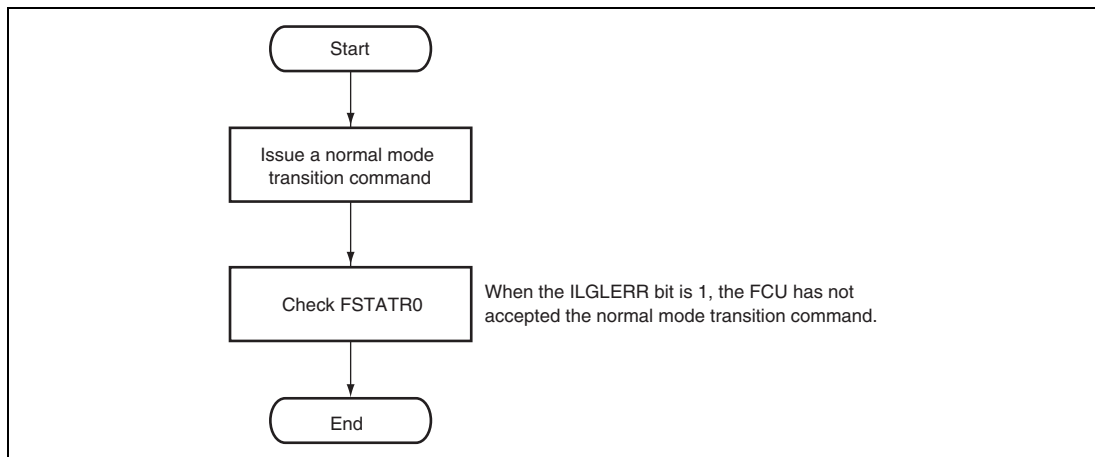
Figure 25.17 Procedure to Use ROM P/E Normal Mode Transition Command
