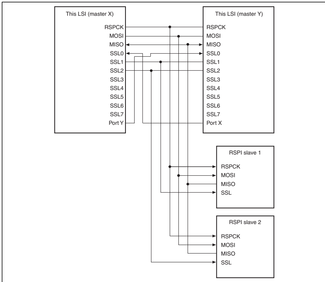
Figure 17.7 Multi-Master/Multi-Slave Configuration Example (This LSI = Master)
