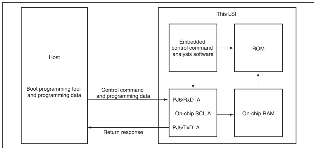
Figure 25.5 System Configuration in Boot Mode
