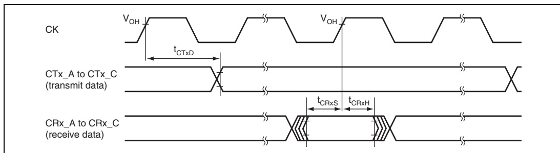
Figure 32.20 CAN Input/Output Timing
