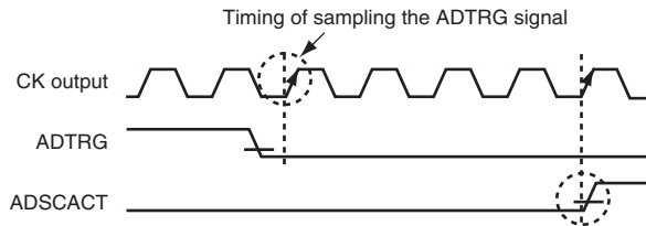
Figure 19.9 External Trigger Input Timing
