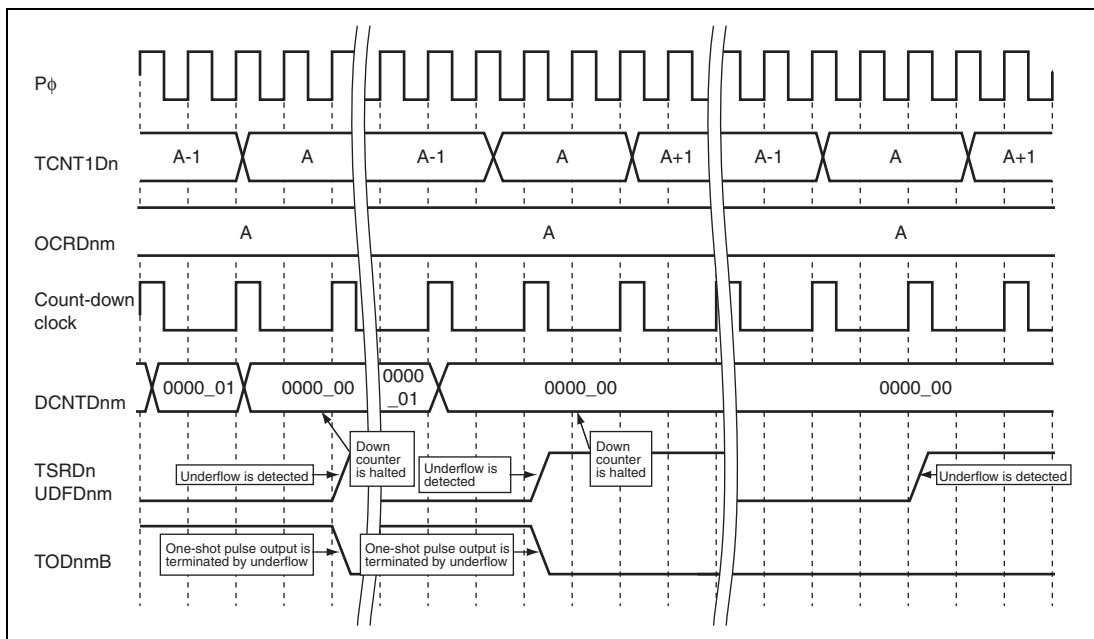
Figure 13.79 Conflict between Compare Match A and Underflow
