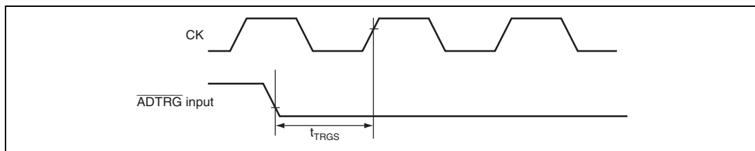
Figure 32.26 External Trigger Input Timing
