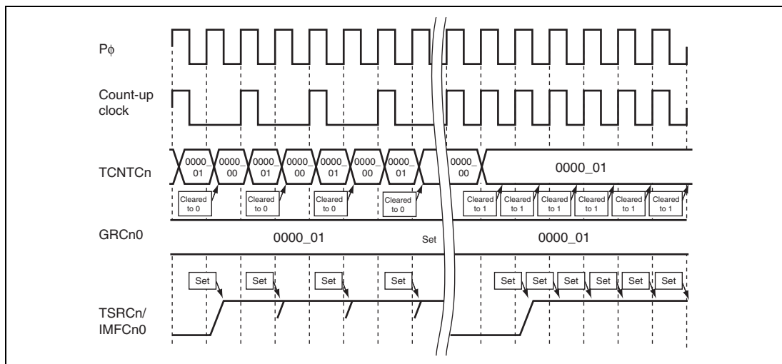
Figure 13.68 Simultaneous Occurrence of Count-Up and Counter Clearing
