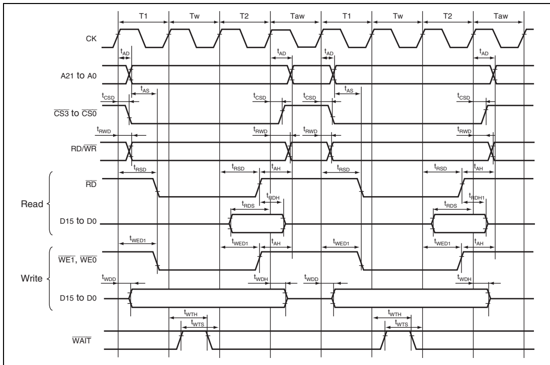
Figure 32.11 Bus Timing
