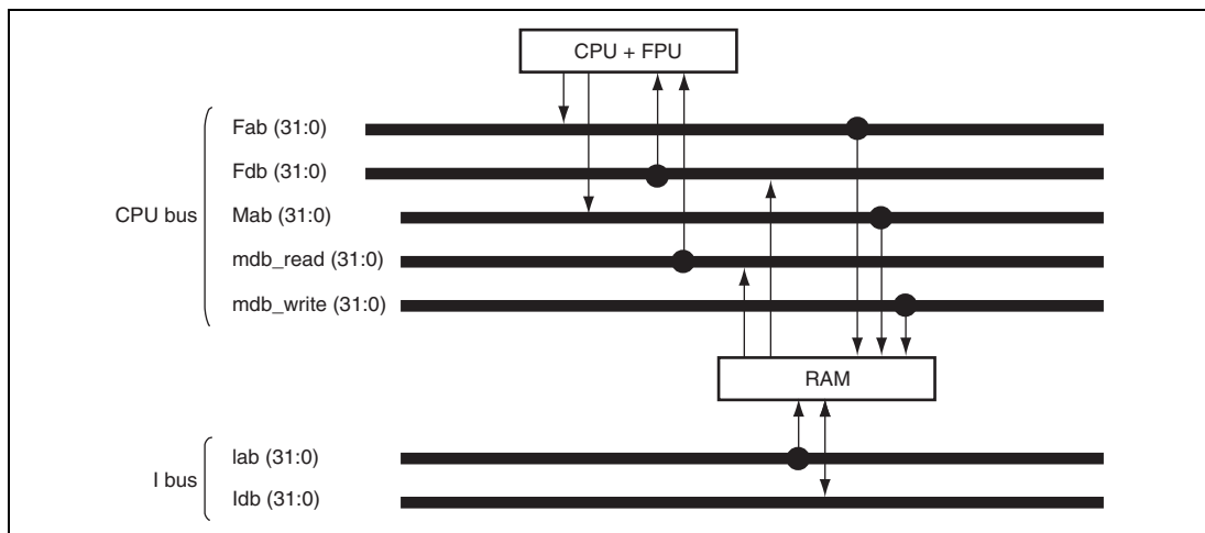
Figure 28.2 Bus Connections in RAM
