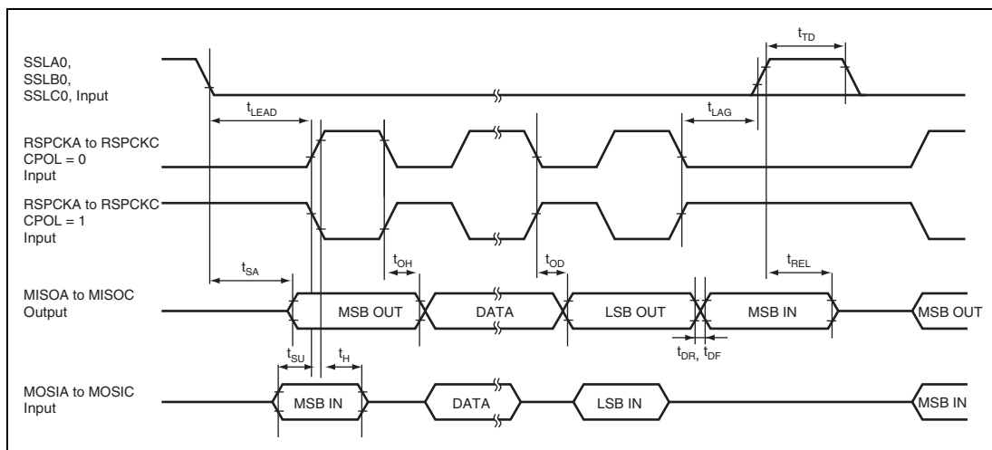
Figure 32.24 SPI Timing (Slave, CPHA = 0)
