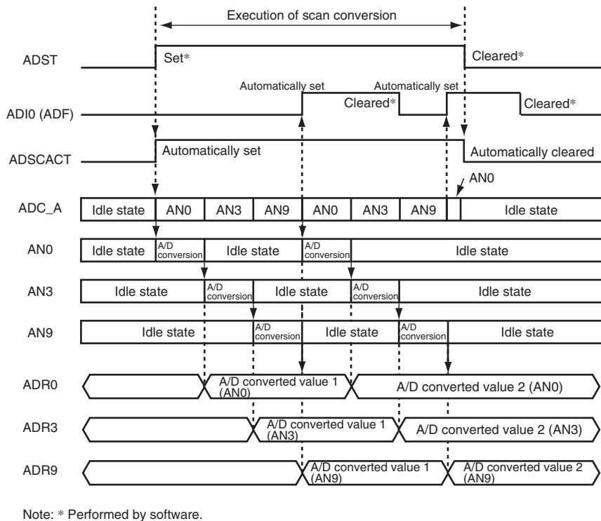
Figure 19.5 Example Operation in Continuous Scan Mode
