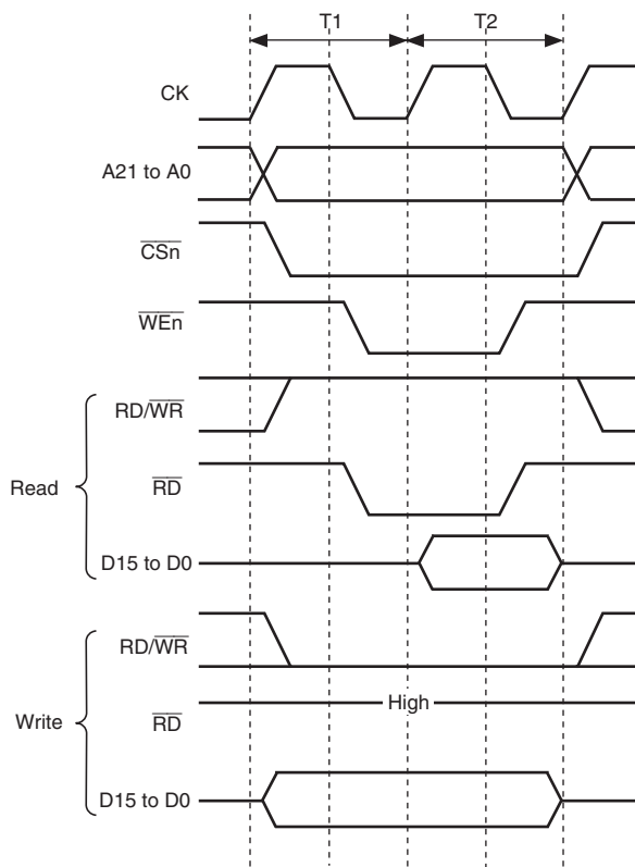
Figure 10.12 Basic Access Timing for SRAM with Byte Selection (BAS = 0)
