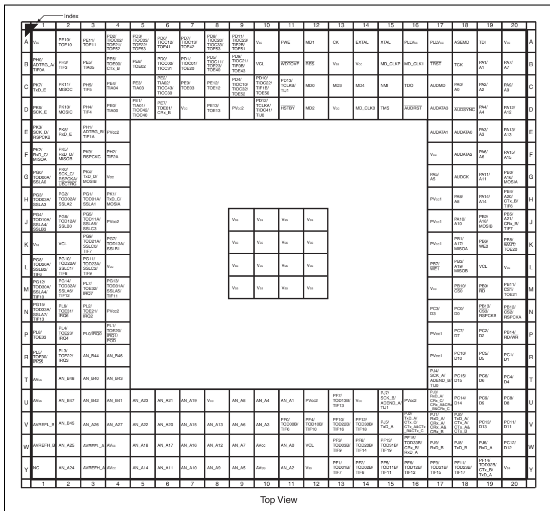
Figure 1.2 Pin Arrangements
