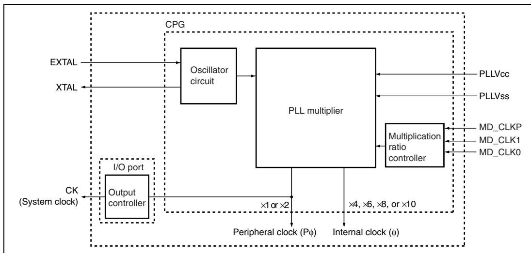
Figure 4.1 Block Diagram of CPG
