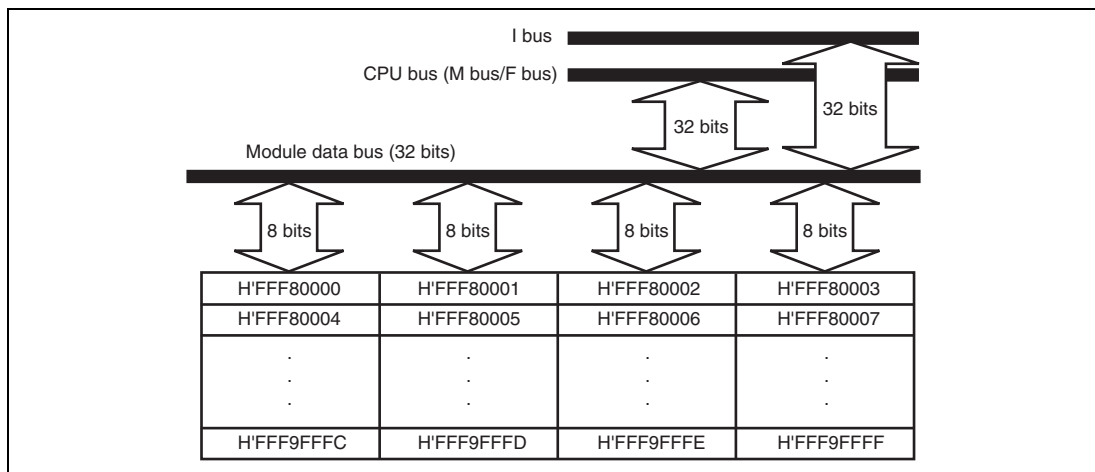
Figure 28.1 RAM Block Diagram
