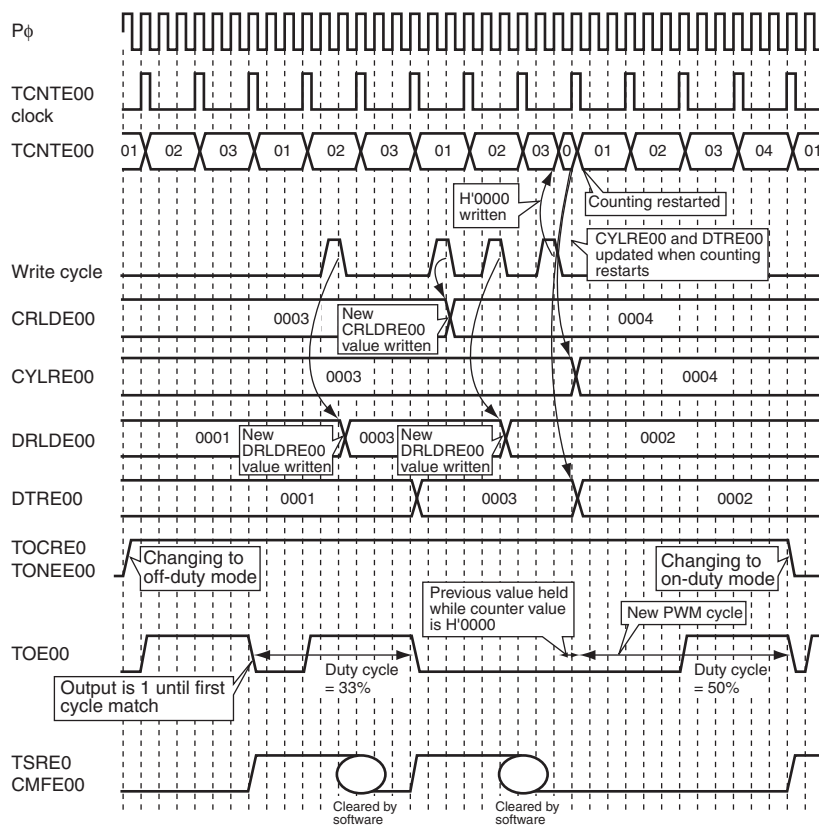
Figure 13.34 Operation of PWM (3)
