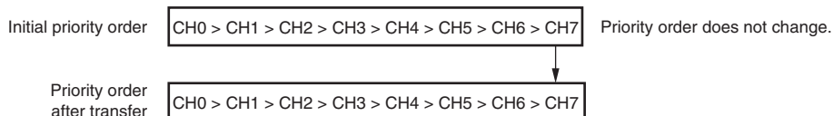
Figure 11.3 Round-Robin Mode
