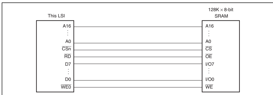
Figure 10.8 Example of 8-Bit Data-Width SRAM Connection
