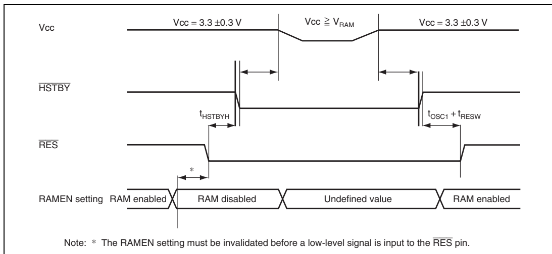
Figure 28.4 RAM Data Retention at Hardware Standby
