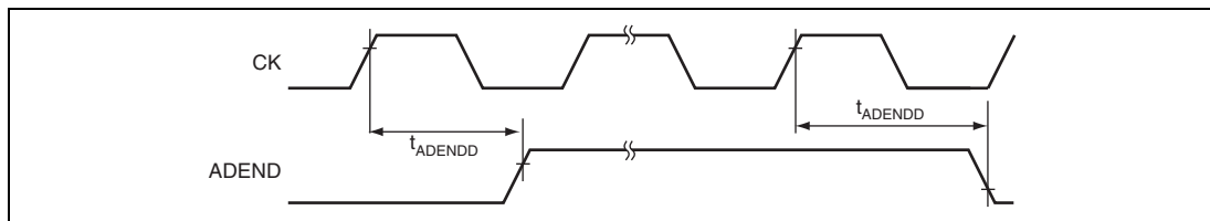
Figure 32.27 Analog Conversion Timing
