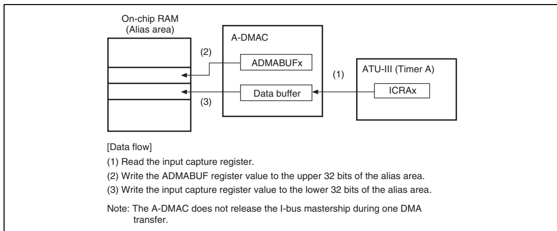
Figure 12.10 Data Flow in Channels for Timer A
