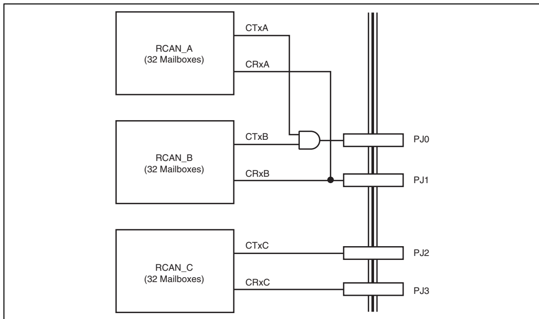
Figure 18.32 Connection Example when Using RCAN-TL1 as 2-Channel Module (64 Mailboxes × 1 Channel and 32 Mailboxes × 1 Channel)
