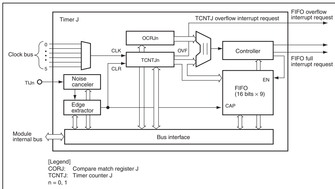
Figure 13.49 Block Diagram of Timer J
