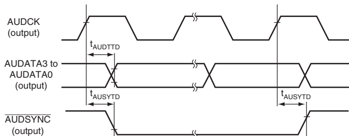
Figure 32.34 Trace Mode Timing
