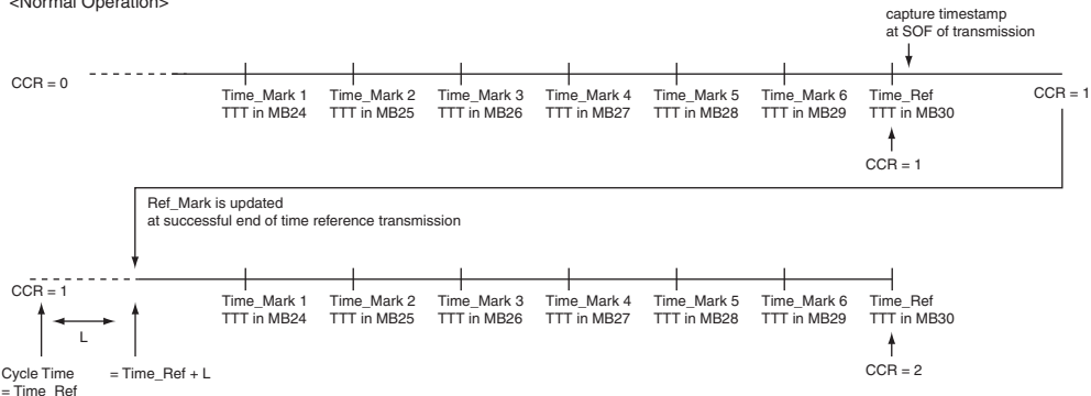
Figure 18.19 (Potential) Time Master
