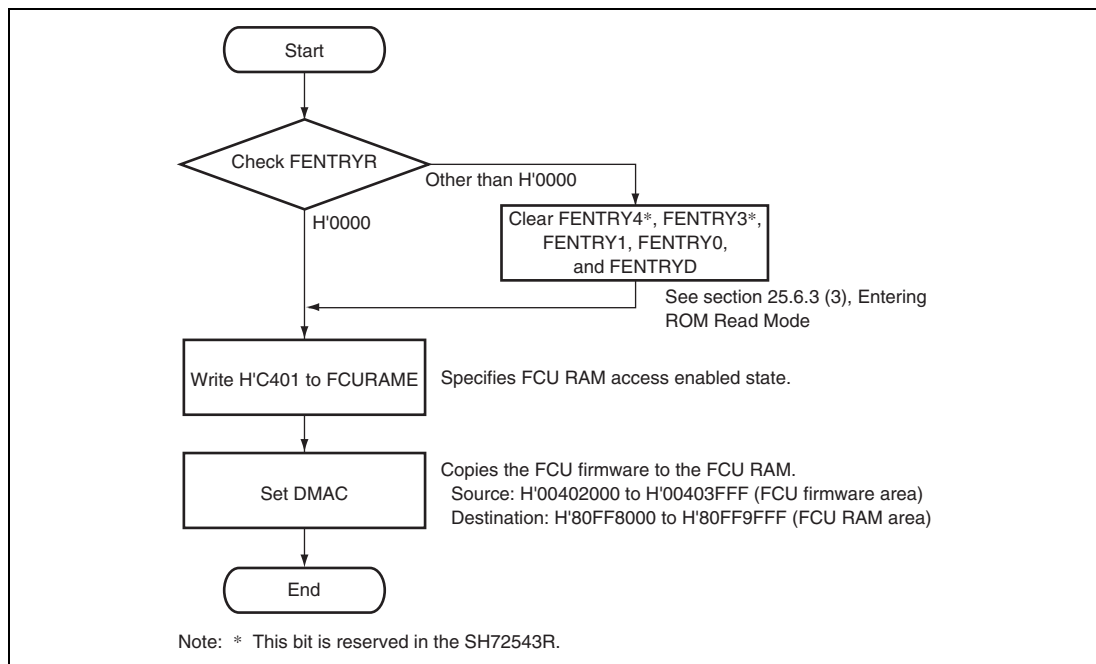
Figure 25.14 Procedure for Firmware Transfer to FCU RAM
