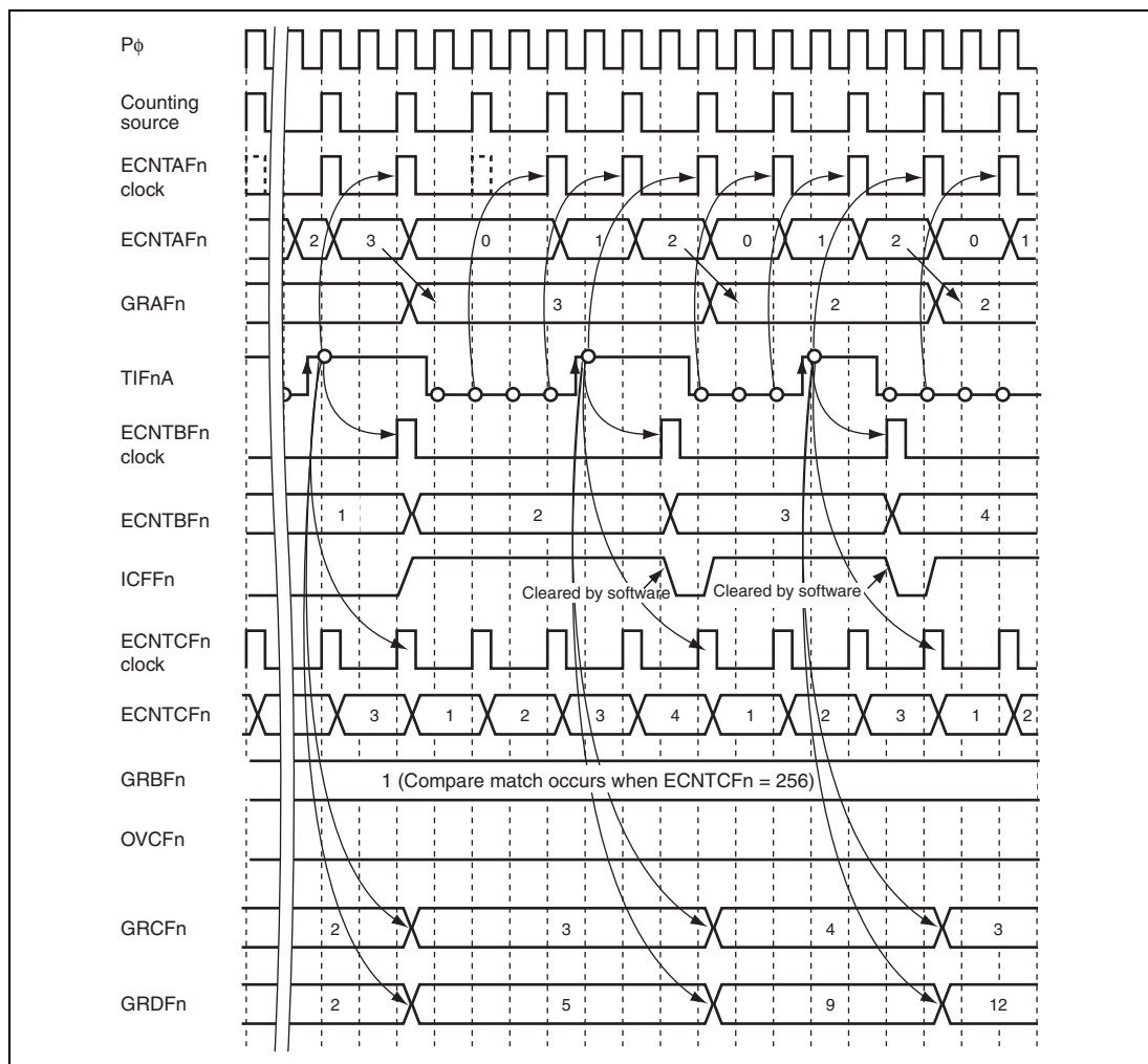
Figure 13.42 Operation Example of Rotation Speed/Pulse Measurement
