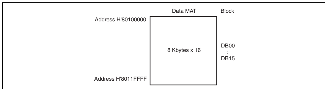
Figure 26.3 Block Configuration of Data MAT
