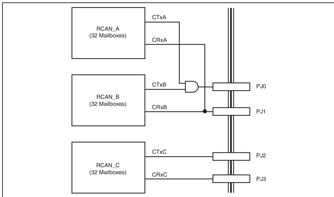
Figure 18.30 Connection Example when Using RCAN-TL1 as 2-Channel Module (64 Mailboxes × 1 Channel and 32 Mailboxes × 1 Channel)
