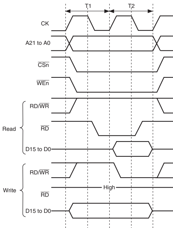
Figure 10.13 Basic Access Timing for SRAM with Byte Selection (BAS = 1)
