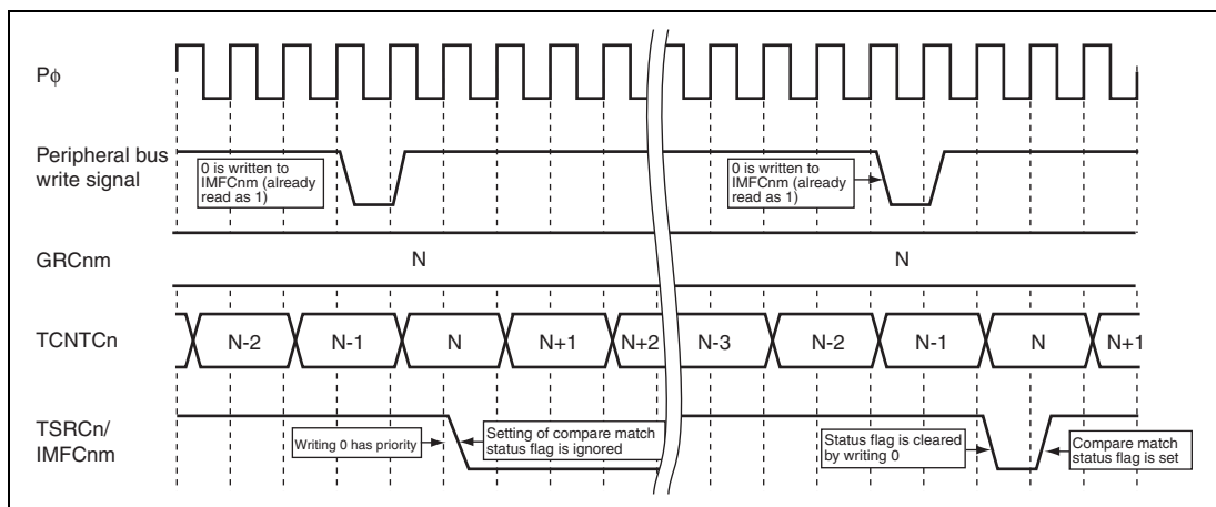
Figure 13.61 Conflict between Setting and Clearing of Compare Match Status Flag
