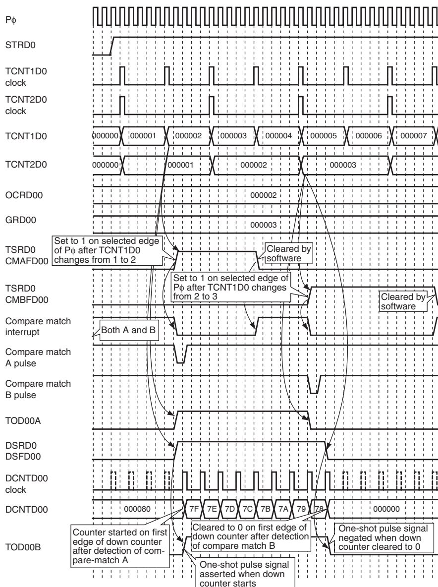
Figure 13.28 Operation Example of One-Shot Pulse Output (1) (Counting Started on Compare Match A and Stopped on Compare Match B)
