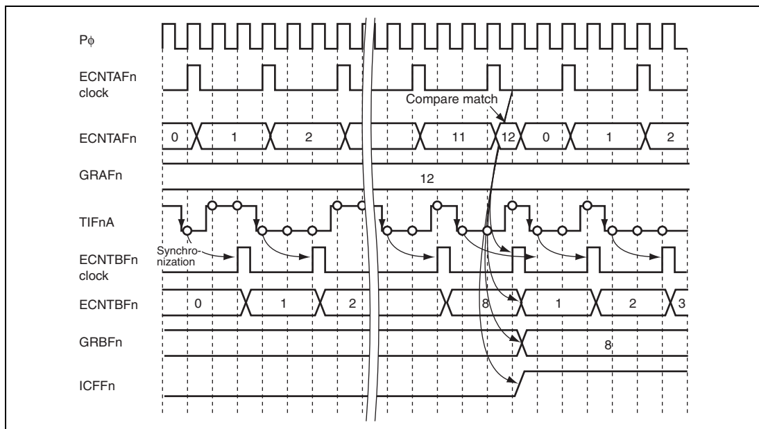
Figure 13.37 Operation Example of Edge Count in a Given Time (Compare Match and Event Occur Simultaneously)
