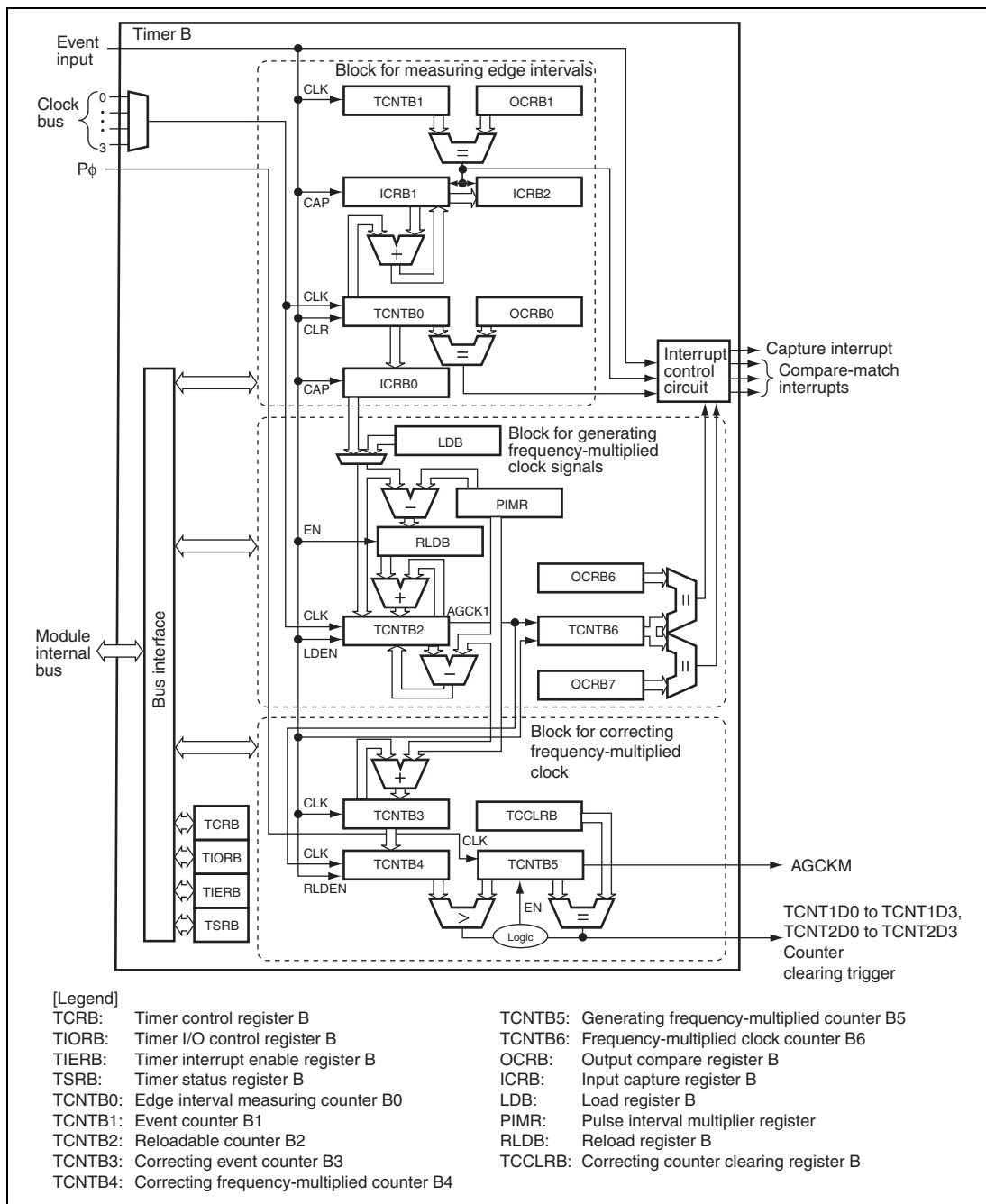
Figure 13.12 Block Diagram of Timer B
