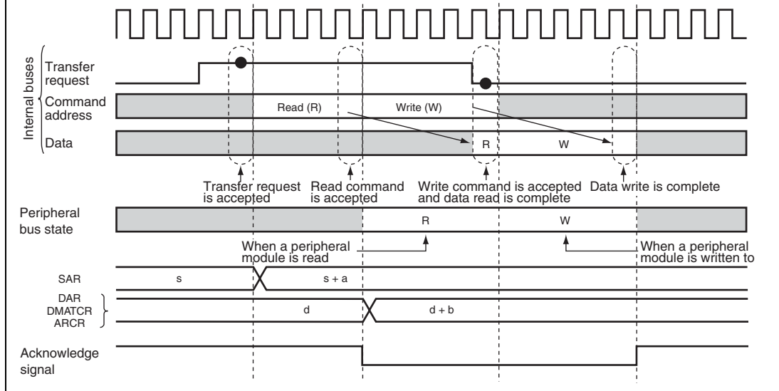
Figure 11.12 Change Timing of Register Contents and Acknowledge Signal
