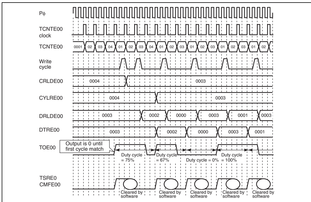
Figure 13.32 Operation of PWM (1)
