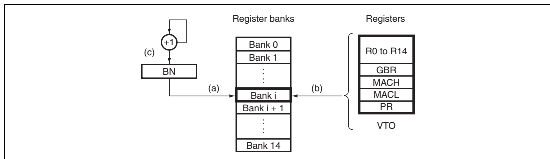
Figure 8.11 Bank Saving Operation
