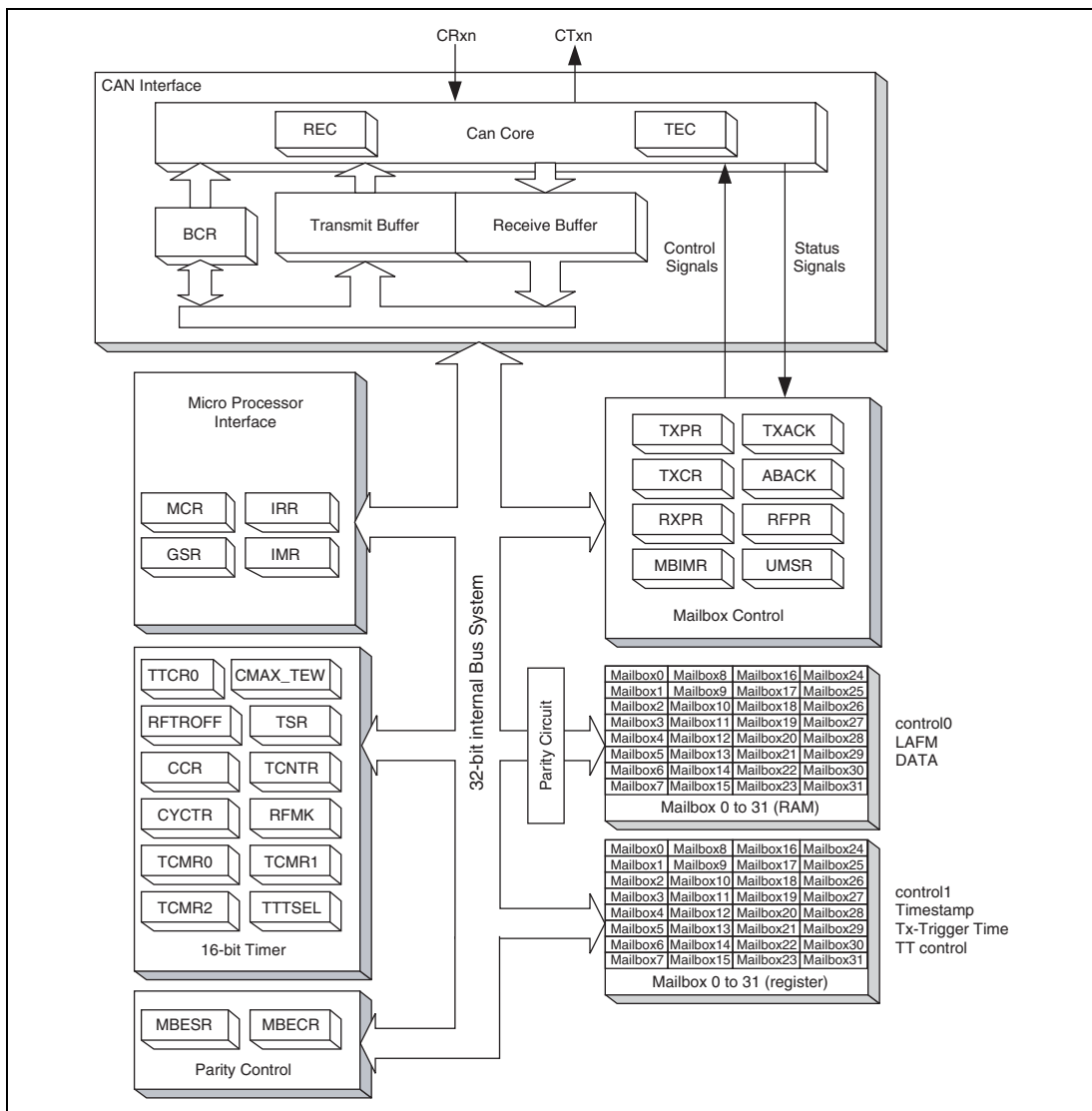
Figure 18.1 RCAN-TL1 architecture
