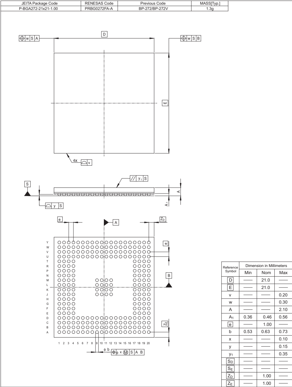
Figure C.1 Package Dimensions
