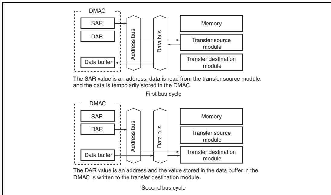
Figure 11.5 Data Flow of Dual Address Mode
