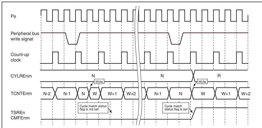
Figure 13.60 Conflict between TCNTEnm Write and Counter Clearing by Cycle Match
