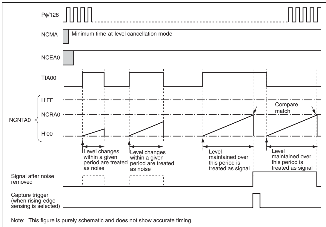
Figure 13.2 Operation of Noise Canceller in Minimum-Time-at Level Cancellation Mode
