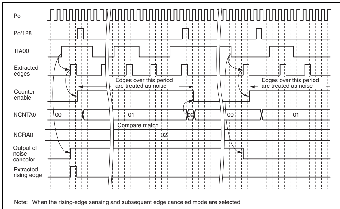
Figure 13.6 Example of Noise Cancellation in Premature-Transition Cancellation
