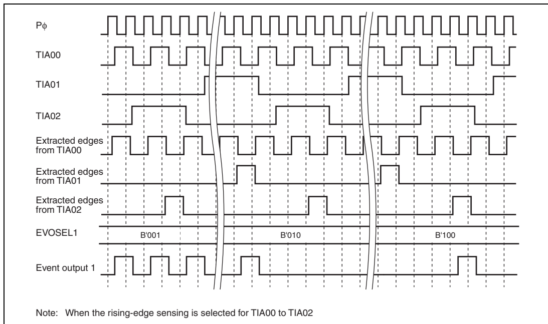
Figure 13.11 Example of Event Output
