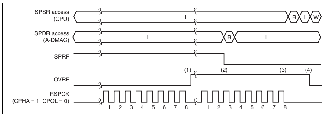
Figure 17.15 SPRF and OVRF Bit Operation Example
