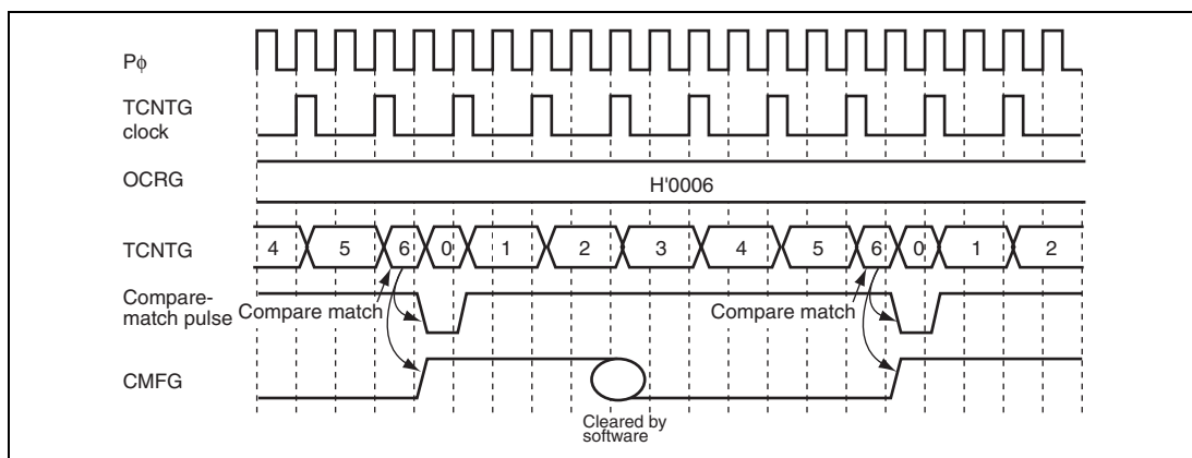
Figure 13.46 Operation Example of Counter and Compare Match
