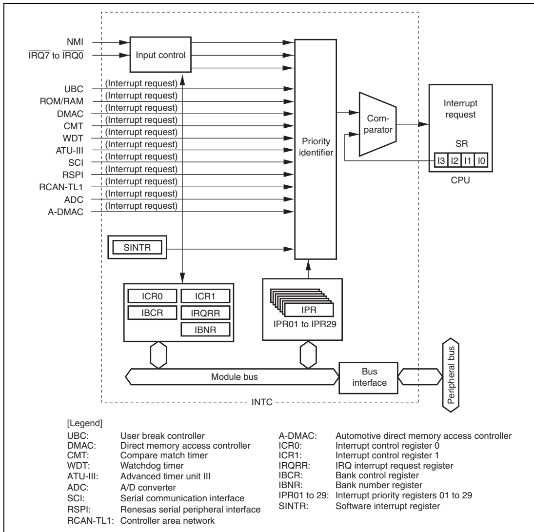
Figure 8.1 Block Diagram of INTC
