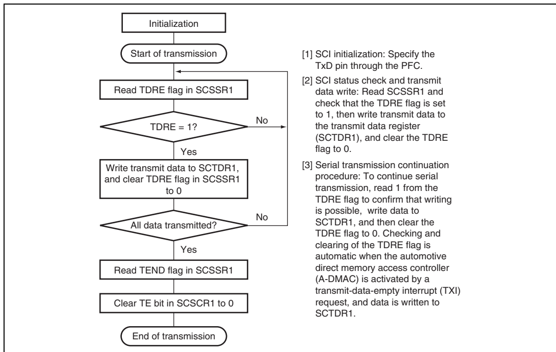
Figure 16.10 Sample Flowchart for Transmitting Serial Data
