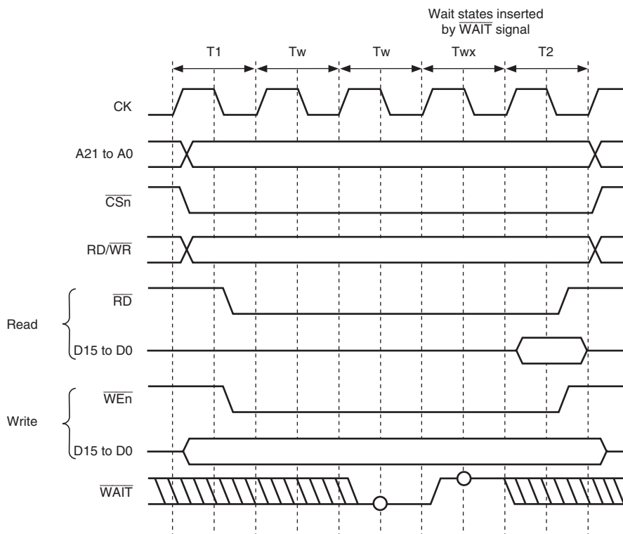
Figure 10.10 Wait Cycle Timing for External Space Access (Wait Cycle Insertion Using \overline{\text{WAIT}} Signal)
