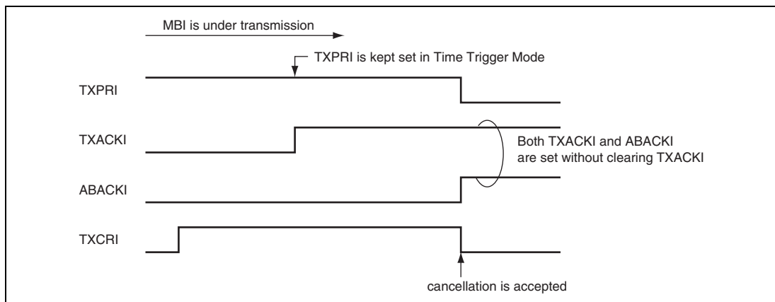
Figure 18.7 TXACK and ABACK in Time Trigger Transmission
