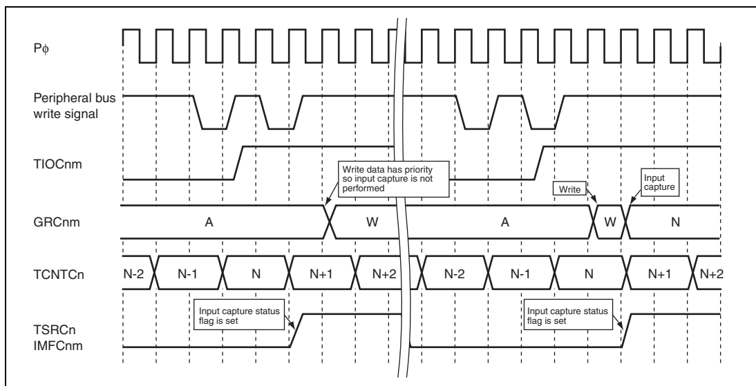
Figure 13.52 Conflict between Writing to GRCnm and Input Capture
