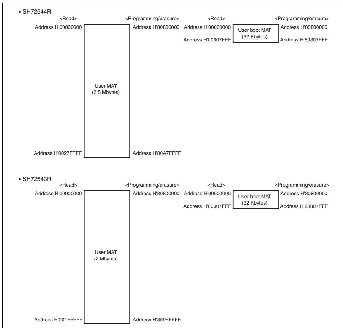
Figure 25.1 Memory MAT Configuration in ROM
