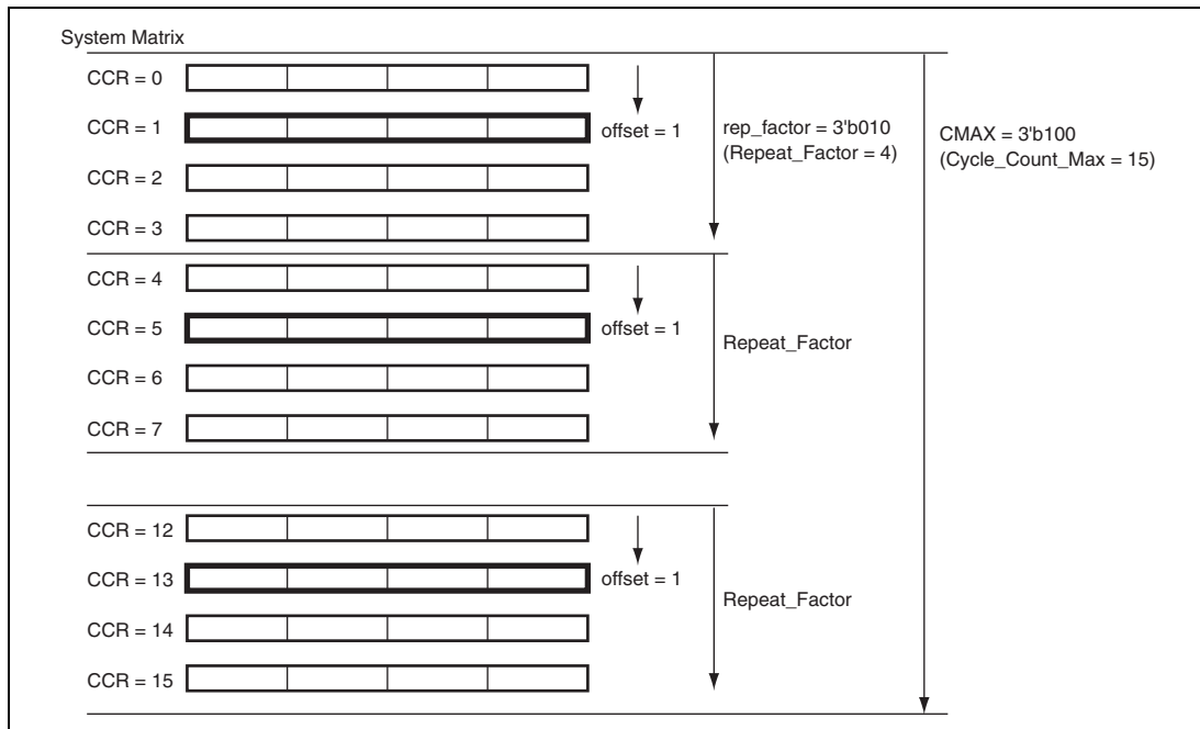
Figure 18.8 System Matrix
