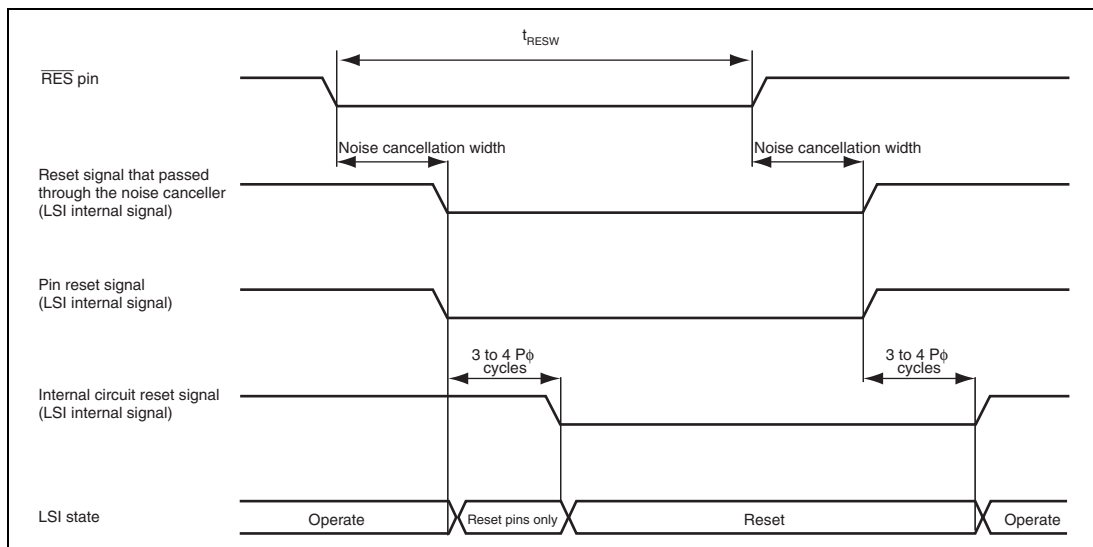
Figure 6.2 Reset Sequence
