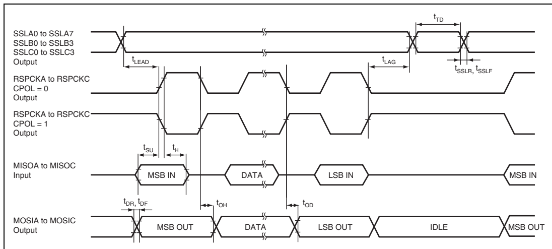
Figure 32.22 SPI Timing (Master, CPHA = 0)
