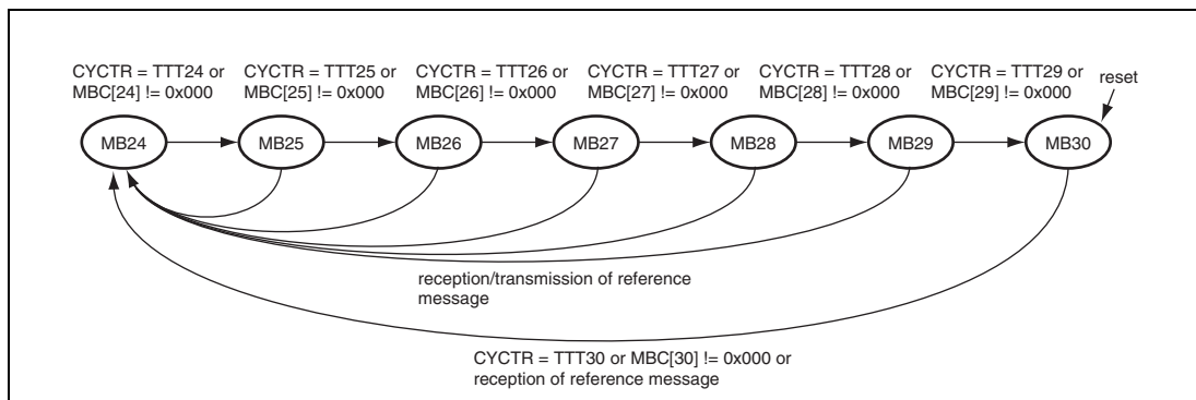
Figure 18.13 TTTSEL modification algorithm
