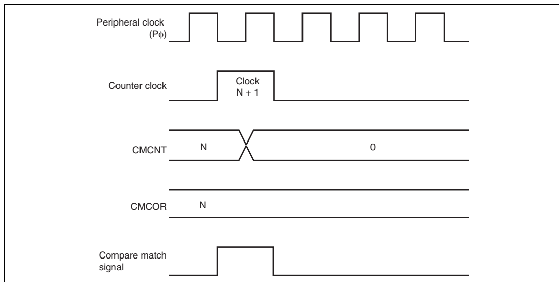
Figure 15.4 Timing of CMF Setting
