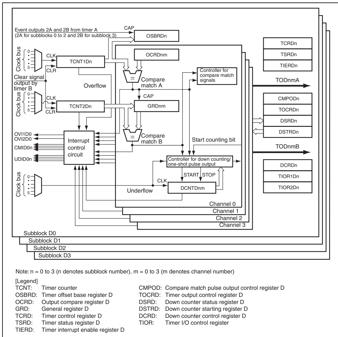
Figure 13.27 Block Diagram of Timer D
