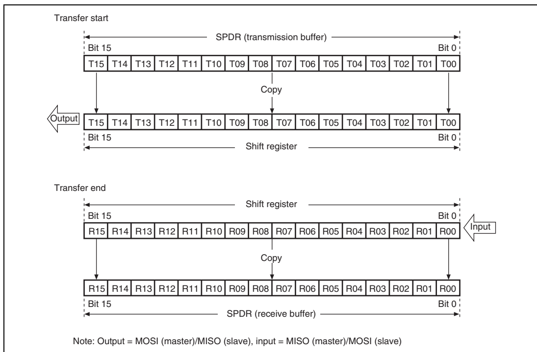
Figure 17.10 MSB First Transfer (16-Bit Data)
