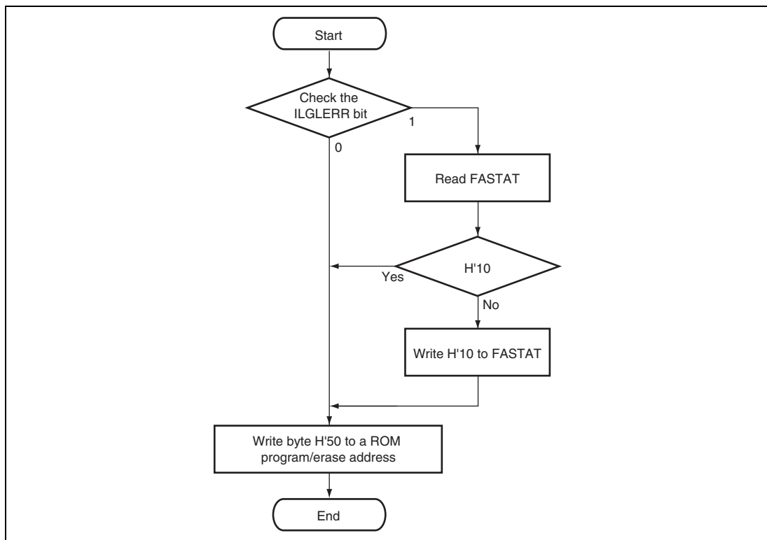
Figure 25.22 Procedure for Clearing Status Register 0
