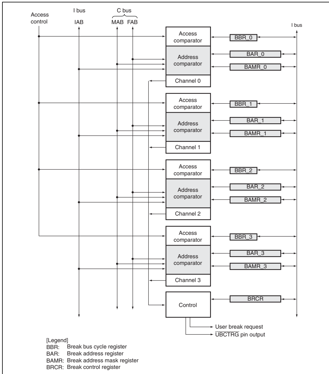
Figure 9.1 Block Diagram of UBC
