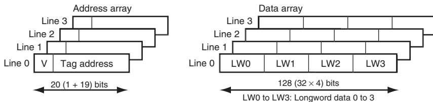
Figure 27.1 Cache Configuration
