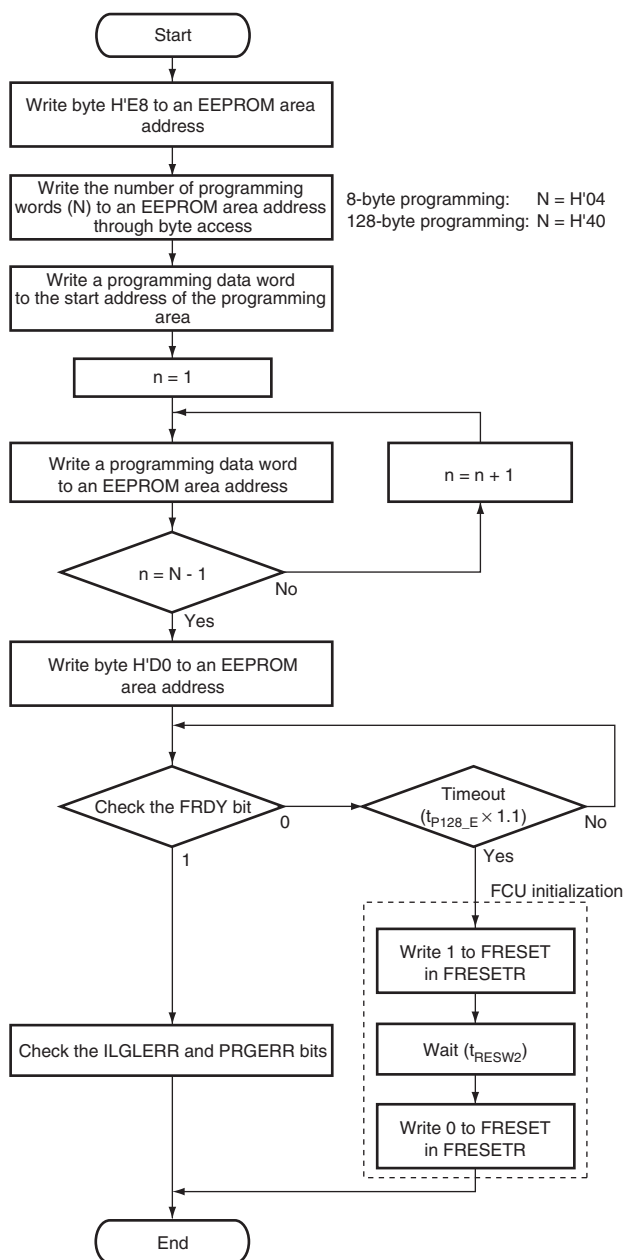
Figure 26.6 Procedure for EEPROM Programming
