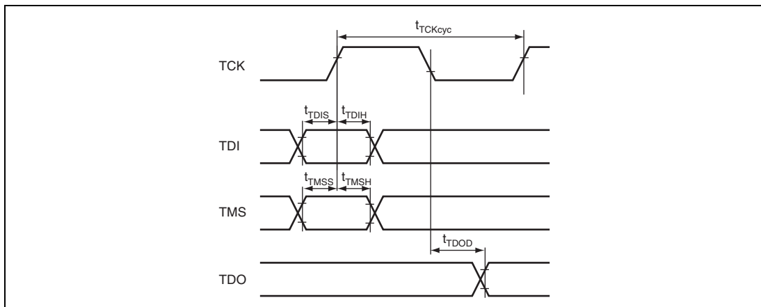
Figure 32.32 JTAG Interface Input/Output
