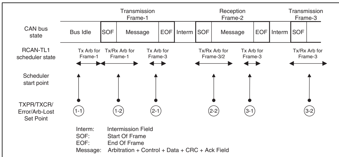
Figure 18.17 Internal Arbitration for transmission
