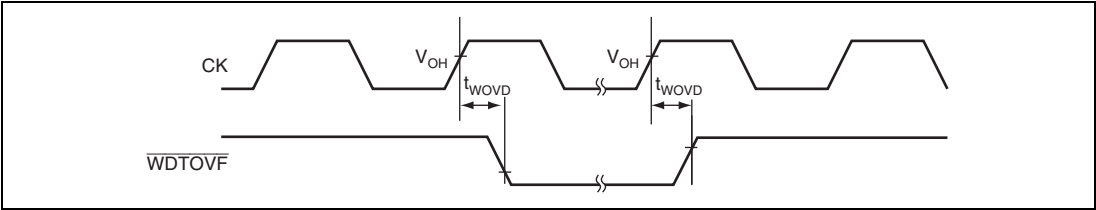
Figure 32.17 Watchdog Timer Timing
