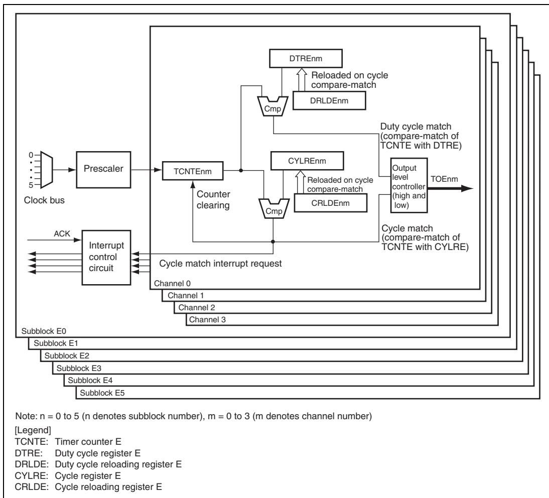
Figure 13.31 Block Diagram of Timer E
