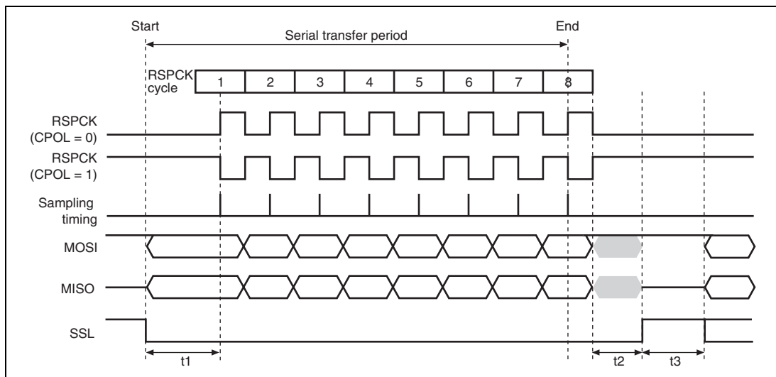
Figure 17.8 RSPI Transfer Format (CPHA = 0)
