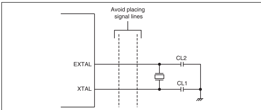
Figure 4.5 Note on Board Design
