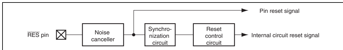
Figure 6.1 Reset Circuit
