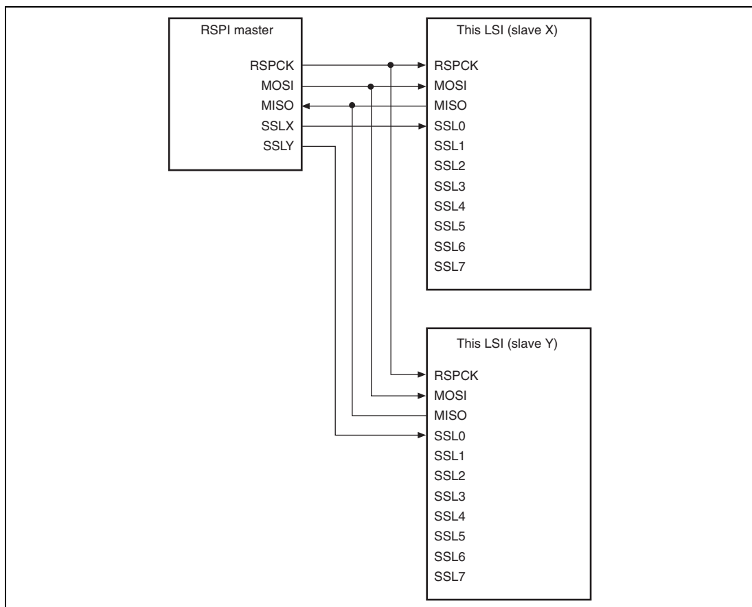
Figure 17.6 Single-Master/Multi-Slave Configuration Example (This LSI = Slave)
