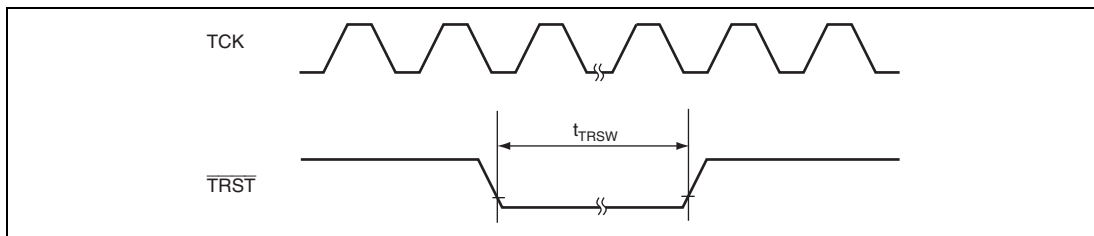
Figure 32.31 JTAG Interface \overline{\text{TRST}} Timing
