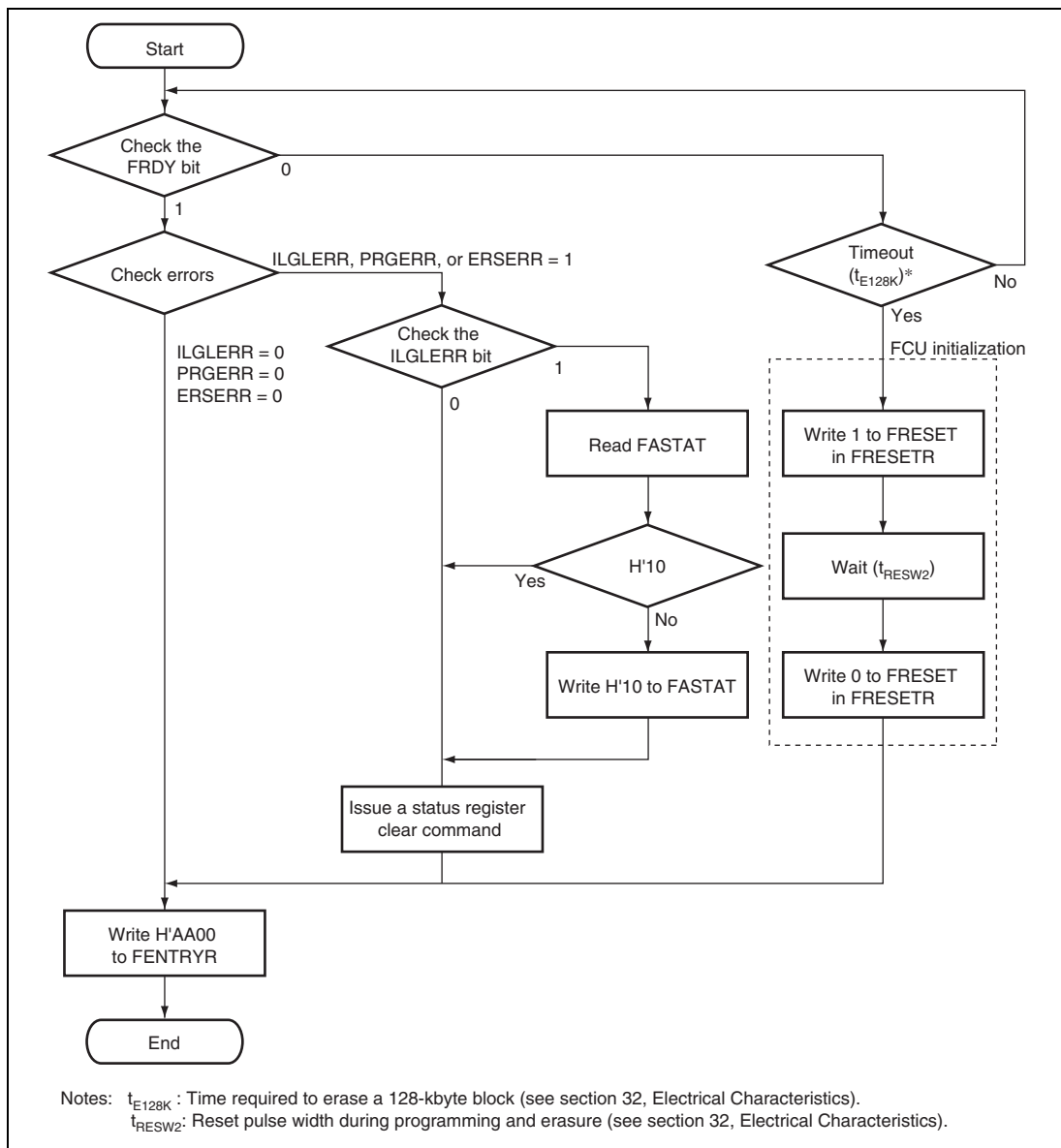
Figure 25.16 Procedure for Transition to ROM Read Mode
