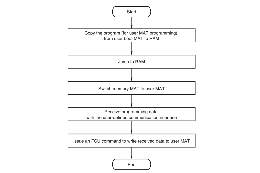
Figure 25.31 Example of User MAT Programming
