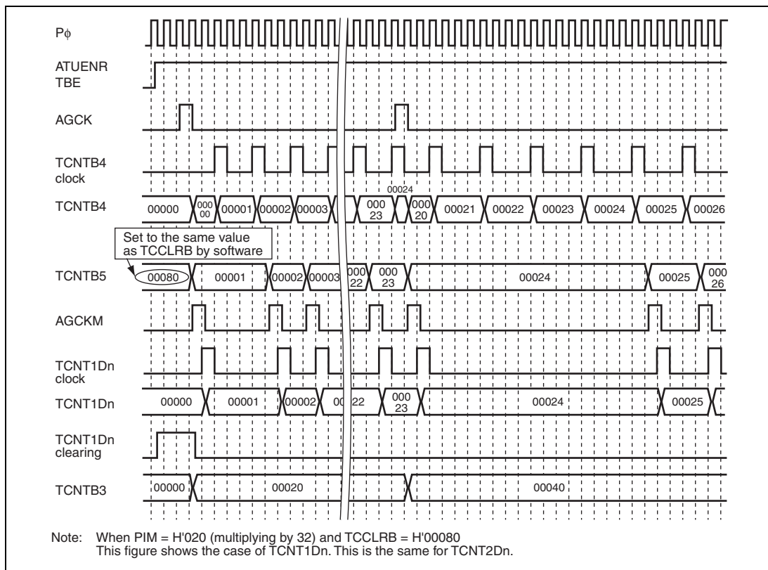
Figure 13.20 TCNTB5 Operation (at Start-Up)
