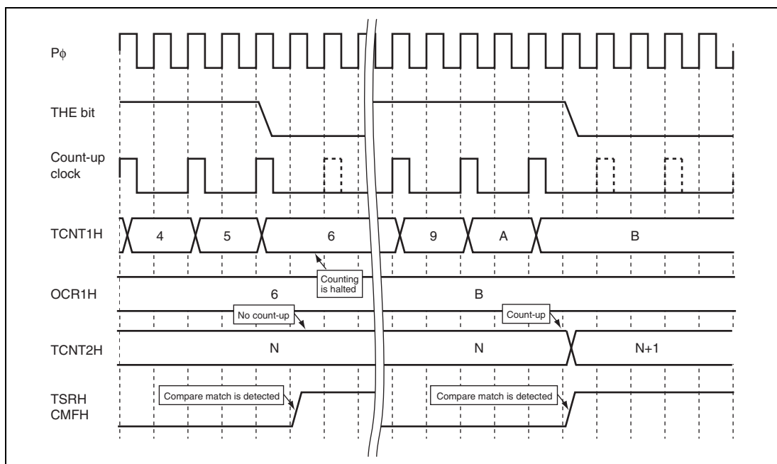
Figure 13.64 Conflict between Compare Match Detection and Disabling of Counter
