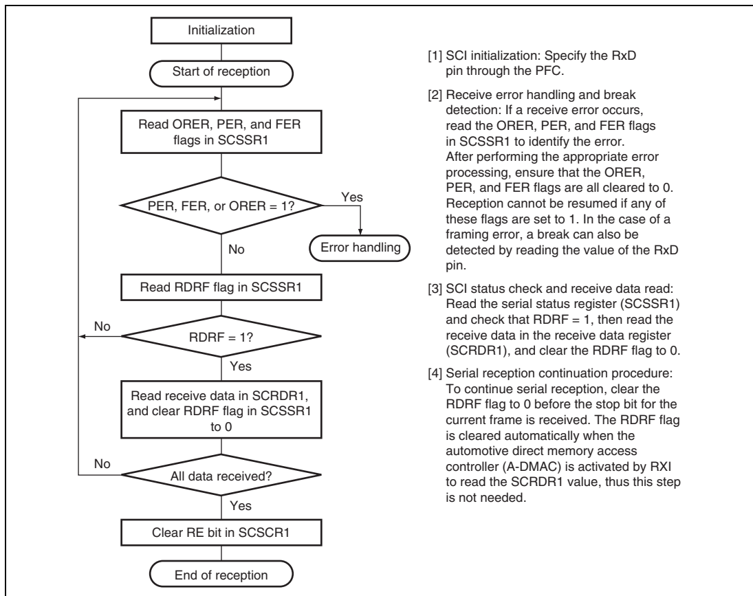
Figure 16.6 Sample Flowchart for Receiving Serial Data (1)
