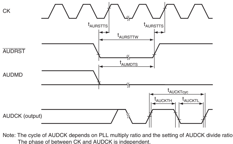
Figure 32.33 Trace Mode Reset Timing
