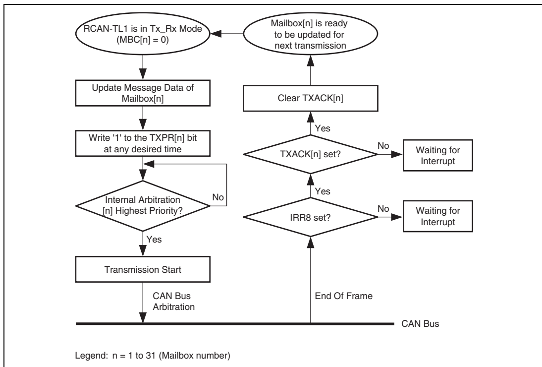
Figure 18.16 Transmission request
