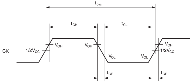
Figure 32.5 Peripheral Clock Timing
