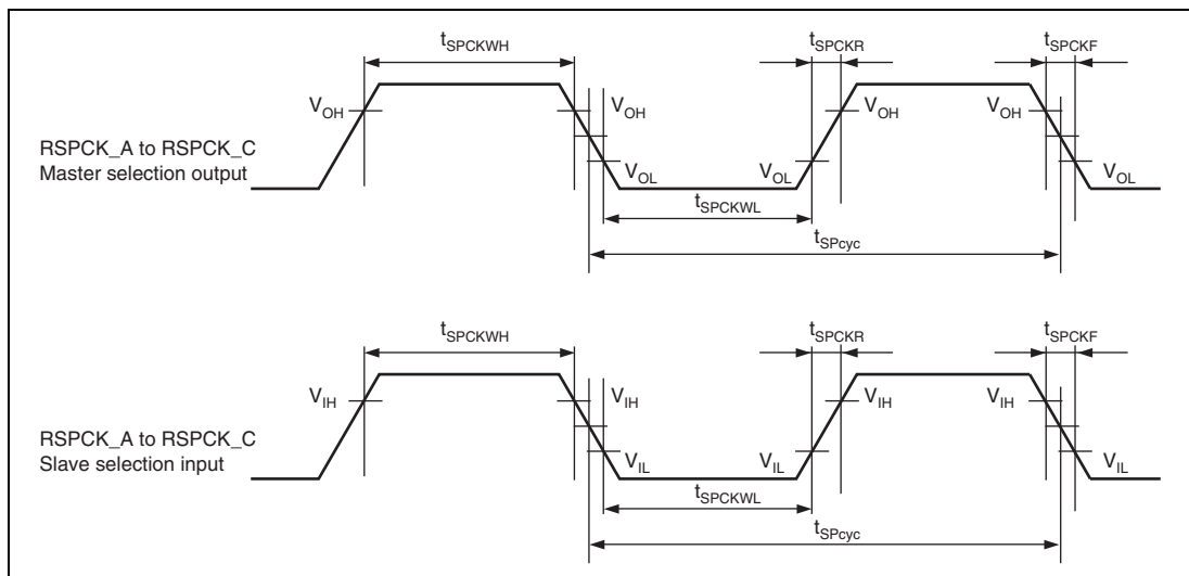
Figure 32.21 SPI Clock Timing
