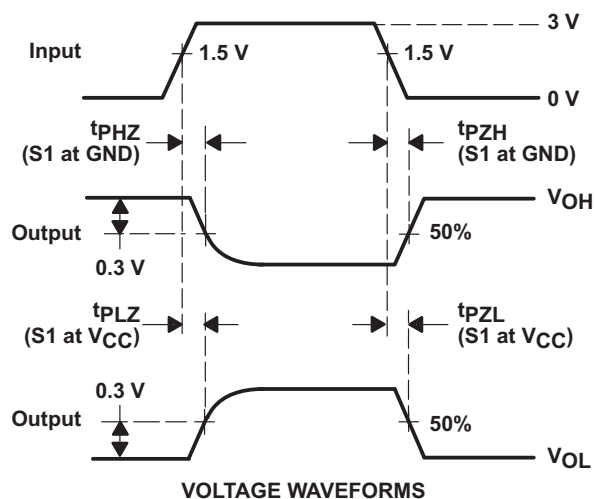
VOLTAGE WAVEFORMS
