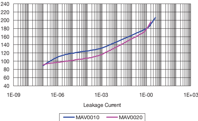
Voltage/Current Characteristics
