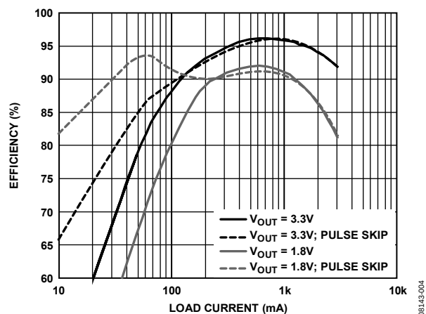
Figure 4. Channel 1 Efficiency vs. Load, V_{IN} = 5V and f_{SW} = 300\text{ kHz} ; V_{OUT} = 3.3V , Inductor Cooper Bussmann DR1050-8R2-R, 8.2\mu\text{H} , 15\text{ m}\Omega ; V_{OUT} = 1.8V , Inductor TOKO FDV0620-4R7M, 4.7\mu\text{H} , 53\text{ m}\Omega
