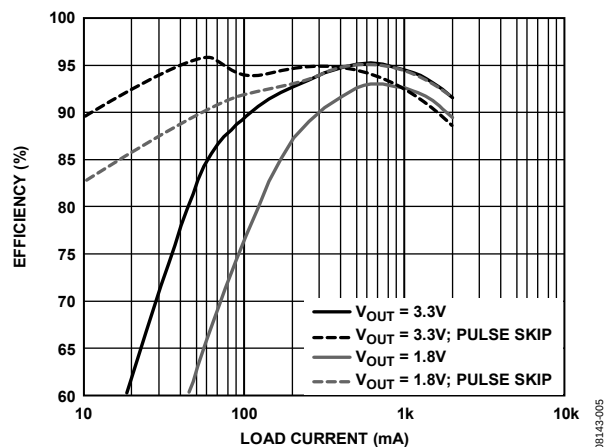
Figure 5. Channel 2 Efficiency vs. Load, V_{IN} = 5V and f_{SW} = 600\text{ kHz} ; V_{OUT} = 3.3V , Inductor TOKO FDV0620-4R7M, 4.7\mu\text{H} , 53\text{ m}\Omega ; V_{OUT} = 1.8V , Inductor TOKO FDV0620-2R2M, 2.2\mu\text{H} , 30\text{ m}\Omega
