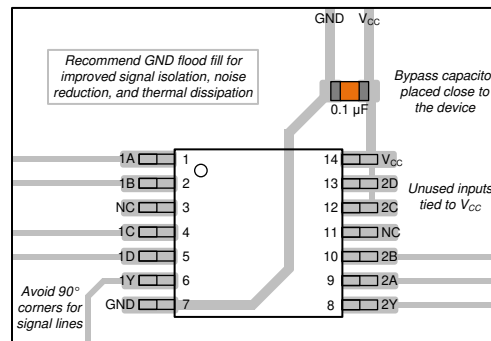
Figure 11. Example layout for the SN74HCS20
