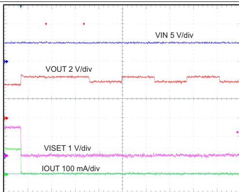
图 7. DPM-Adaptor Current Limits
