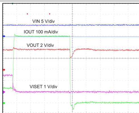
图 8. Hot Plug Source with No Battery - Battery Detection
