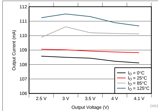
图 17. Current Regulation Over Temperature
