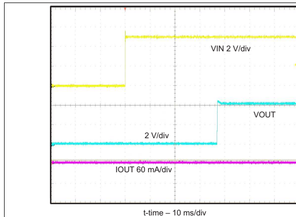
图 3. Power Up Timing
