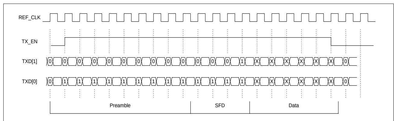
Parameter Symbol Min Typ Max Unit REF_CLK cycle time REF_CLK – 20 – ns TXEN, TX_ER, TXD[1:0] setup time to REF_CLK rising TXEN_SETUP 4 – – ns TXEN, TX_ER, TXD[1:0] hold time from REF_CLK rising TXEN_HOLD 2 – – ns TD± after TXEN assert TXEN_TDATA – 89 – ns TXD to TD± steady state delay TXD_TDATA – 95 – ns Note: TXD[1:0] shall provide valid data for each REF_CLK period while TX_EN is asserted. As the REF_CLK frequency is 10 times the data rate in 10MB/s mode, the value on TXD[1:0] shall be valid such that TXD[1:0] can be sampled every 10th cycle, regardless of the starting cycle within the group and yield the correct frame data.
