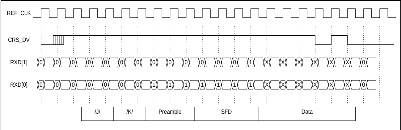
Figure 7: RMII Receive Packet Timing
