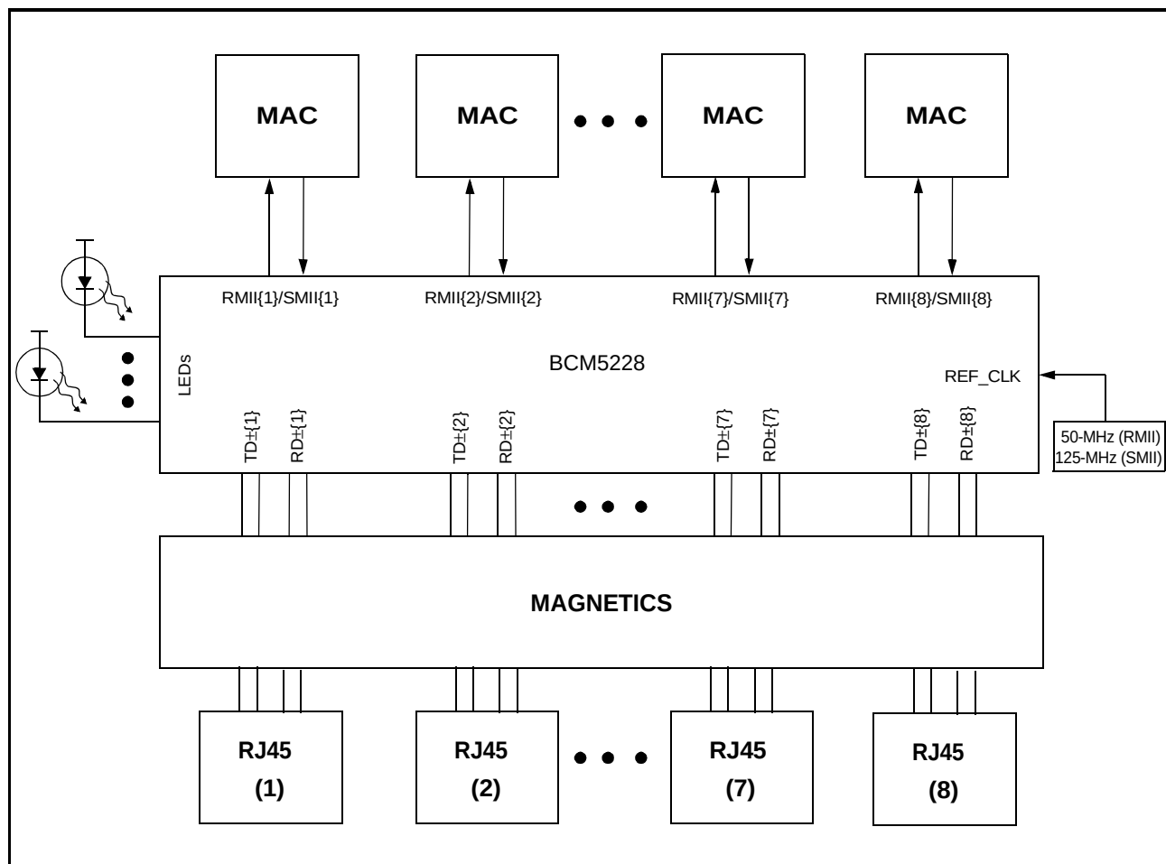
Figure 16: Switch Application
