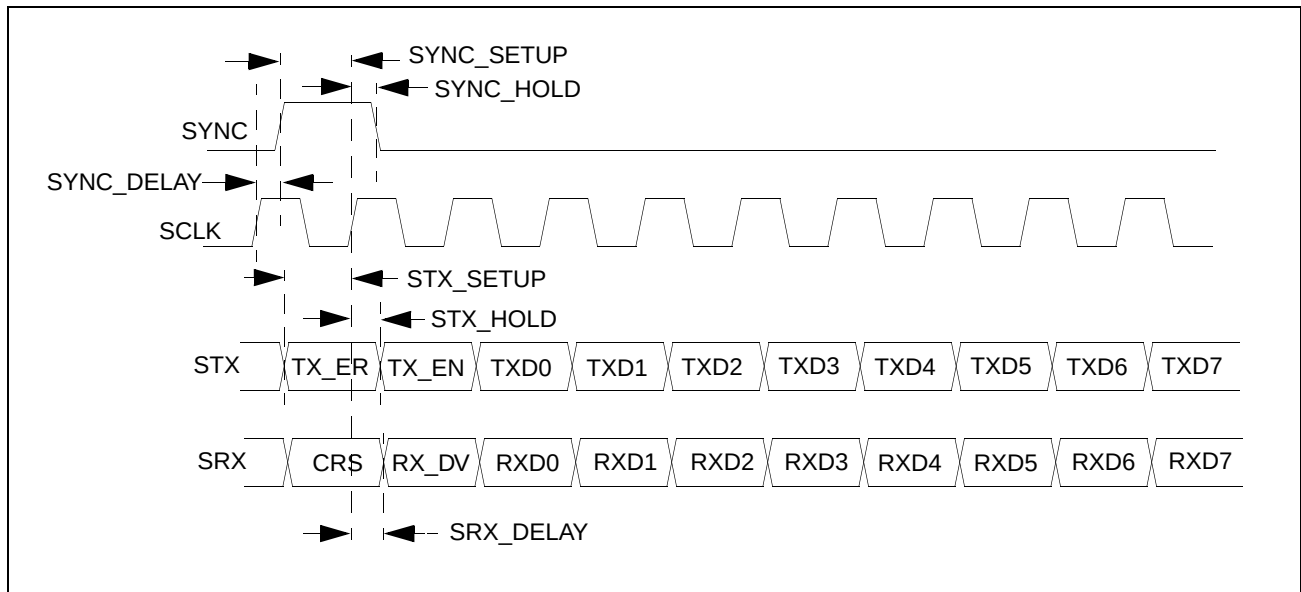
Figure 9: SMII/S3MII Timing
