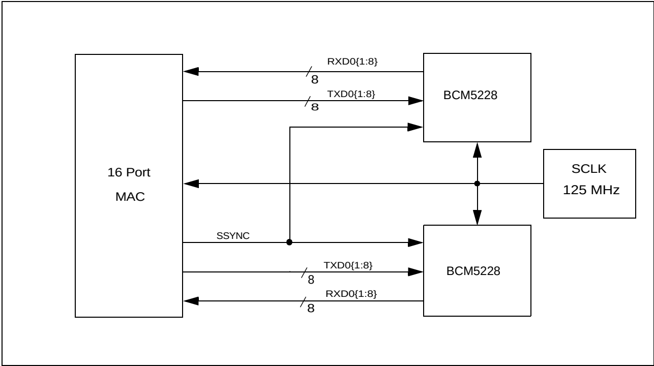
Figure 14: SMI Application
