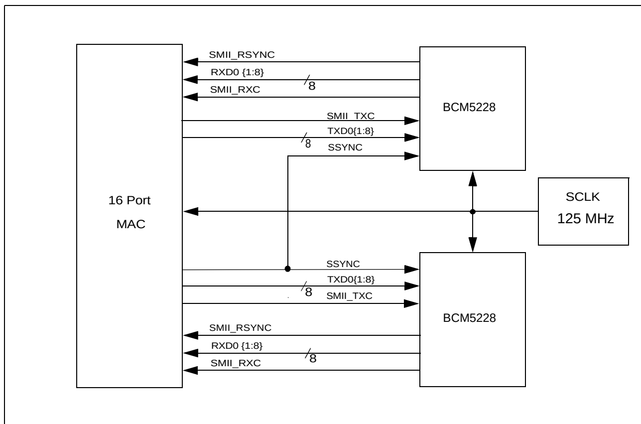
Figure 15: SMI Application using Source Synchronous Signals
