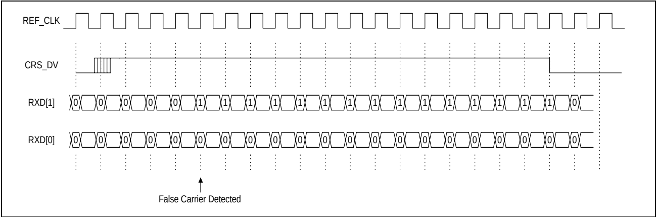
Figure 8: RMII Receive Packet with False Carrier
