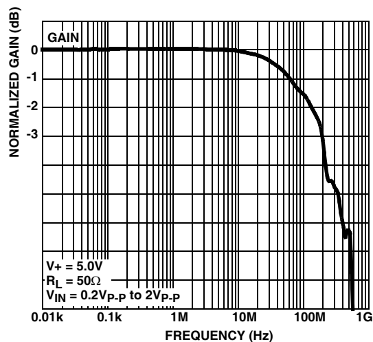
FIGURE 16. FREQUENCY RESPONSE
