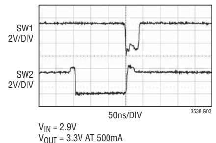
Switch Pins Before Entering Boost Mode
