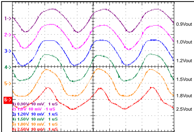
Figure 27: Output Voltage Ripple at 3.3V input voltage and rated load current (10 mV/div). Load capacitance: 10 \mu F ceramic capacitor and 15 \mu F tantalum capacitor. Bandwidth: 20 MHz. See Figure 26.
