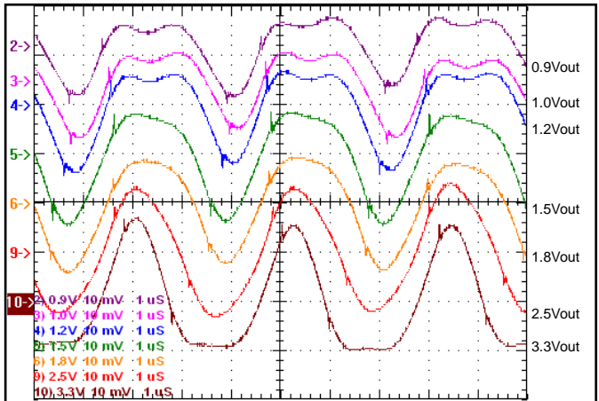
Figure 28: Output Voltage Ripple at 5.0V input voltage and rated load current (10 mV/div). Load capacitance: 10 \mu F ceramic capacitor and 15 \mu F tantalum capacitor. Bandwidth: 20 MHz. See Figure 26.
