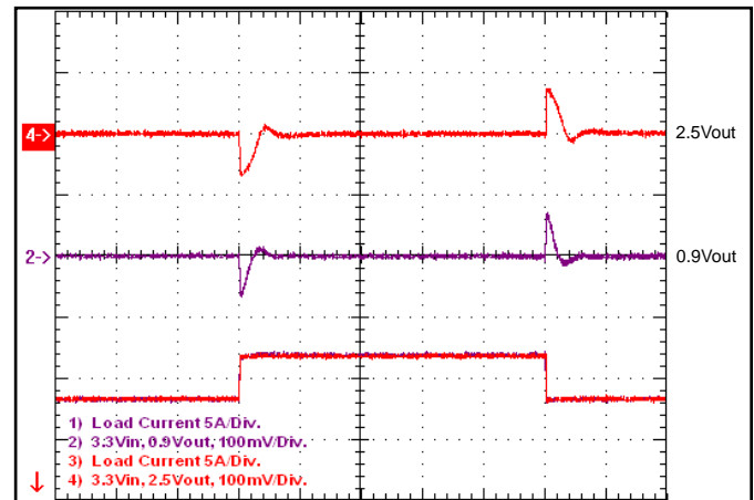
Figure 16: Output voltage response at 3.3Vin to step-change in load current (40% of Iout max; di/dt=3A/μs). Load cap: 470μF, 25mΩ ESR tantalum and 10μF ceramic. Top: Vout (100mV/div), Bottom: Iout (5A/div).
