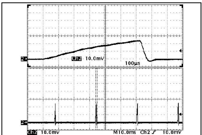
Figure 30: Load current (10A/div) as a function of time when a 5.0V in , 0.9V o unit attempts to turn on into a 10 m \Omega short circuit. Top trace (100 \mu s/div) is an expansion of the on-time portion of the bottom trace.
