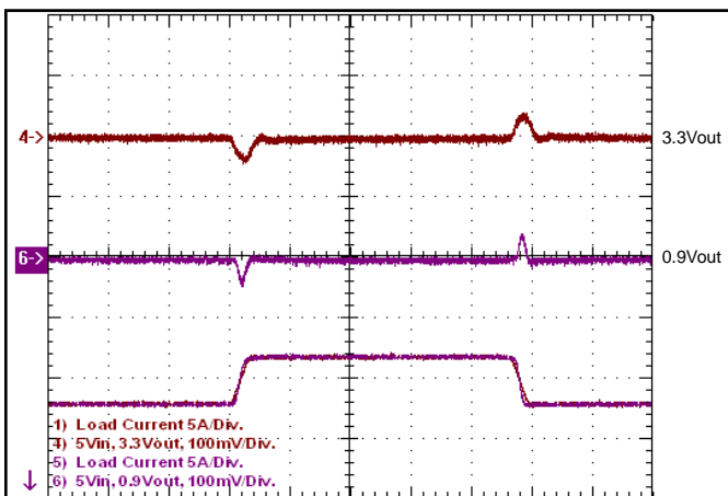
Figure 17: Output voltage response at 5.0Vin to step-change in load current (40% of Iout max; di/dt=0.1A/μs). Load cap: 15μF, 100mΩ ESR tantalum and 10μF ceramic. Top: Vout (100mV/div), Bottom: Iout (5A/div).
