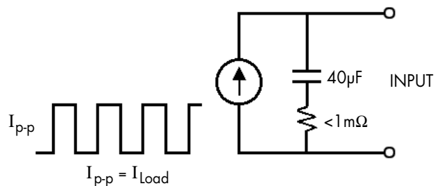
Figure B: Equivalent model for input ripple
