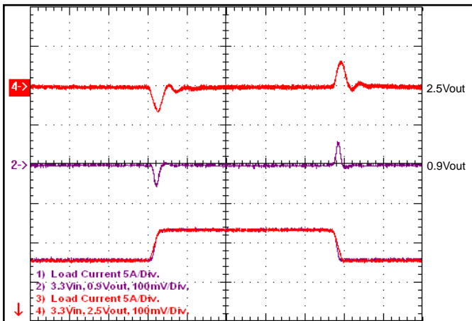
Figure 15: Output voltage response at 3.3Vin to step-change in load current (40% of Iout max; di/dt=0.1A/μs). Load cap: 15μF, 100mΩ ESR tantalum and 10μF ceramic. Top: Vout (100mV/div), Bottom: Iout (5A/div).
