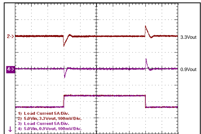
Figure 18: Output voltage response at 5.0Vin to step-change in load current (40% of Iout max; di/dt=3A/μs). Load cap: 470μF, 25mΩ ESR tantalum and 10μF ceramic. Top: Vout (100mV/div), Bottom: Iout (5A/div).
