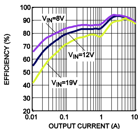
Figure 26 — Efficiency Curve
