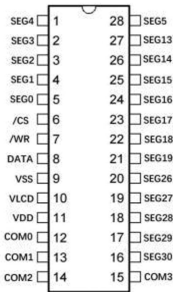
1621B 28SOP-A/SSOP-A
