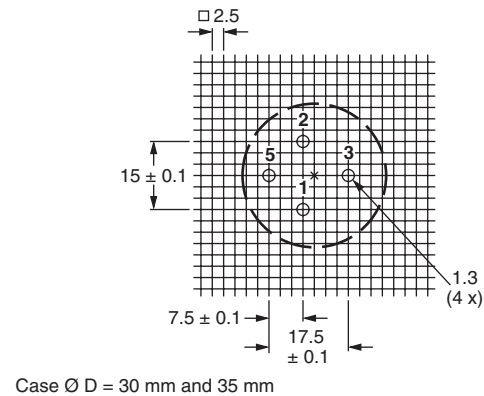
Fig.4 Mounting hole pattern viewed from the component side
