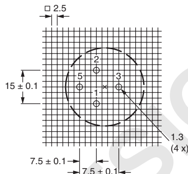
Fig.6 Mounting hole pattern viewed from the component side
