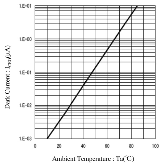
Ambient Temperature vs. Dark Current Condition : V_{CE0} = 10V
