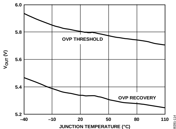
Figure 18. Typical Overvoltage Protection (OVP) Threshold
