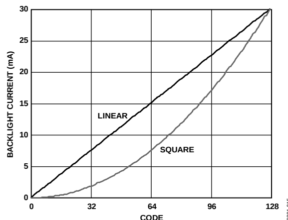
Figure 29. Backlight Current vs. Input Code
