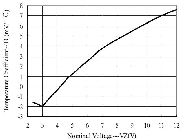
Typical Temperature Coefficient
