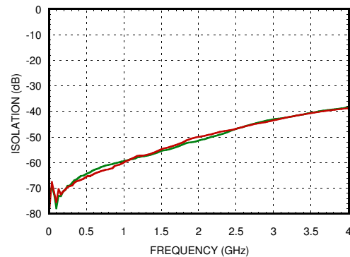
Isolation Between Ports RF1 and RF2
