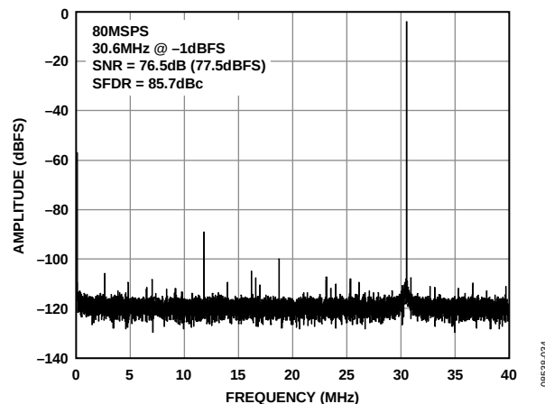
图9. AD9269-80单音FFT( f_{IN} = 30.6\text{ MHz} )
