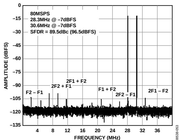
图8. AD9269-80双音FFT( f_{IN1} = 28.3\text{ MHz} 、 f_{IN2} = 30.6\text{ MHz} )
