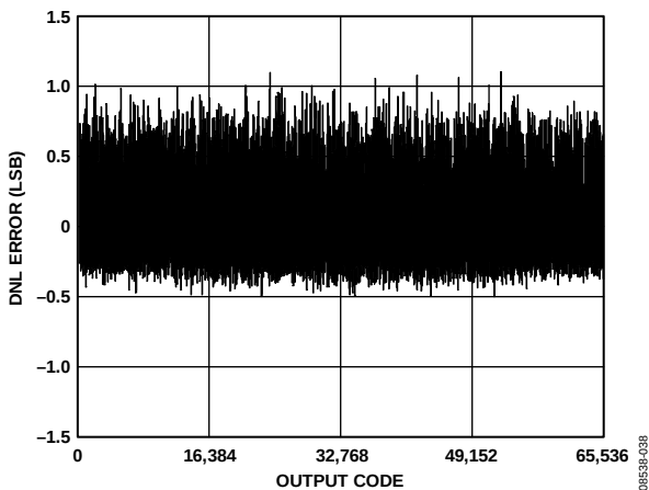
图14. DNL误差 ( f_{IN} = 9.7\text{ MHz} )
