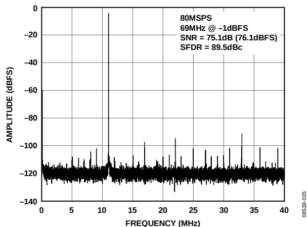
图7. AD9269-80单音FFT( f_{IN} = 69\text{ MHz} )
