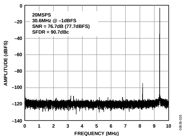
图27. AD9269-20单音FFT( f_{IN} = 30.6\text{ MHz} )
