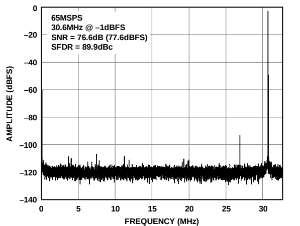
图20. AD9269-65单音FFT( f_{IN} = 30.6\text{ MHz} )
