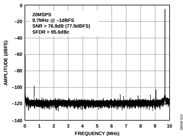
图26. AD9269-20单音FFT( f_{IN} = 9.7\text{ MHz} )
