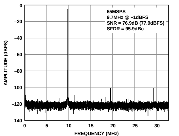
图18. AD9269-65单音FFT( f_{IN} = 9.7\text{ MHz} )
