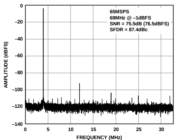
图19. AD9269-65单音FFT( f_{IN} = 69\text{ MHz} )
