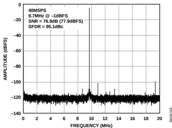
图23. AD9269-40单音FFT( f_{IN} = 9.7 MHz)
