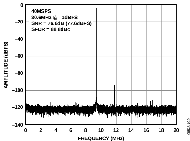
图24. AD9269-40单音FFT( f_{IN} = 30.6 MHz)
