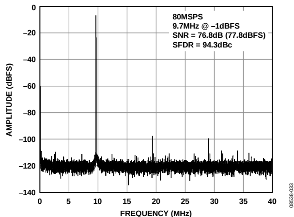
图6. AD9269-80单音FFT( f_{IN} = 9.7\text{ MHz} )
