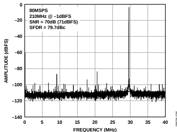
图10. AD9269-80单音FFT ( f_{IN} = 210\text{ MHz} )
