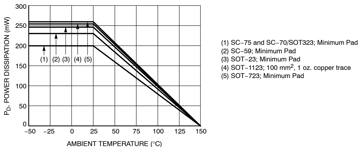
Figure 1. Derating Curve
