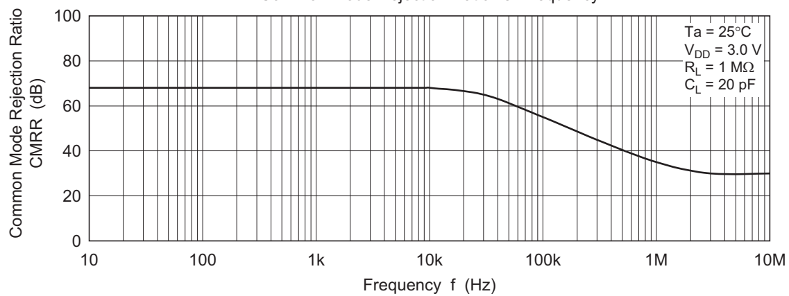
Figure 3-13. HA1630S06 Common Mode Rejection Ratio vs. Frequency
