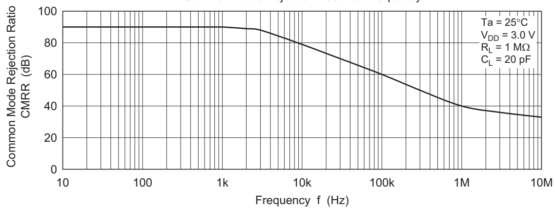
Figure 2-13. HA1630S05 Common Mode Rejection Ratio vs. Frequency
