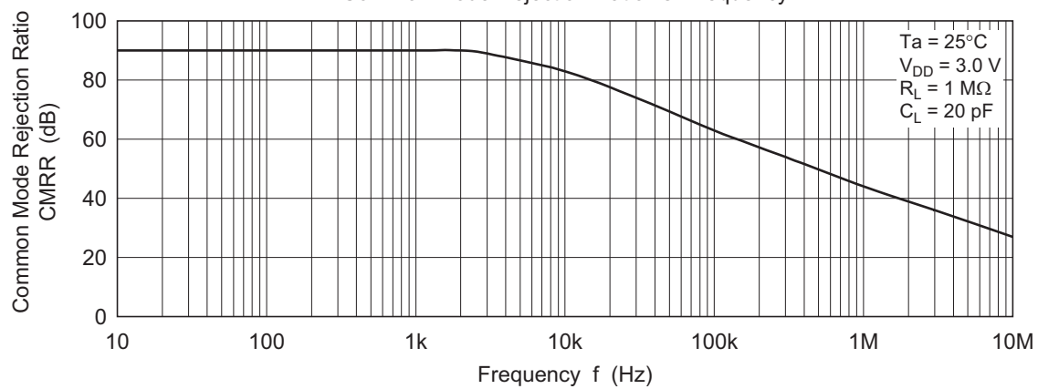
Figure 1-13. HA1630S04 Common Mode Rejection Ratio vs. Frequency
