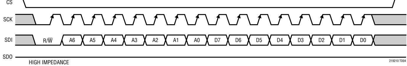
SPI Port Timing (Write Mode)
