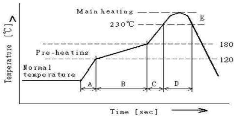
Temperature Profile
