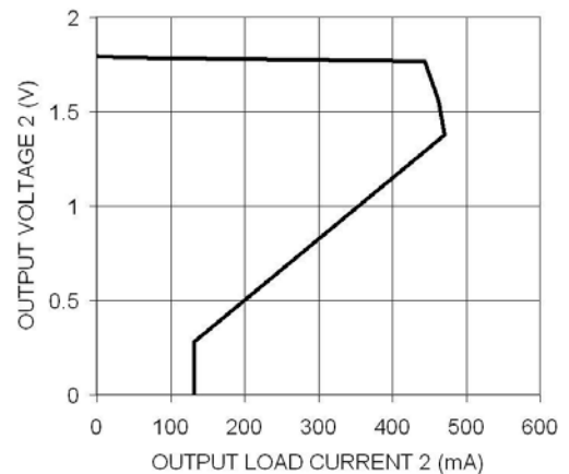
Figure 14. Output Voltage 2 vs. Load Current 2
