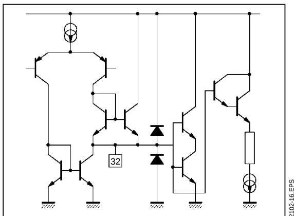
Figure 14 : Pin 32 (CKP)
