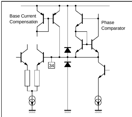
Figure 19 : Pin 34 (CLPF)
