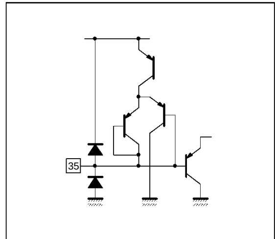
Figure 20 : Pin 35 (FBL)
