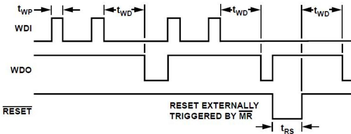
Figure 16. Watchdog Timing
