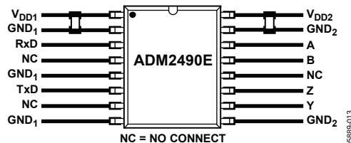
Figure 24. Recommended Printed Circuit Board Layout
