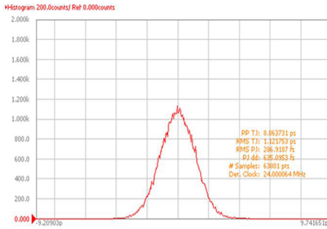
Frequency - 24.000MHz
