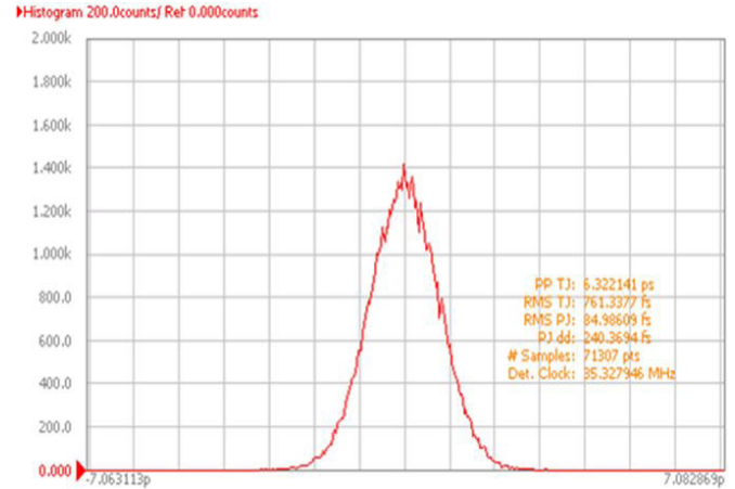
Frequency - 35.328MHz
