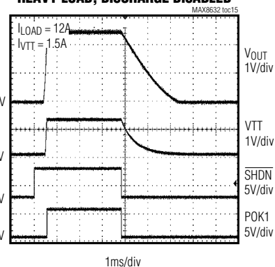
STARTUP AND SHUTDOWN INTO HEAVY LOAD, DISCHARGE DISABLED
