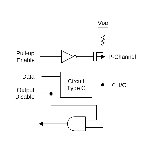
Figure 1-5. Pin Circuit Type D-2 (P3)
