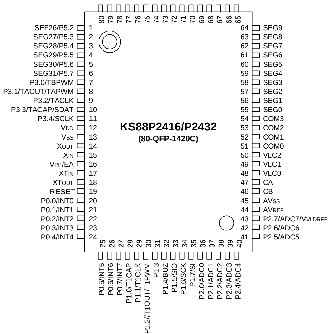
Figure 21-1. KS88P2416/P2432 Pin Assignments (80-QFP Package)
