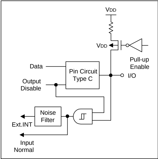
Figure 1-6. Pin Circuit Type D-4 (P0)
