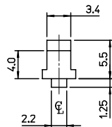
DETAIL "B" SCALE 2:1
